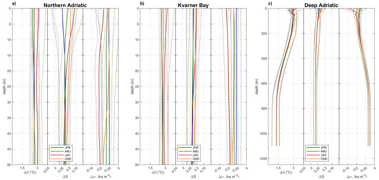
Figure 20. Variations (SCE-CTR) between median seasonal (again, with seasons defined as in Pranić et al. 2021 to enable the comparison with Figure 12) potential temperature ( \theta ), salinity ( S ), and potential density anomaly ( \sigma_{\theta} ) profiles in the Northern Adriatic (a), Kvarner Bay (b), and Deep Adriatic (c). Dashed lines bracket the ensemble spread.
