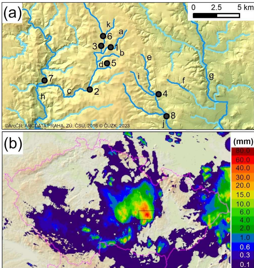
355 Figure 9: Flash flood on 15 July 2002: (a) the geographic situation in the affected area, (b) six-hour precipitation totals based on merged radar data across the Czech Republic (the "□" symbol marks the impacted area). Localities: 1 – Crhov, 2 – Hodonín, 3 – Křtěnov, 4 – Kunštát, 5 – Louka, 6 – Olešnice, 7 – Štěpánov nad Svatkou, 8 – Zbraslavce. Watercourses (dark blue): a – Crhovský potok, b – Dvorský potok, c – Hodonínka, d – Loucký potok, e – Petrůvka, f – Sebránek, g – Svitava, h – Svatka, i – Sychotínský potok, j – Úmoří, k – Veselský potok.
