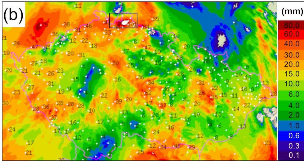
Figure 11: Flash flood on 7 August 2010: (a) the geographic situation in the affected area, (b) daily precipitation totals according to merged radar information over the Czech Republic (the "□" symbol marks the impacted area). Localities: 1 – Bílý Kostel nad Nisou, 2 – Bohatynia (Poland), 3 – Chrastava, 4 – Dětrichov, 5 – Frýdlant, 6 – Hejnice, 7 – Heřmanice, 8 – Hrádek nad Nisou, 9 – Raspenava, 10 – Višňová, Watercourses (dark blue): a – Jeřice, b – Lužická Nisa, c – Oleška, d – Rokytkva, e – Rynoltický potok, f – Smědá, g – Václavický potok, h – Vítkovský potok.
