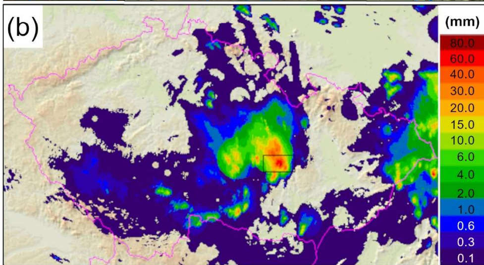
Figure 9: Flash flood on 15 July 2002: (a) the geographic situation in the affected area, (b) six-hour precipitation totals based on merged radar data across the Czech Republic (the "□" symbol marks the impacted area). Localities: 1 – Crhov, 2 – Hodonín, 3 – Křtěnov, 4 – Kunštát, 5 – Louka, 6 – Olešnice, 7 – Štěpánov nad Svatkou, 8 – Zbraslavce. Watercourses (dark blue): a – Crhovský potok, b – Dvorský potok, c – Hodonínka, d – Loucký potok, e – Petrůvka, f – Sebránek, g – Svitava, h – Svatka, i – Sychotínský potok, j – Úmoří, k – Veselský potok.
