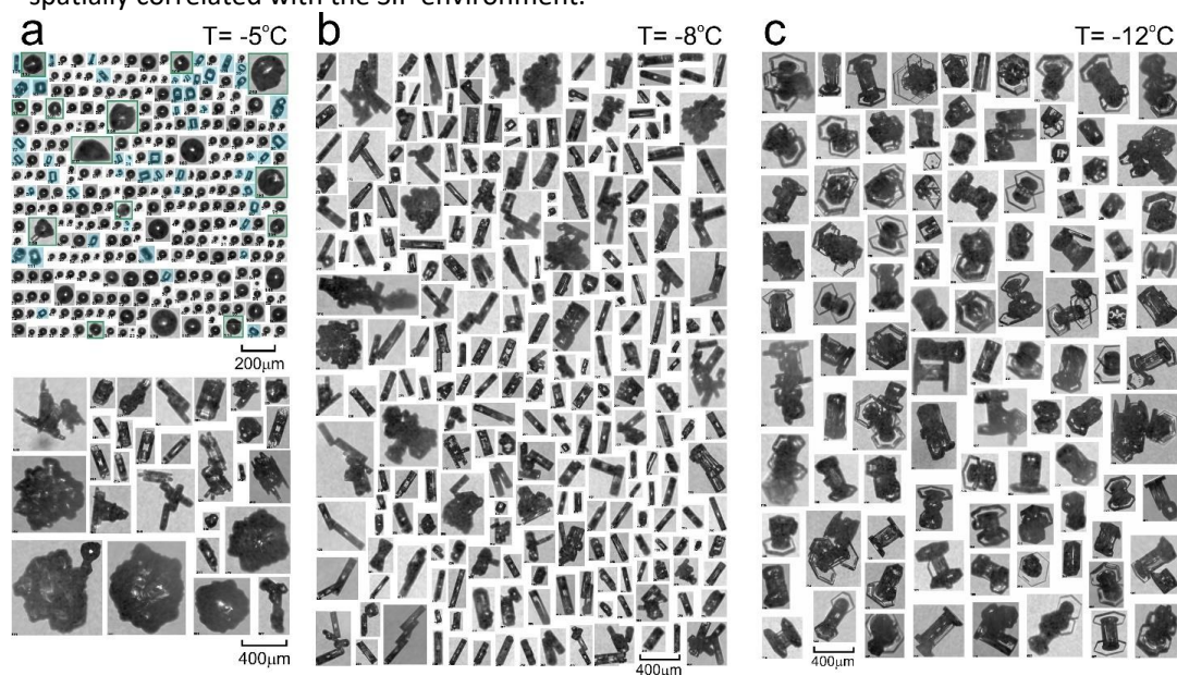
Figure 1. Images of ice particle observed in MCS during the NRC Convair-580 flight on 15 May 2015 measured by the SPEC CPI. (a-top): spatial sequence of liquid drops and small faceted ice crystals (highlighted by blue), deformed and fragmented frozen drops (green frames), (a-bottom): large ice particles from the SIP region shown in a-top 09:40:42–09:40:47, 5600m, T=-5.1^\circ\text{C} , IWC \approx 0.6 \text{g m}^{-3} , N_{ice} \approx 1000 \text{L}^{-1} ; (b) spatial sequence of ice particles measured in the cloud region dominated by columnar ice, 10:49:58–10:50:04, 6250m, T=-7.8^\circ\text{C} , IWC \sim 1.8 \text{g m}^{-3} , N_{ice} \approx 600 \text{L}^{-1} ; (c) spatial sequence of particles in the region dominated by capped columns 11:47:38–11:47:50, 7000 m, T=-11.7^\circ\text{C} , IWC \sim 0.9 \text{g m}^{-3} , N_{ice} \approx 100 \text{L}^{-1} .
