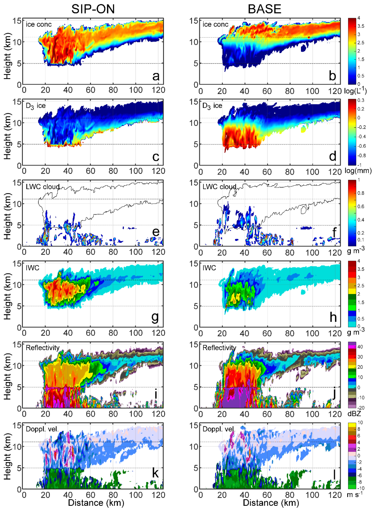
735 Figure 8. Vertical cross section domains of different parameters of GEM simulations for SIP-ON (left column) and BASE (right column) setups: (a,b) N_{ice} ; (c,d) D_3 ice ; (e,f) LWC_{cloud} ; (g,h) IWC ; (i,j) Z ; (k,l) U_{Doppl} . The cross sections were performed for the same vertical plane at 90 minutes on the modelled time. Horizontal dashed lines show levels corresponding to T = 0^\circ C ( H = 4.9 km ) and T = -40^\circ C ( H = 11.1 km ) levels.
