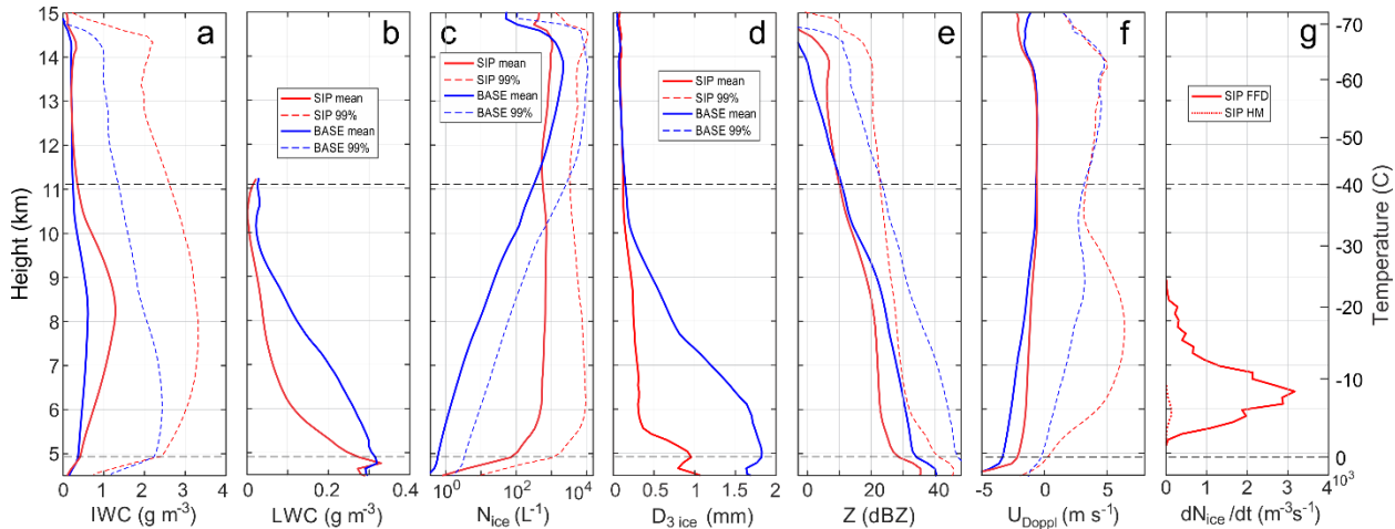
Figure 9. Average profiles of the results of SIP-ON (red) and BASE (blue) simulations. (a) IWC (solid) and IWC_{99} (dashed), (b) LWC (solid), (c) N_{ice} (solid) and N_{ice\ 99} (dashed), (d) D_{3\ ice} (e) Z (solid) and Z_{99} (dashed); (f) U_{Doppl} (solid) and U_{Doppl\ 99} (dashed); (g) ice crystal production rates for FFD (solid) and HM (dashed) for the SIP-ON simulation. The profiles spatially averaged over the cloud domain above the precipitation below the melting layer. The cloud domain was determined as the environment with IWC > 0.001 \text{ g m}^{-3} . The temporal averaging was performed over 13 modeling domains with time step 5 min within the time frame from 75 to 135 min.
