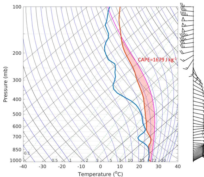
Figure B1C1. Initial atmospheric profiles for the idealized simulations. The blue line represents the dew point temperature, the red line represents the environment sounding (temperature), and the magenta line represents the parcel lapse rate. (Qu et al., 2022)
