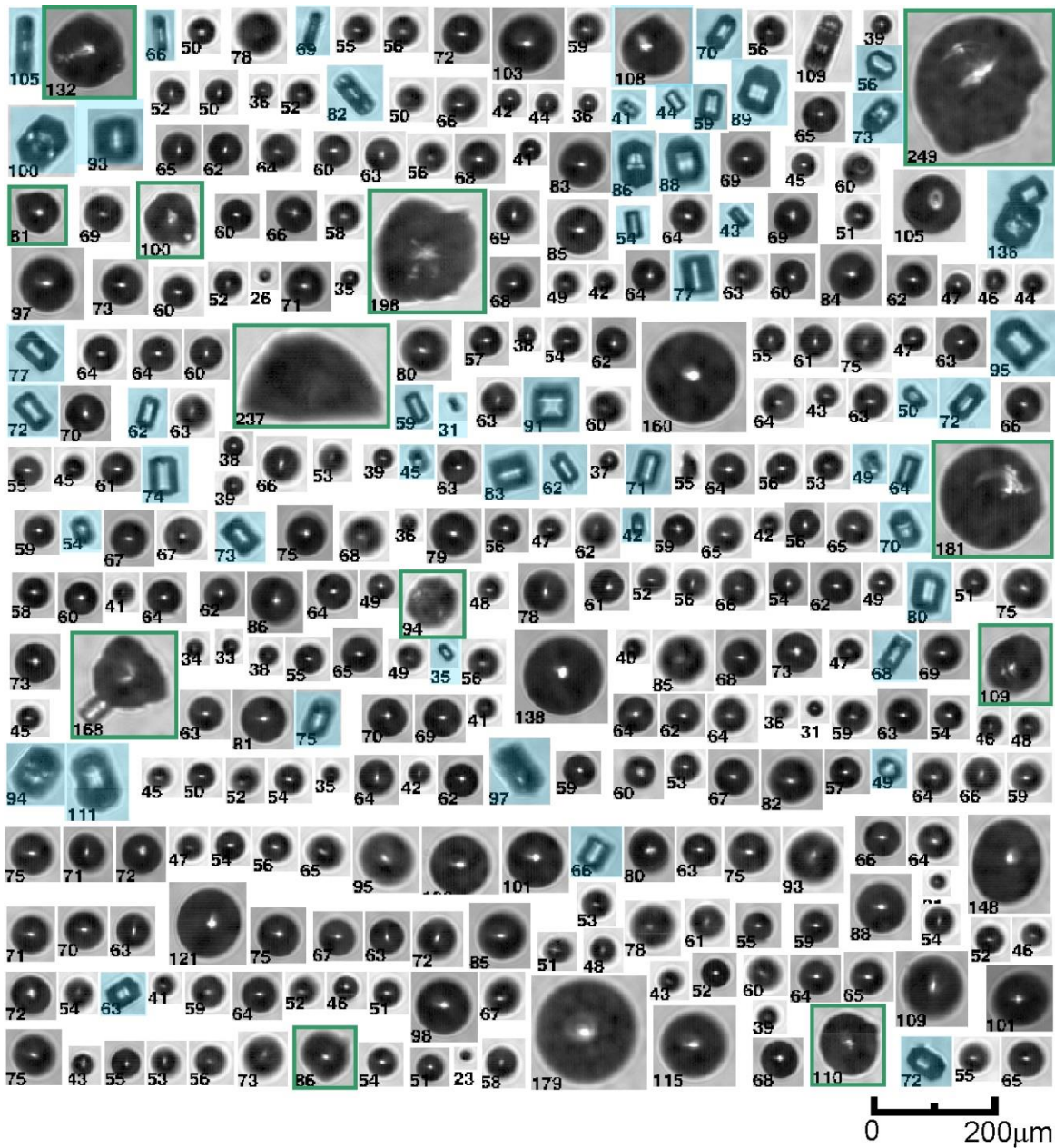
Figure A1. Zoomed-in images of cloud particles in Fig.1a showing details of shapes of secondary ice (highlighted in blue) and frozen drops (highlighted by green frames).
