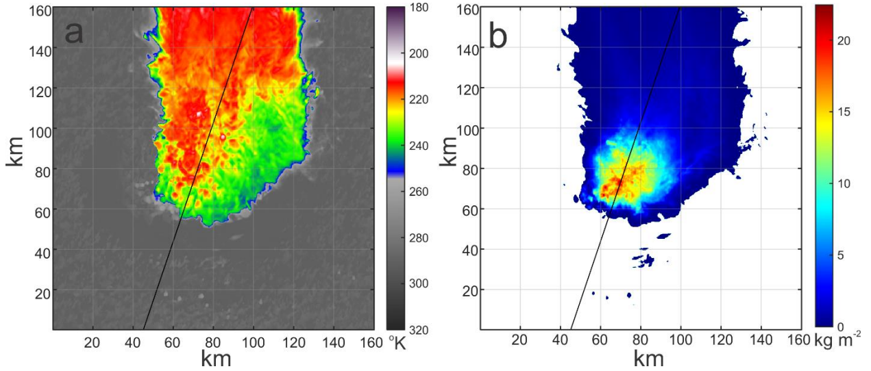
Figure C1D1. Brightness temperature at 11.2 \mu\text{m} (a) and ice water path (b) of the GEM simulated cloud system at 90 min. Black lines indicate the cross sections of the microphysical fields shown in Fig. 8.
