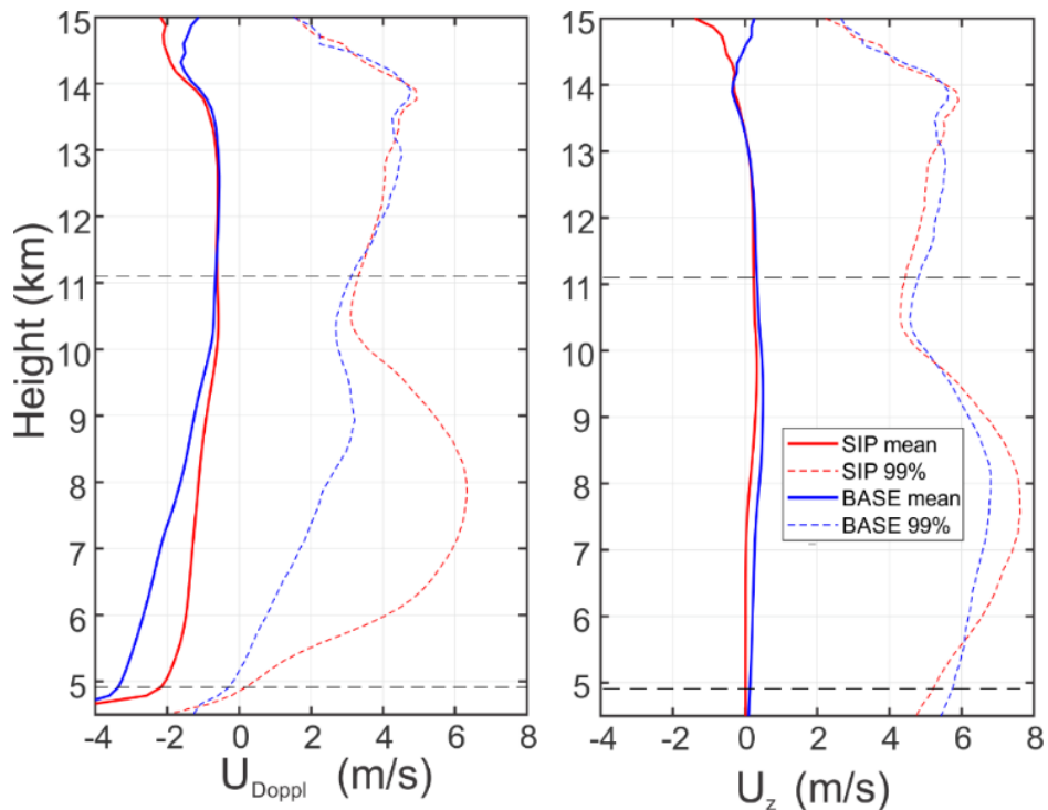
Figure C2D2. Average vertical profiles of GEM simulated Doppler velocity U_{Doppl} and vertical wind velocity U_z . The averaging was performed over time period from 75 to 135 min.
