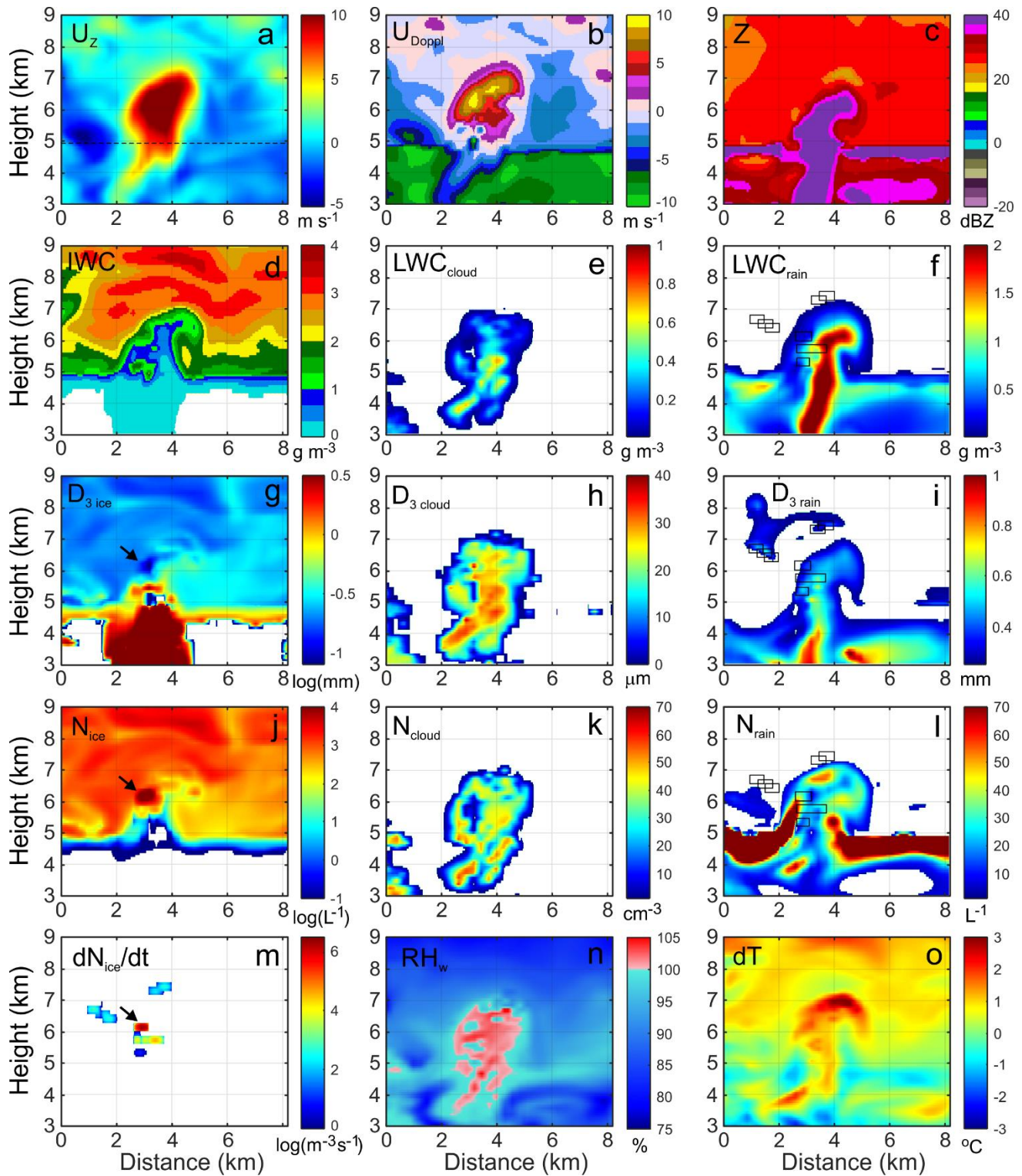
1010 Figure 12. Model microphysical and thermodynamical fields illustrating the effects of recirculating rain drops in convective updrafts on the FFD process. (a) vertical velocity U_z ; (b) Doppler velocity U_{Doppl} ; (c) radar reflectivity Z ; (d) IWC ; (e) LWC_{cloud} ; (f) LWC_{rain} ; (g) mean mass diameter of ice D_{3\ ice} ; (h) mean mass diameter of cloud droplets D_{3\ cloud} ; (i) mean mass diameter of rain drops D_{3\ rain} ; (j) ice particles number concentration N_{ice} ; (k) 1015 cloud droplets number concentration N_{cloud} ; (l) rain drops number concentration N_{rain} ; (m) SIP rate dN_{ice}/dt ; (n) relative humidity over liquid RH_w ; (o) temperature perturbation \Delta T . The rectangles in (f), (i), (l) indicate locations of the active SIP regions shown in (m).
