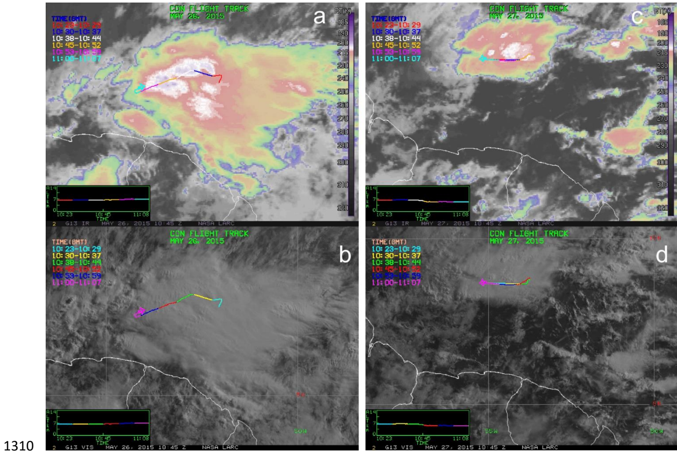
Figure A1B1. GOES-13 satellite infrared and visible images with the Convair-580 flight track for the flight segments shown in (a,b) Fig. 6 and (c,d) Fig. 7.
