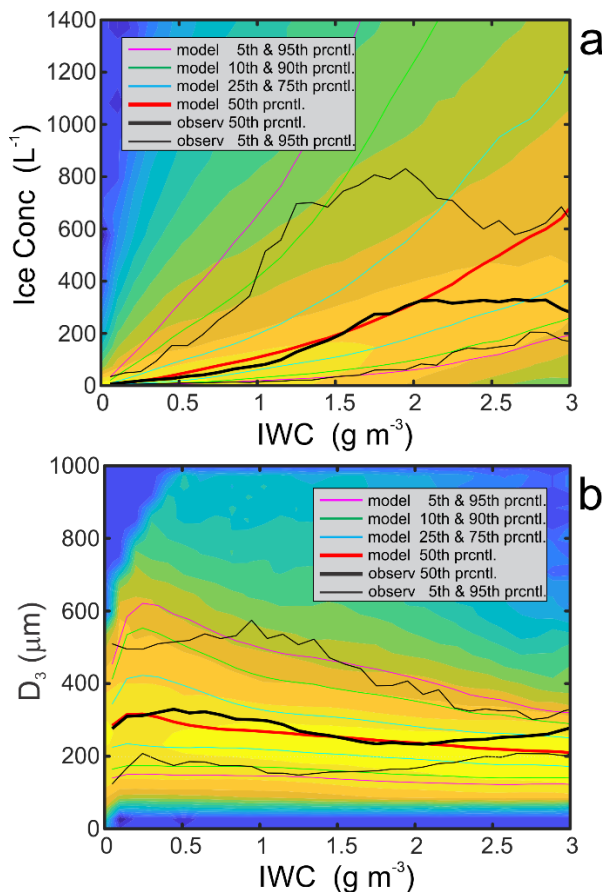
945 Figure 11. Comparisons of modeling results and in situ observations of IWC , D_{3\ ice} and N_{ice} . Fields of modeled (a) concentration of ice particles >40\ \mu m vs IWC and (b) equivalent volume diameter of ice particles vs IWC . Observed median (thick) and 5 th and 95 th percentile (thin) values are shown in black. The modeling data were averaged over time period from 75 to 135 min and the range of altitudes between 5.8 and 7.4 km corresponding to the CV580 sampling altitudes.
