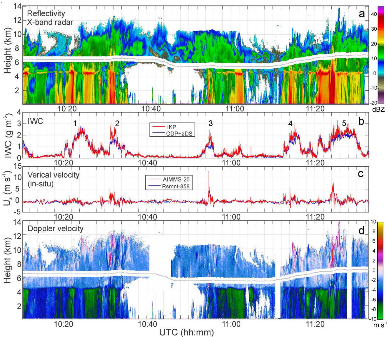
Figure 7. Time series of (a) X-band radar reflectivity, (b) IWC, (c) vertical velocity, (d) Doppler velocity measured by the X-band radar. The numbers in (b) indicate HIWC cell number (see text). The measurements were collected from the NRC Convair-580 on 27 May 2015.
