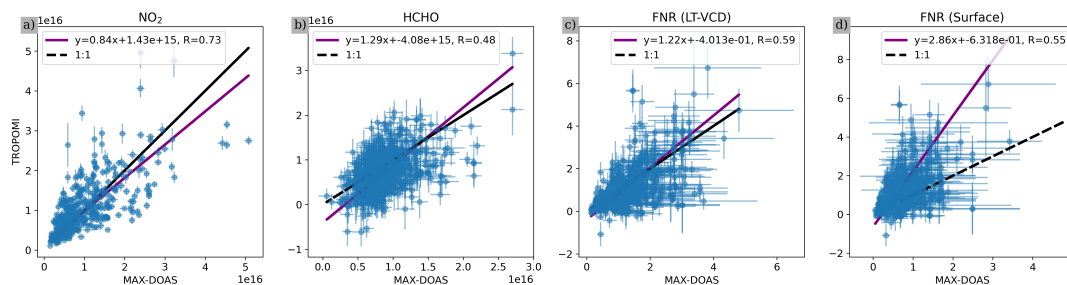
Figure 4. a) Correlation of hourly averaged MAX-DOAS NO 2 retrievals with tropospheric columns retrieved from TROPOMI. b) Correlation of hourly averaged MAX-DOAS HCHO retrievals with tropospheric columns retrieved from TROPOMI. c) Correlation of hourly averaged MAX-DOAS LT-VCD based FNRs with those calculated using tropospheric columns retrieved from TROPOMI. d) Correlation of hourly averaged MAX-DOAS surface based FNRs with those calculated using tropospheric columns retrieved from TROPOMI. The purple lines show the orthogonal distance regression, while the black dashed lines shows the 1:1 relationship. Uncertainties for both retrievals are shown in blue.
