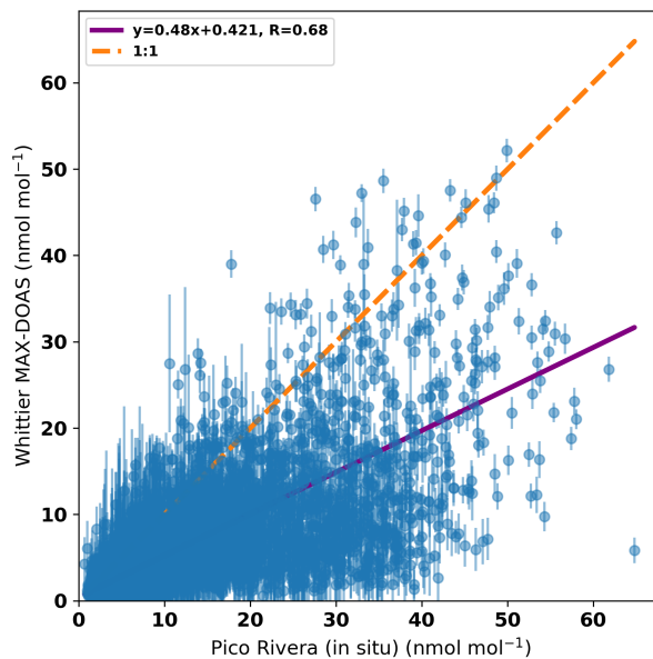
Figure 3. Correlation of hourly averaged MAX-DOAS measurements with in situ NO 2 data from the California Air Resources Board site in Pico Rivera, 5 km north of the college. The purple line shows the linear regression, while the orange line shows the 1:1 relationship.
