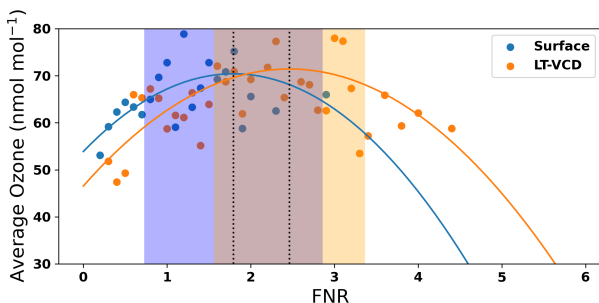
Figure 2: Determination of ozone formation regimes from ground-based MAX-DOAS data collected at the TROPOMI overpass time. Ozone values binned by surface FNR are shown in blue, while those binned by LT-VCD FNR are shown in orange. Second order polynomial fits are shown using solid lines, with the shaded region representing the uncertainty in the maximum value. Dashed vertical lines represent the maximum probability of an ozone exceedence as a function of FNR for both methods.
