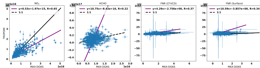
Figure 1: a) Correlation of hourly averaged MAX-DOAS \text{NO}_2 retrievals with tropospheric columns retrieved from TROPOMI. b) Correlation of hourly averaged MAX-DOAS HCHO retrievals with tropospheric columns retrieved from TROPOMI. c) Correlation of hourly averaged MAX-DOAS LT-VCD based FNRs with those calculated using tropospheric columns retrieved from TROPOMI. d) Correlation of hourly averaged MAX-DOAS surface based FNRs with those calculated using tropospheric columns retrieved from TROPOMI. The purple lines show the orthogonal distance regression, while the black dashed lines shows the 1:1 relationship. Uncertainties for both retrievals are shown in blue.
