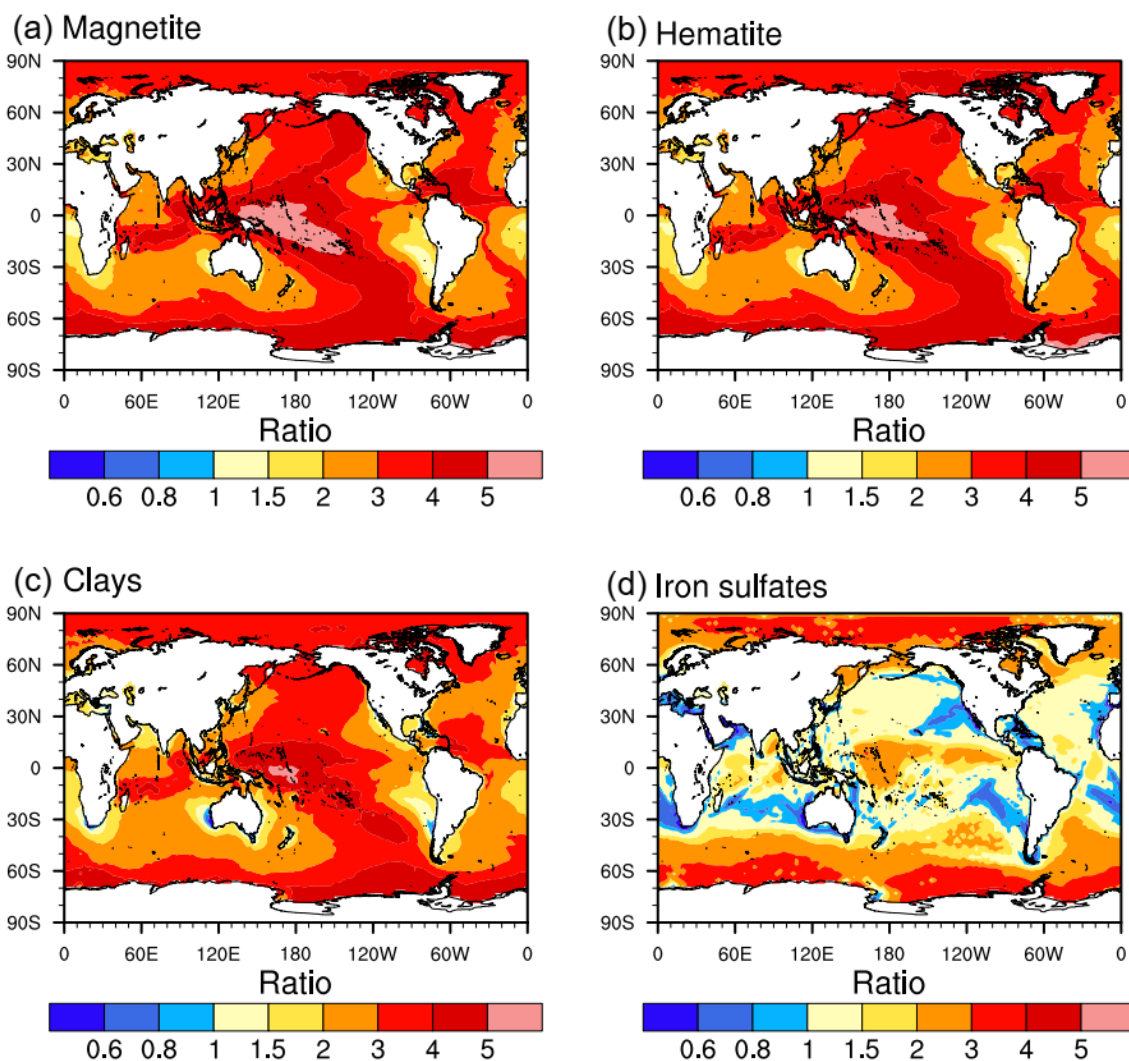
270 271 Fig. 6. Ratios of yearly accumulated soluble iron deposition for four anthropogenic iron-containing minerals, comparing fine- 272 sized and coarse-sized cases.
