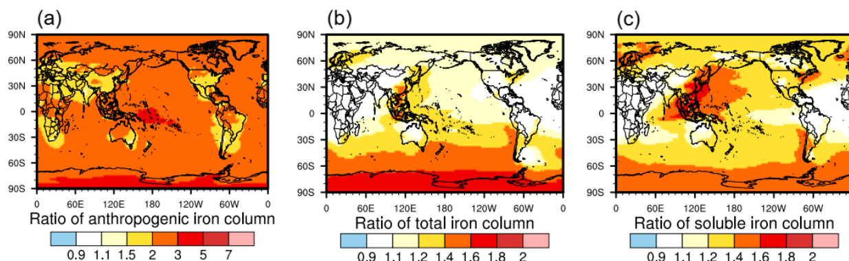
221 Fig. 4. Global map of variability in yearly averaged iron column concentrations between the fine-sized group and the coarse- 222 sized group. The variability ratios (fine-sized/coarse-sized) are calculated for (a) anthropogenic iron, (b) total iron, and (c) 223 soluble iron, respectively. Herein, total iron is a combination of iron from dust, biomass burning, and anthropogenic sources, 224 the soluble form of which denotes soluble iron. The ratios represent the maximum differences between the fine-sized group 225 (the Moteki2017 and Rathod2020 cases) and the coarse-sized group (the Hamilton2019 and Wang2015 cases) and indicate the 226 spread of iron simulations.
