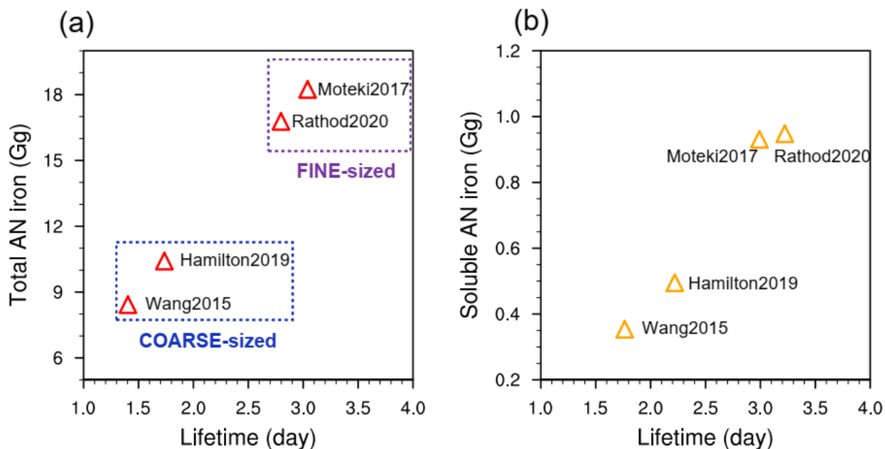
186 187 Fig. 2. Global anthropogenic iron concentration burdens and lifetimes varied by the emission size distributions. The scatter 188 plots are shown for (a) anthropogenic iron (labeled as AN iron) burden vs. lifetime and (b) soluble anthropogenic iron vs. 189 lifetime. Four representative cases are examined in this work: Moteki2017, Rathod2020, Hamilton2019, and Wang2015. The 190 first two cases are grouped into “FINE-sized” and the other two are grouped into “COARSE-sized”.
