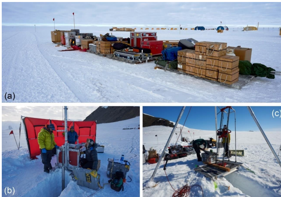
220 Figure 3: Equipment needed for shallow subglacial bedrock drilling. (a) In the foreground, all cargo (except snowmobiles and fuel) deployed for 2019-20 drilling campaign at Mt Murphy. (b) US Ice Drilling Program “Eclipse” ice drill in use at Mt Murphy. (c) US Ice Drilling Program “Winkie” drill, and associated equipment. The Eclipse drill is used to drill through ice to access the bedrock whilst the
