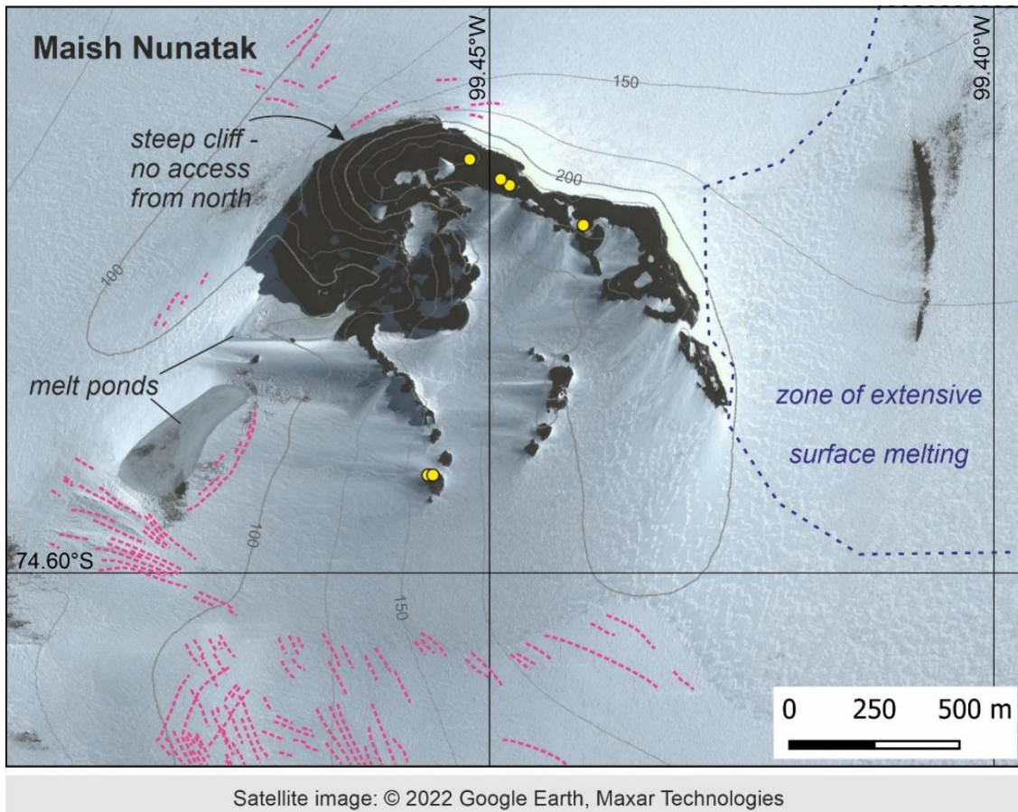
610 Figure 14. Satellite image of Maish Nunatak showing features that are important for drill site accessibility. Pink dotted lines show location of crevasses. Locations of erratic cobbles dated by Johnson et al. (2014) are indicated by yellow circles (see also Fig. 13b). No GPR surveys were undertaken at this site. Contours of surface elevation (at 25 m intervals) are from the REMA DEM (Howat et al., 2022). Satellite image ©2022 Google Earth, Maxar Technologies (imagery date: 2 March 2012).
