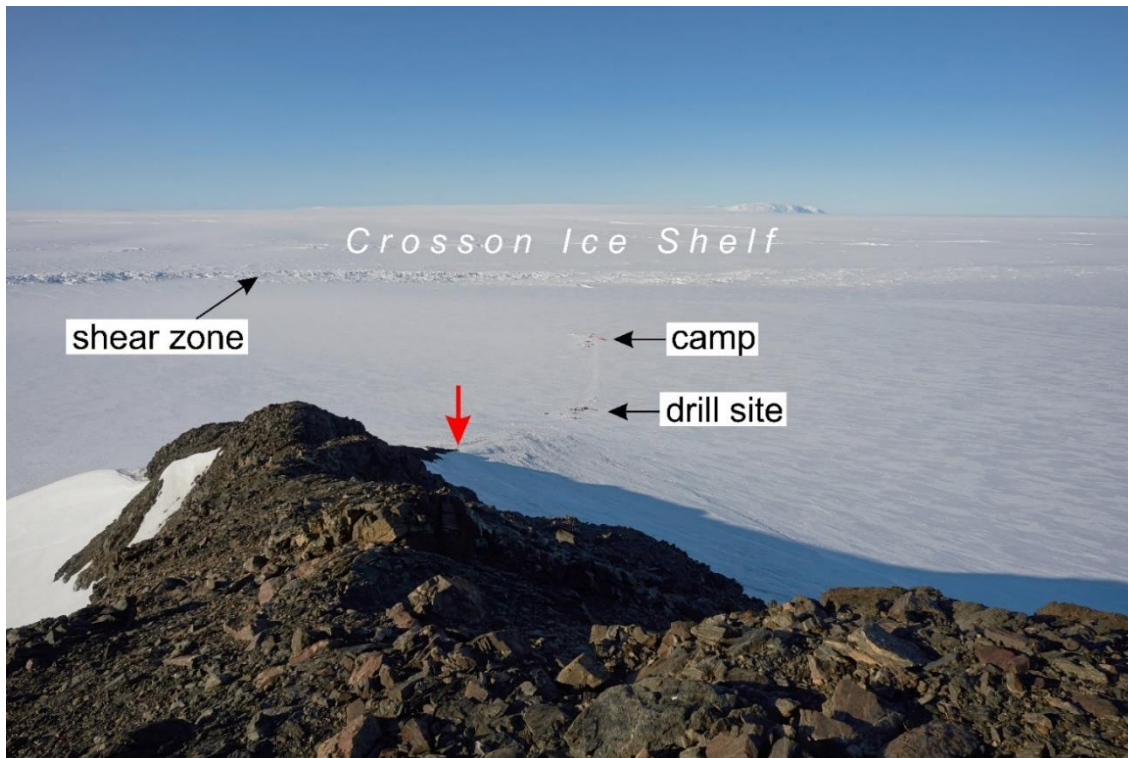
170 Figure 2: Photograph of a drill site at the Mt Murphy massif in the central Amundsen Sea Embayment. At the location marked by the red downward pointing arrow, the bedrock ridge (foreground) extends north from Kay Peak (Fig. 1a) below the ice sheet surface in a direction perpendicular to the present grounding line less than 2 km away (demarcated by shear zone crevasses). Its orientation and close proximity
