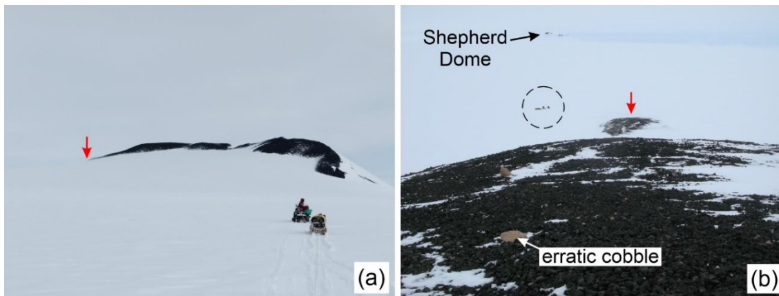
405 Figure 5: Topography and surroundings of Winkie Nunatak. (a) Photograph of Winkie Nunatak viewed from the north. Arrow indicates where the SE ridge extends below the ice surface. Sledge and snowmobile for scale. (b) View from Winkie Nunatak looking down the SE ridge towards Shepherd Dome. Red down-pointing arrow shows tip of ridge. Note erratic cobbles strewn on lava bedrock surface. Sledge and two snowmobiles (circled) for scale.
