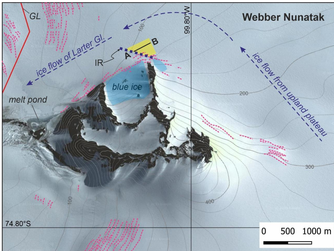
Figure 10. Satellite image of Webber Nunatak, showing areas of known crevassing and blue ice. Pink dotted lines and blue shaded areas show location of crevasses and blue ice, respectively. The location of the radar profile (A-B) shown in Fig. 12a and b is indicated by a shaded yellow box that outlines the survey area used to compile Fig. 12c. The dotted line labelled ‘IR’ shows the base of a ridge in the ice sheet surface. Numerous large crevasses were observed on the ridge slope to the SW of the line. Contours of surface elevation (at 25 m intervals) are from the REMA DEM (Howat et al., 2022). The solid red line (labelled ‘GL’) marks the location of the 2011 grounding line (Rignot et al., 2016). Satellite image ©2022 Google Earth, Maxar Technologies (imagery date: 16 February 2012).
