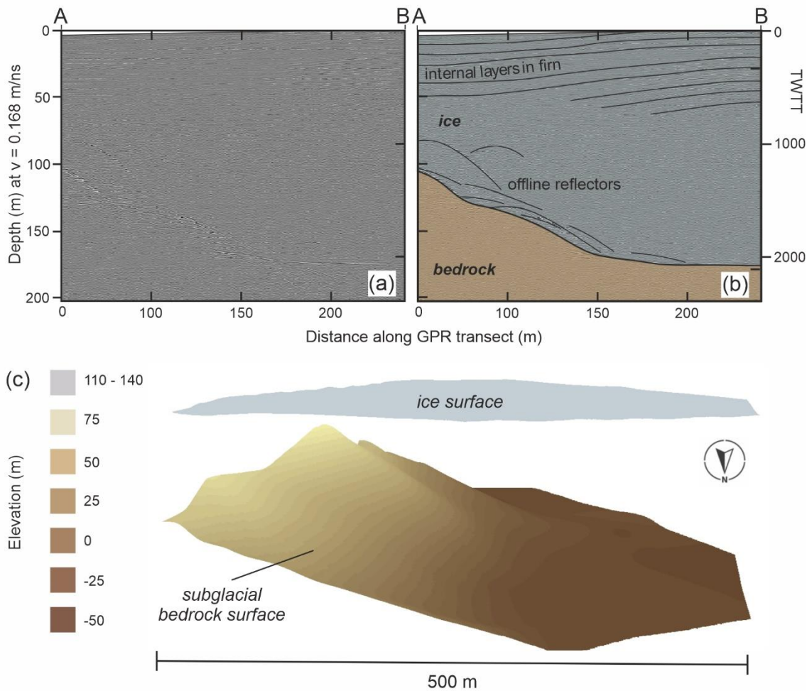
570 Figure 12. GPR analysis of Webber Nunatak. (a) and (b) 2D radar profile from Webber Nunatak , showing subglacial ridge crest (location of profile A-B is shown in Fig. 10). TWTT is two-way travel time. Panel (b) shows digitised basal topography and the ice surface and is annotated to show subsurface features (thin black lines). (c) Radar-based interpolation of the subglacial ridge.
