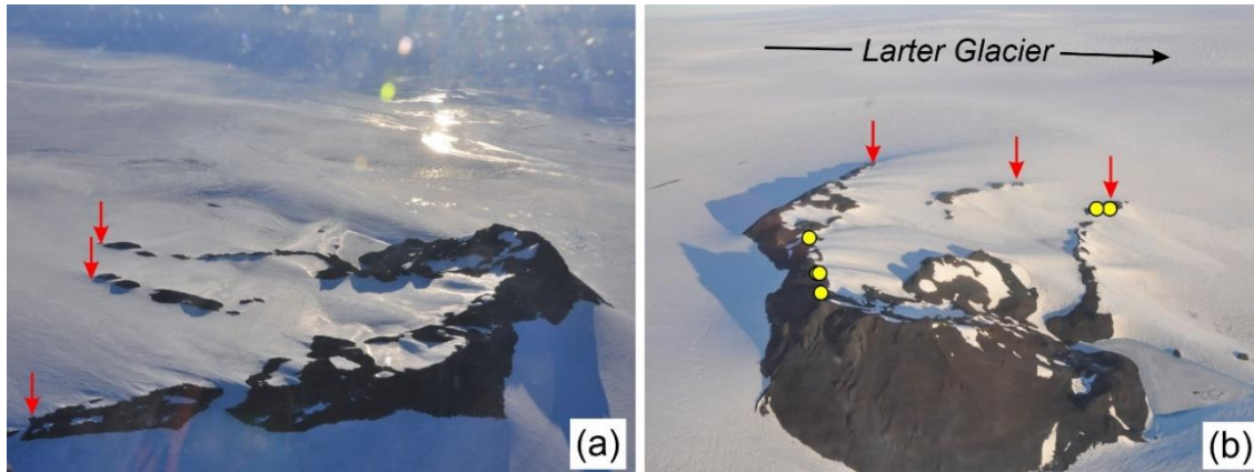
Figure 13. Topography and surroundings of Maish Nunatak. (a) View from the air, looking SW. Arrows indicate the tips of three low-gradient bedrock ridges described in the text: the distance between the outer ridges is 880 m. (b) View looking approximately SE, towards Larter Glacier. Circular symbols indicate the locations of erratic cobbles sampled for 10 Be exposure dating in an earlier study (Johnson et al., 2014). As in panel (a), the outermost ridges are separated by a distance of 880 m. Both photographs were taken in 2010 by James Smith (British Antarctic Survey).
