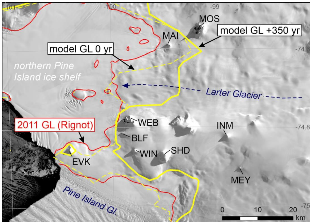
305 Figure 4: Position of present and modelled (future) grounding lines relative to nunataks in the Hudson Mountains region. The modern (2011) observed grounding line position is shown as a solid red medium-thickness line (Rignot et al., 2016). The modelled grounding line position at present-day (model GL 0 yr) is shown as a thin dashed yellow line, and at 350 years into the future (model year 2350) as a thick yellow line (model GL +350 yr). Both are from the NSM simulations of Larour et al. (2019). The underlying satellite image is Landsat-8, courtesy of USGS. Nunataks mentioned in the text are labelled as follows: EVK (Evans Knoll), BLF (World's End Bluff), WEB (Webber Nunatak), WIN (Winkie Nunatak), SHD (Shepherd Dome), INM (Inman Nunatak) , MEY (Meyers Nunatak) , MAI (Maish Nunatak), MOS (Mt Moses). 310
