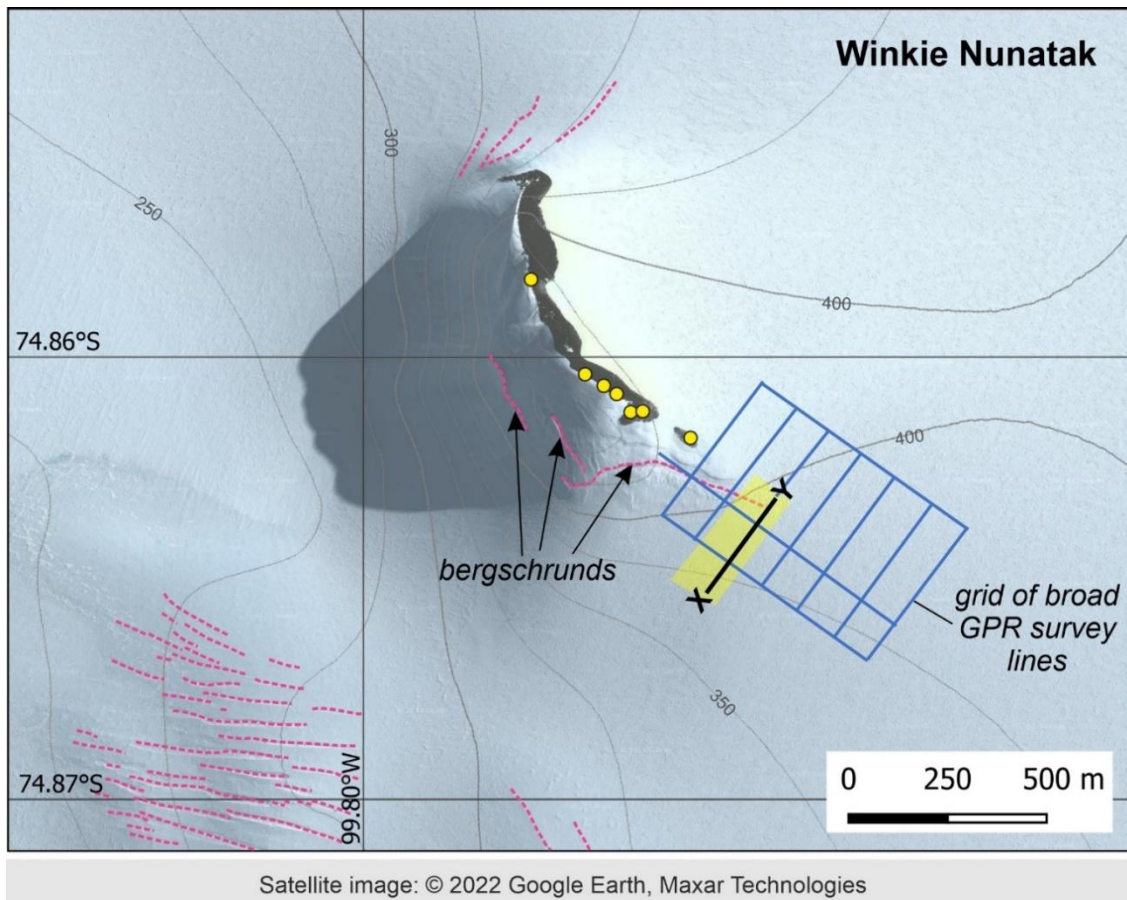
Figure 6: Satellite image of Winkie Nunatak, showing areas of known crevassing (pink dotted lines). Contours of surface elevation (at 25 m intervals) are from the REMA DEM (Howat et al., 2022). Satellite image ©2022 Google Earth, Maxar Technologies (imagery date: 16 February 2012). Locations of erratic cobbles dated by Nichols et al. (2023) are indicated by yellow circles. The location of radar profile (X-Y) in Fig. 8 is shown here inside a shaded yellow rectangle that outlines the coverage of our detailed survey grid (five lines; see Appendix A). The lines of the broader GPR survey (Appendix A) are also shown.
