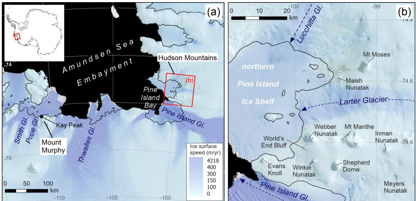
150 Figure 1: The location of the Hudson Mountains study site within the Amundsen Sea sector of Antarctica. (a) Map of Amundsen Sea Embayment, showing location of subglacial bedrock drilling sites near Kay Peak, Mt Murphy (Fig. 2) and Hudson Mountains. (b) Location
