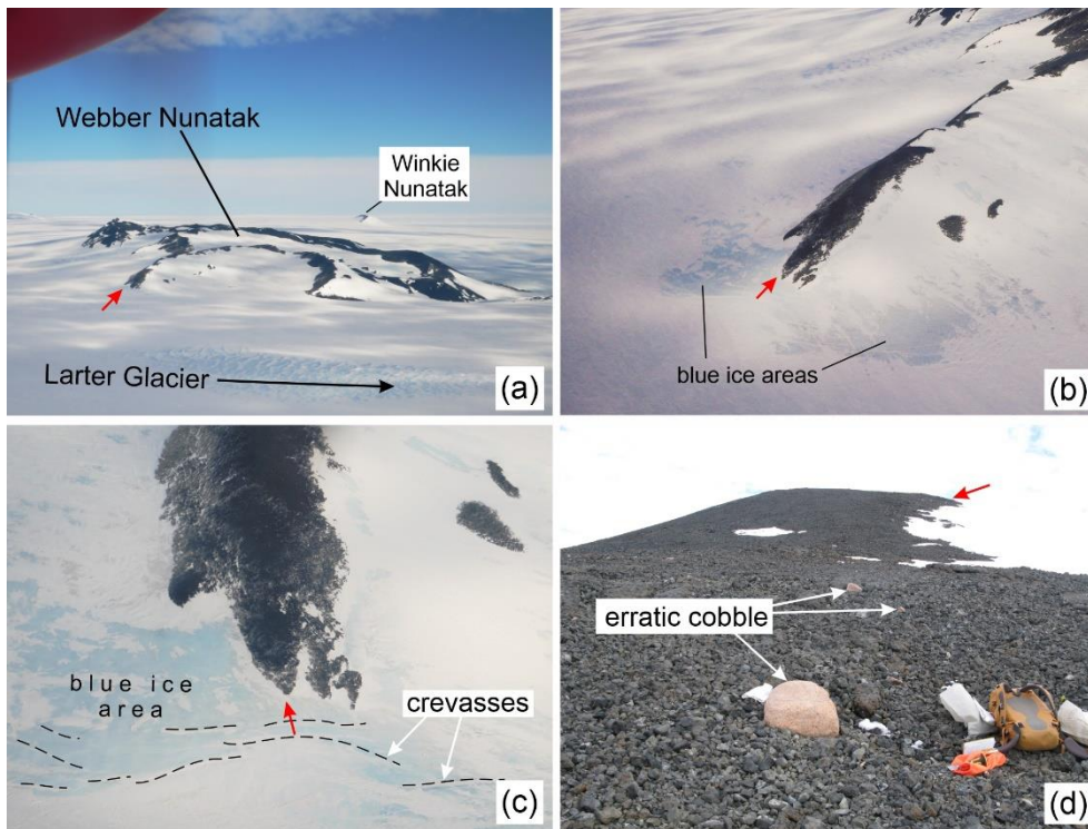
Figure 9. Topography and glaciology around Webber Nunatak. Short red arrows denote ‘Ridge A’ (see text). close to the candidate drill site. (a) Webber Nunatak viewed from Larter Glacier, showing candidate drill site (off end of Ridge A). Note extensive crevassing on Larter Glacier, preventing access by aircraft from the northern side. The nunatak length from left to right in the image is 3.5 km. (b) Ridge A ( width ~150 m ) viewed from the air. (c) Close-up view of ridge A ( width ~150 m ) and the adjacent blue ice area, viewed from above. Several crevasses are visible extending perpendicular to the ridge. (d) The lower part of Ridge A, looking towards Larter Glacier. A few erratic cobbles are perched on the basalt rubble. Rucksack and field equipment for scale; the cobble in the foreground is 50 cm diameter.
