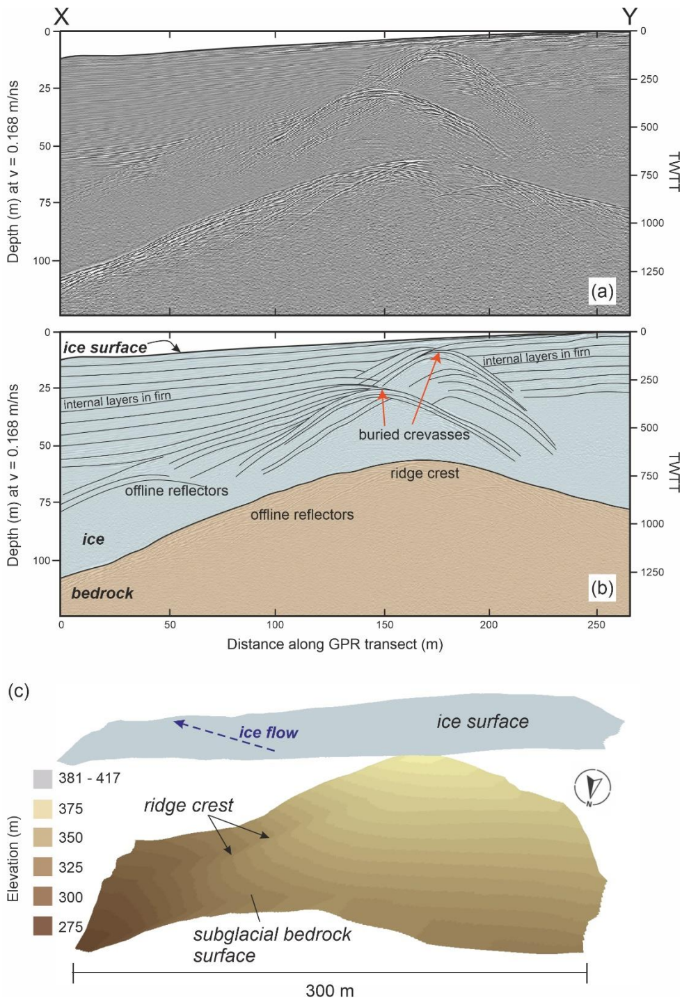
475 Figure 8. GPR survey results from Winkie Nunatak. (a) 2D radar profile (the location of profile X-Y is shown in Fig. 6). TWTT is two-way travel time. (b) 2D radar profile showing digitised basal topography and ice. Subsurface features including firn layers, crevasses and offline reflectors from basal bedrock are labelled. (c) Radar-based interpolation of the subglacial bedrock ridge at Winkie Nunatak (the area covered by these data is shown in Fig. 6).
