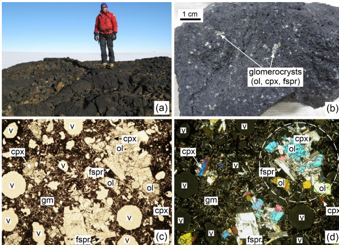
625 Figure 15. Photographs showing bedrock lithology at Maish Nunatak. (a) Field photograph of pillow lavas, with person for scale. (b) Close-up photograph of lava in hand specimen, showing prominent clusters (glomerocrysts) of olivine (ol), clinopyroxene (cpx) and feldspar (fspr). (c) Thin section photograph of lava (sample MAI-201; British Antarctic Survey ID R19.6.1), in PPL. Field of view is 8 mm. v=vesicle, gm=groundmass, cpx=clinopyroxene, ol=olivine, fspr=feldspar. (d) Thin section photograph of same lava as in panel c, in XPL. A 630 glomerocryst is enclosed by the dashed white line. Field of view is 8 mm. v=vesicle, gm=groundmass (comprising feldspar and clinopyroxene crystals)
