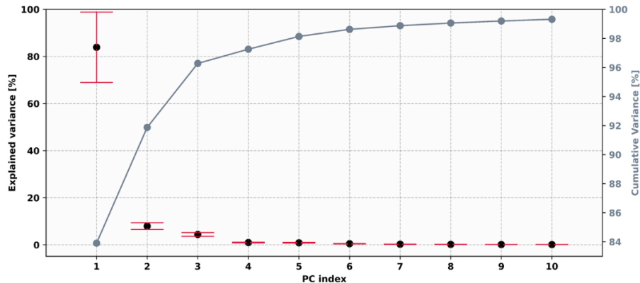
Figure S2. Eigenvalues of the top ten leading modes of variability for the annual H0 field in Patagonia, obtained through the EOF analysis (black dots), and their associated typical errors (red bars), following the method of North et al., (1982). Moreover, the accumulated percentage of the total variance explained by each principal component (gray dots) is depicted on the right axis.
