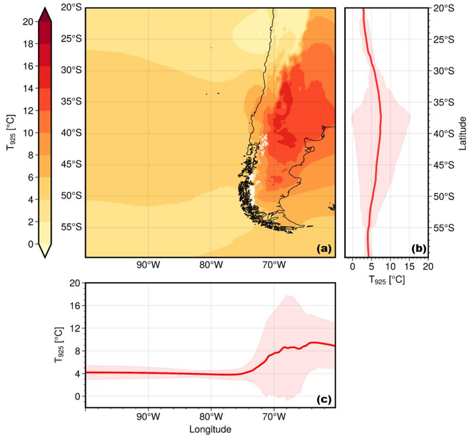
Figure S3. Spatial distribution of the January minus July mean air temperature at 925 hPa. Lighter areas depict a lower temperature, while red areas indicate higher values. The white contours delineate the extent of ice coverage in the region. Each distribution is accompanied by a latitudinal profile (b) and a longitudinal profile (c), showcasing the spatially averaged temperature values. The red shaded area in these profiles represents the interquartile range.
