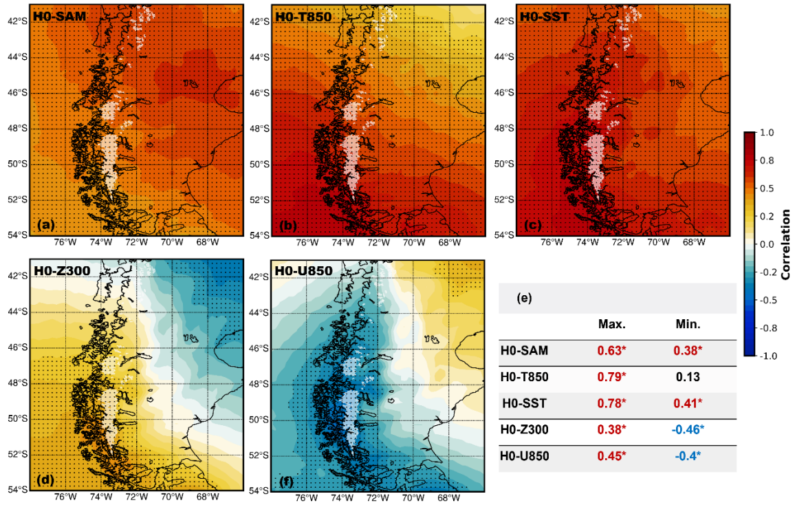
Figure S4. Spatial correlation maps between the detrended annual mean isotherm field and the detrended custom indices timeseries SAM (a), T850 (b), SST (c), Z300 (d), and U850 (f). The white contours outline the ice coverage boundaries within the region. Black circles denote statistically significant correlations. (e) Correlation chart with the maximum and minimum values of every spatial field showed, where the asterisk symbol (*) indicates statistical significance ( p -value < 0.05). Red (blue) correlation values depicted positive (negative) correlations.
