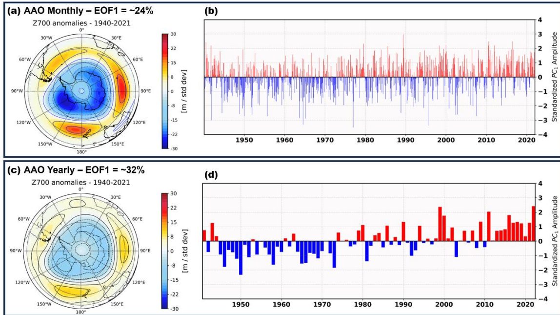
Figure S1. Leading Empirical Orthogonal Function (EOF) of ERA5 700 hPa geopotential height through two datasets: (a) monthly mean data, and (c) annual mean data spanning from 1940 to 2021. The EOFs are generated from detrended 700 hPa geopotential height anomaly data, weighted by the square root of the cosine of latitude, within the latitude range of 20^{\circ} to 90^{\circ} S. The resulting patterns are displayed as regression maps, depicting the interplay between the leading Principal Component (PC) time series and the spatial distribution of the evolving height anomalies (b and d, respectively). The temporal pattern is illustrated by blue and red bars (negatives/positive values) of the first Principal Component, scaled to unit variance (divided by the square root of its eigenvalue). Each panel includes insights into the proportion of explained variance and showcases the standardized PC time series grounded in the NOAA Climate Prediction Center's (CPC) 1979-2000 reference period.
