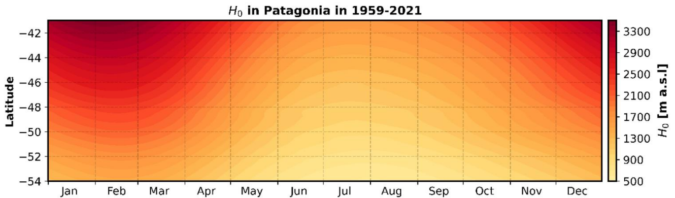
225 Figure 6: Latitudinal profile of daily climatology of H_0 in Patagonia from 1959 to 2021.
