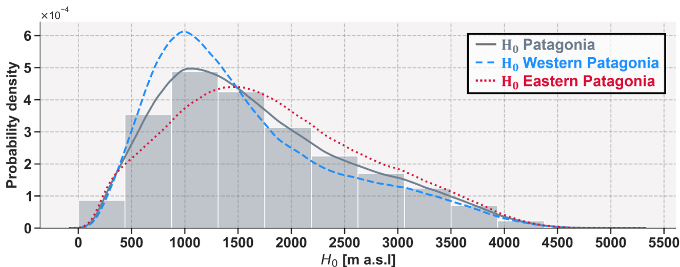
Figure 5: Histogram of daily simulated 0°C isotherm height in Patagonia. The grey bars represent the daily values of H_0 obtained from the spatial average across the entire study area from 1959 to 2021. The curves, on the other hand, indicate the fit of the kernel density estimation for the entire region (grey), Western Patagonia (blue), and Eastern Patagonia (red).
