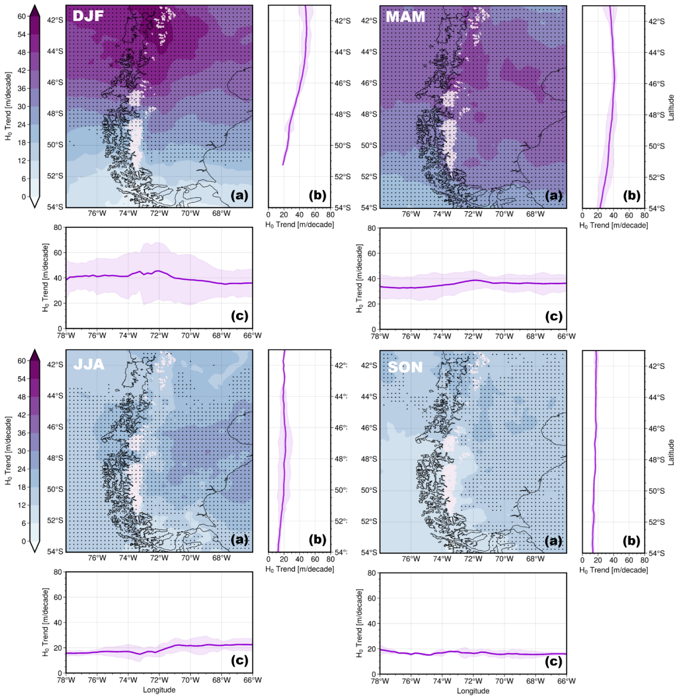
290 Figure 8: Spatial distribution of the 0^{\circ}\text{C} isotherm trends ( H_0 ) across the seasons. Lighter areas depict a lower height of the trends, while purple areas indicate higher values. The white contours delineate the extent of ice coverage in the region. Each distribution is accompanied by a latitudinal profile (b) and a longitudinal profile (c), showcasing the spatially averaged H_0 trend values. The purple shaded area in these profiles represents the respective interquartile range for each profile ( \text{IQR}_{m,z} ). Black circles denote statistically significant trends at p\text{-value} < 0.05 .
