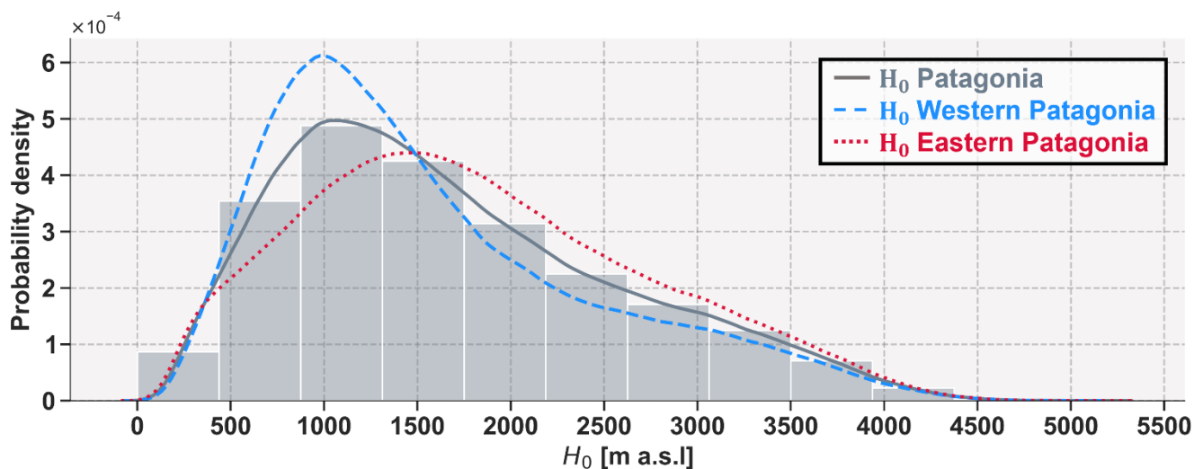
Figure 5: Histogram of daily simulated 0°C isotherm height in Patagonia. The gray bars represent the daily values of H_0 obtained from the spatial average across the entire study area from 1959 to 2021. The curves, on the other hand, indicate the fit of the kernel density estimation for the entire region (gray), Western Patagonia (blue), and Eastern Patagonia (red).
