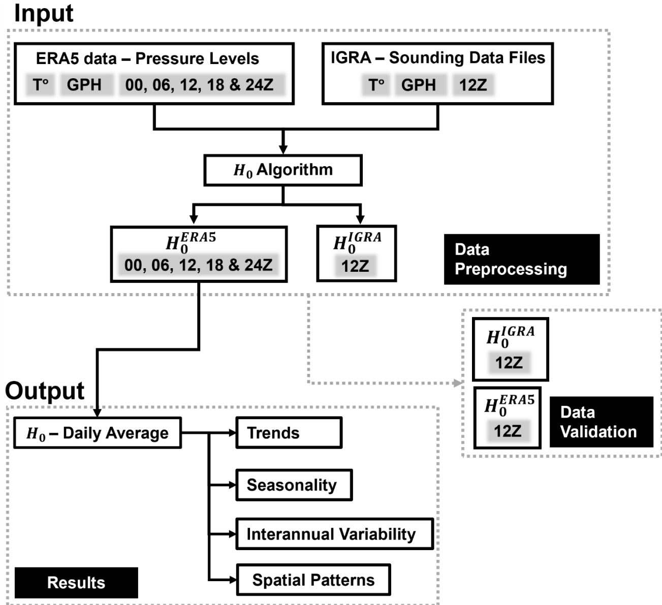
145 Figure 2: The data processing workflow for H_0 between 1959 and 2021. Two distinct sets of input data were utilized: one comprising reanalysis data and the other containing radiosonde observations. The isotherm 0^\circ\text{C} values were derived from these datasets, and a validation process was employed. Daily values were computed based on the reanalysis data.
