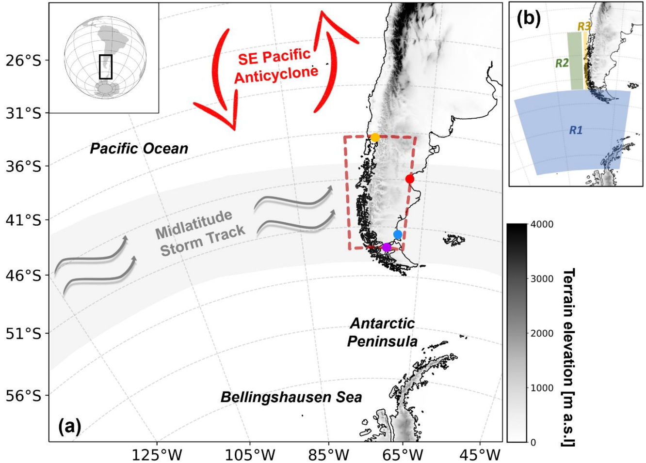
Figure 1: a) Topographic map of South America highlighting key features in the Patagonia region. Terrain elevation (m a.s.l) acquired from ETOPO1 model with 1 arcmin resolution. The red rectangle indicates the study region of Patagonia. The dots indicate the locations of the radiosonde stations of Puerto Montt (orange), Comodoro Rivadavia (red), Río Gallegos (blue), and Punta Arenas (purple). b) Coloured areas represent the regions used for the construction of custom climate indices.
