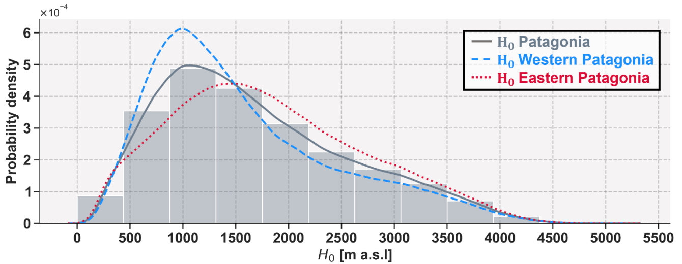
225 | Figure 5: Histogram of daily simulated 0°C isotherm height in Patagonia. The gray bars represent the daily values of H_0 obtained from the spatial average across the entire study area from 1959 to 2021. The curves, on the other hand, indicate the fit of the kernel density estimation for the entire region (gray), Western Patagonia (blue), and Eastern Patagonia (red).
