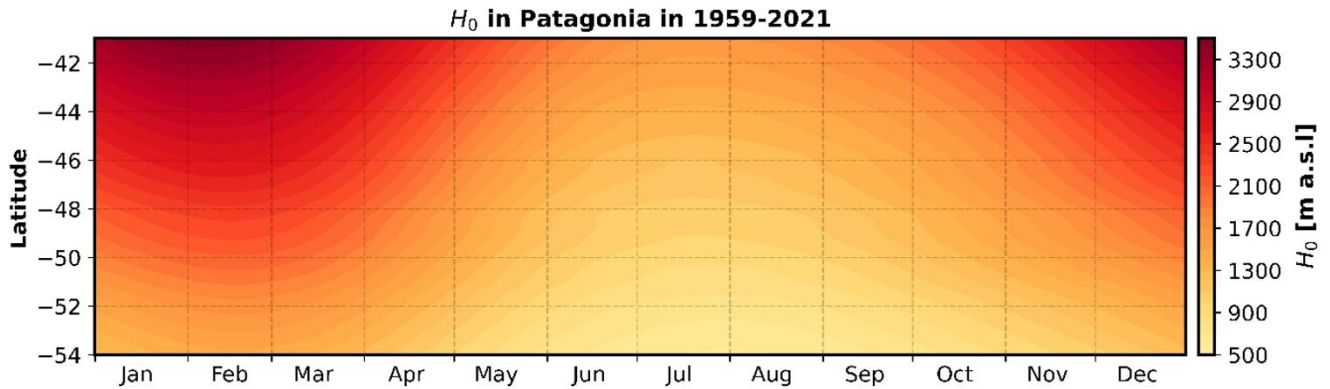
235 | Figure 6: Latitudinal profile of daily climatology of H_0 in Patagonia from 1959 to 2021.
