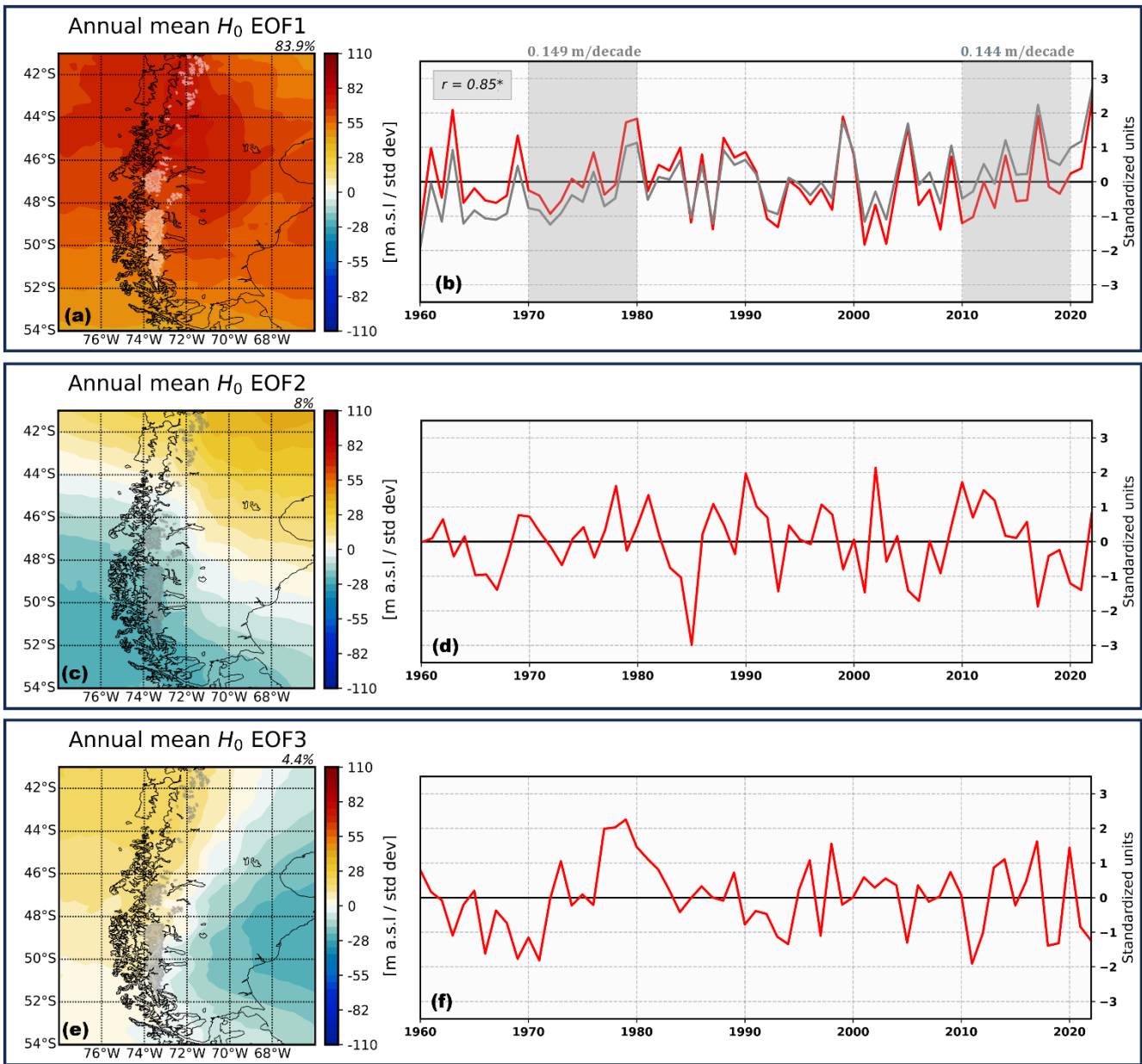
Figure 9: First three leading modes of variability extracted through an Empirical Orthogonal Function (EOF) analysis conducted on Patagonia's annual freezing level field spanning from 1959 to 2021. (a, c & e) The resulting patterns are presented as regression maps, illustrating the relationship between the leading Principal Component (PC) time series and the spatial distribution of the time-varying height anomalies. Additionally, the temporal pattern is illustrated by the first Principal Component (red line), scaled to unit variance (divided by the square root of its eigenvalue), while the grey line portrays the standardized anomalies of the spatial average of the annual freezing level field across Patagonia (b, d & f). In panel b, the grey box indicates Pearson's correlation between these two patterns and the grey contour area represents the periods with highest anomaly trend with their respective values. We continue the analysis for the second and third modes of variability (c-d and e-f, respectively). However, these modes show low correlation values with the freezing level anomalies, and thus, the focus is shifted away from freezing level anomalies in these cases. The white (a) and gray (c & e) contours delineate the extent of ice coverage in the region.
