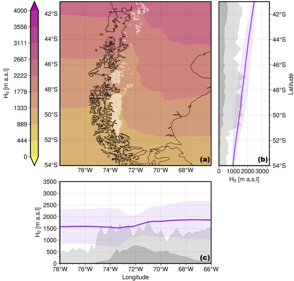
195 Figure 4: (a) Spatial distribution of the annual average of H 0 . Lighter areas depict a lower height of H 0 , while red areas indicate higher values. The white contours delineate the extent of ice coverage in the region. Each distribution is accompanied by a (b) latitudinal profile and (c) a longitudinal profile, showcasing the spatially averaged H 0 values. The purple shaded area in these profiles represents the respective interquartile range for each profile (IQR m,z ). The grey contours illustrate topographic profiles corresponding to the 2.5th percentile (dark grey) and 97.5th percentile (light grey).
