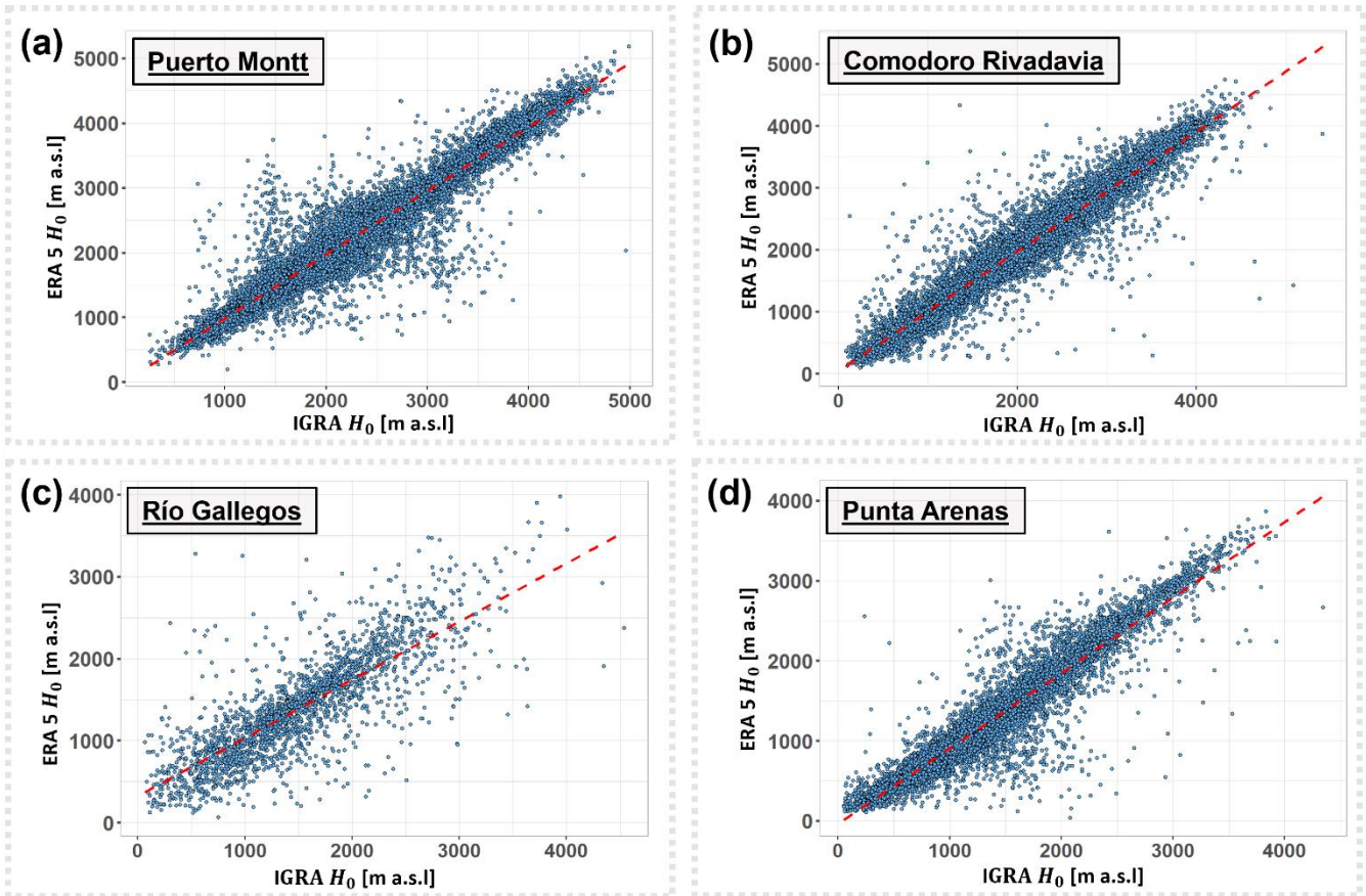
175 Figure 3: Scatterplots from Puerto Montt (a), Comodoro Rivadavia (b), Río Gallegos (c) and Punta Arenas (d). The reference data corresponds to H_0^{ERA5} (closest grid point) and H_0^{IGRA} . The red dotted line in scatterplots shows the 1:1 line.
