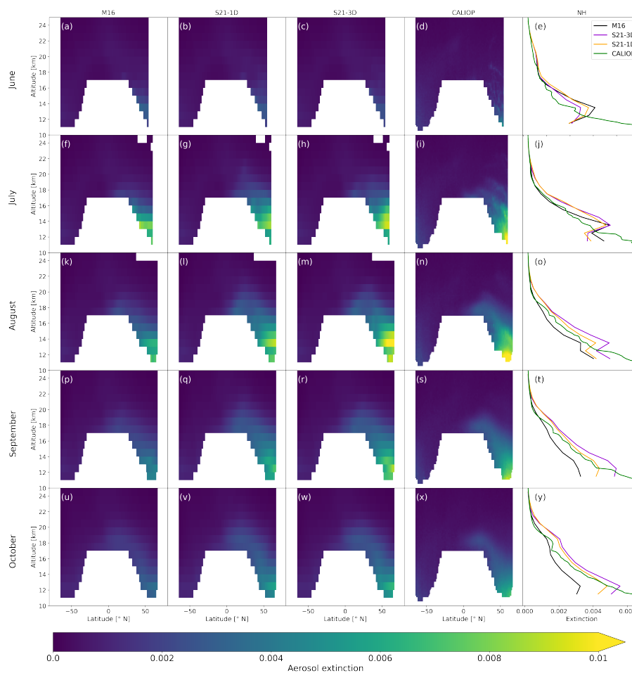
Figure 6. Monthly mean stratospheric evolution of the aerosol extinction coefficient for the three simulations and satellite observations from CALIOP. The first three columns show the simulations, (M16, S21-1D, and S21-3D), and the fourth column represents the CALIOP observations. The fifth column shows the average vertical aerosol extinction profiles in the NH for both simulations and the observations. The rows correspond to different months, starting from June to November 2009. The white areas are excluded values located in the troposphere, and missing latitudes in CALIOP. Note that the simulations have a wavelength of 550 nm whereas CALIOP observations have a wavelength of 532 nm.
