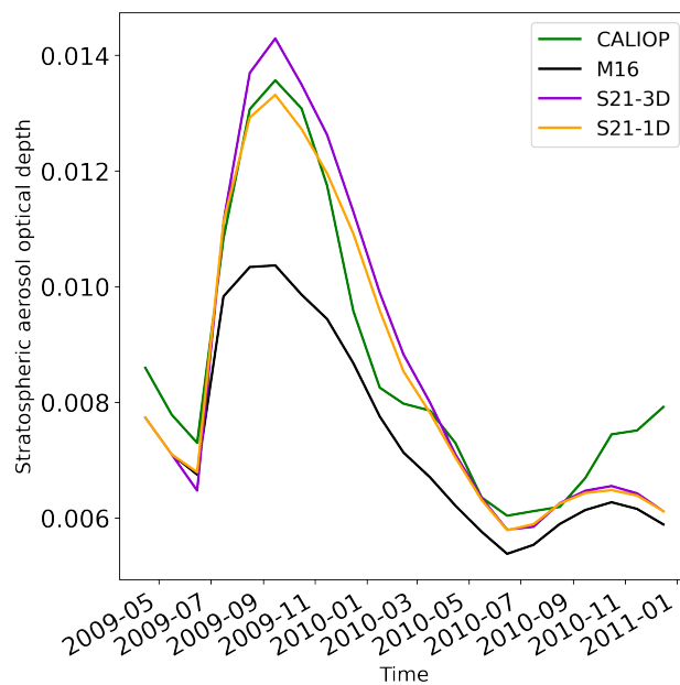
Figure 7. Stratospheric Aerosol optical depth (AOD) for the three simulations M16, S21-3D, and S21-1D, compared with observations by CALIOP. Note that the simulations show AOD at 550 nm whereas CALIOP observations provide AODs at a wavelength of 532 nm.
