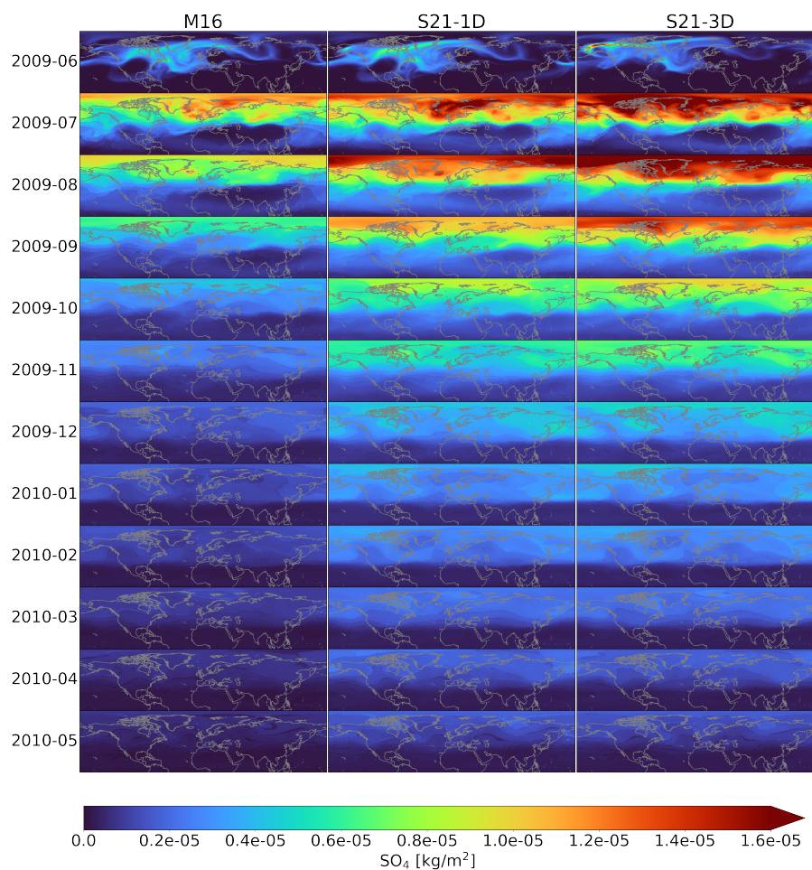
Figure 5. Monthly mean of stratospheric \text{SO}_4 in the NH during the first year post the volcanic eruption. To isolate the volcanic \text{SO}_4 we have subtracted the \text{SO}_2 levels in the No-Volc simulation from the other three simulations.
