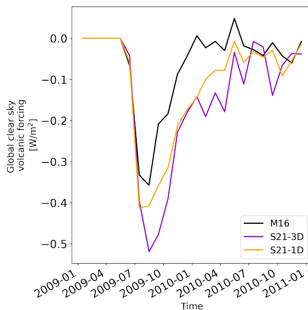
Figure 8. Global clear sky volcanic forcing from the Sarychev eruption for the three model simulations.
