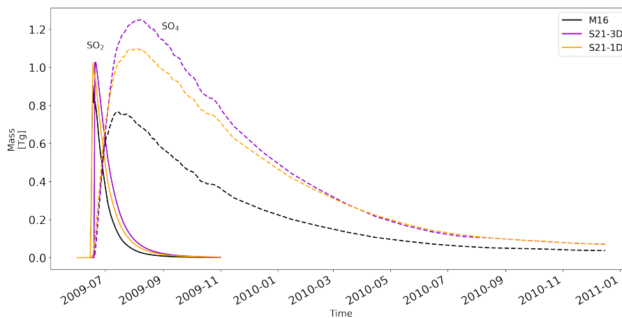
Figure 4. Stratospheric evolution of \text{SO}_2 (gas) and \text{SO}_4 (particle phase) over time. Daily values for both \text{SO}_2 and \text{SO}_4 til the end of October 2009, monthly values for \text{SO}_4 from November 2009 to December 2010. To isolate the volcanic \text{SO}_2 and \text{SO}_4 we have subtracted the \text{SO}_2 levels in the No-Volc simulation from the other 3 simulations.
