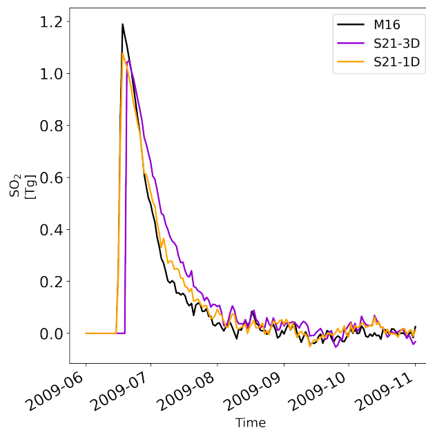
Figure 2. Global evolution of volcanic SO 2 in the M16, S21-1D and S21-3D simulations. To isolate the volcanic SO 2 we have subtracted the SO 2 levels in the No-Volc simulation from the other 3 simulations.
