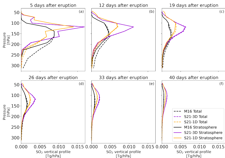
Figure 3. Vertical profile for volcanic \text{SO}_2 at 5 (a), 12 (b), 19 (c), 26 (d), 33 (e), and 40 (f) days after the volcanic eruption on the 15 of June. The dashed lines represent the total amount of \text{SO}_2 in the atmosphere whereas the solid lines represent the total amount of \text{SO}_2 in the stratosphere. To isolate the volcanic \text{SO}_2 we have subtracted the \text{SO}_2 levels in the No-Volc simulation from the other 3 simulations.
