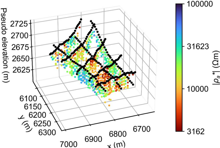
690 Figure A1: 3D visualization of the data along P1-P8 after the filtering procedure. The data are presented in terms of the apparent resistivity ( |\rho_a^*| ). Electrode positions are visualized as black dots.
