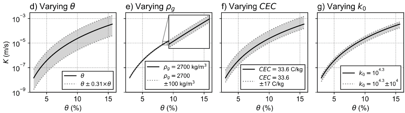
595 Figure 8: Uncertainty analysis of the hydrogeological parameters \theta (a-c) and K (d-g). The black line symbolizes \theta and K , respectively, in relation to the absolute values, while the gray area, limited by dotted lines, shows the range of \theta and K using \pm 1 standard deviation (68% confidence interval) of the parameters used in Eq. 12-14. The range of values used in a)-c) for \sigma_\infty and \theta was chosen based on the minimum and maximum of \sigma_\infty and \theta in the 4 m and 20 m depth slices (c.f., Fig. 4). While we used a constant value for the tested parameters in subplots a)-c) and e)-g), we varied \theta according to the values given in Fig. 4a,b and used a mean fractional standard deviation of 0.31, derived from error propagation for \theta .
