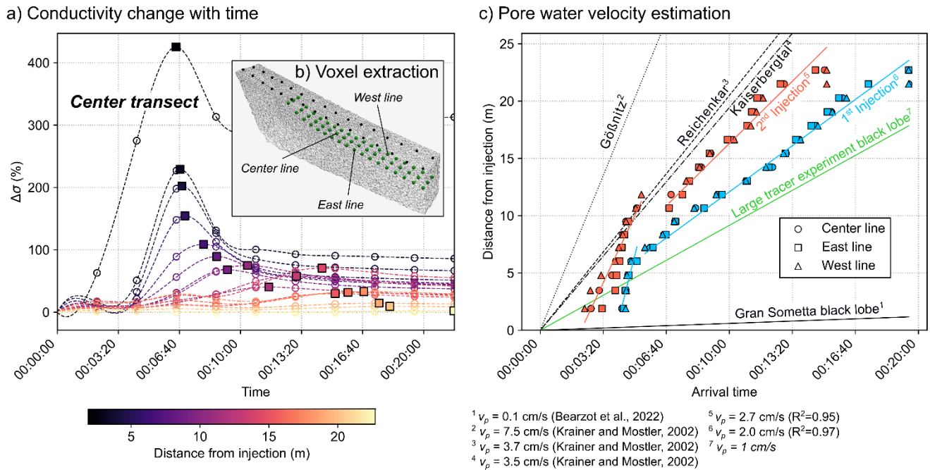
520 Figure 7: a) Change of the conductivity in % with time relative to the baseline for different voxels (positions are presented in b)) along the center line of the tracer path in the active layer during the small-scale tracer experiment in the white lobe. The distance of the voxels from the injection position is presented by the line color, the maximum change of conductivity for each voxel is visualized by a square symbol. c) shows the time of the maximum change of conductivity for each voxel in relation to the distance from the injection point. The slope of a linear regression (in blue for injection 1, in red for injection 2) gives the pore water velocity. Pore water velocities of other studies are visualized by the black lines for a comparison. The estimated pore water velocity in the large-scale tracer experiment on the black lobe is added in green.
