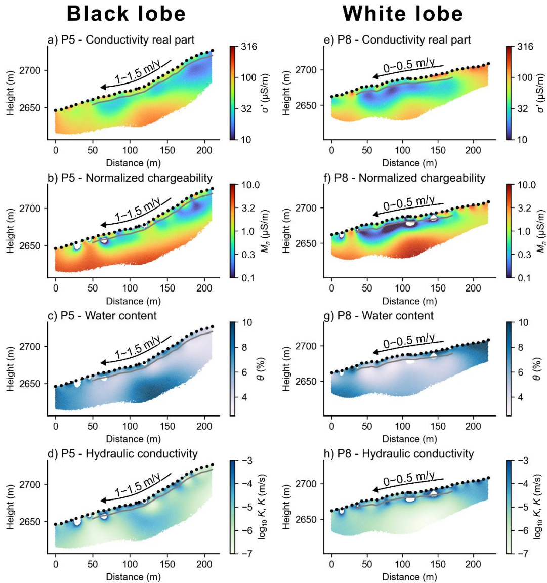
655 Figure 9: a) and e) show the real part of the complex conductivity, b) and f) the normalized chargeability, c) and g) the water content and d) and h) the hydraulic conductivity along P5 (left) and P8 (right). Pixels where the normalized chargeability results in negative values are blanked. The positions of electrodes are indicated by black dots, the interface between the active layer and the frozen layer is presented by a gray line. The rock glacier flow direction of each lobe is presented by a black arrow including its mean velocity.
