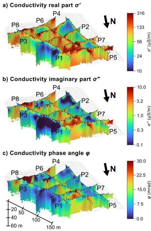
Figure 3: Slices of the 3D inverse model along the profiles at 0.5 Hz in terms of a) real part, b) imaginary part and c) phase angle of the complex conductivity. The north direction is given by a black arrow. The positions of electrodes are indicated by black dots.
