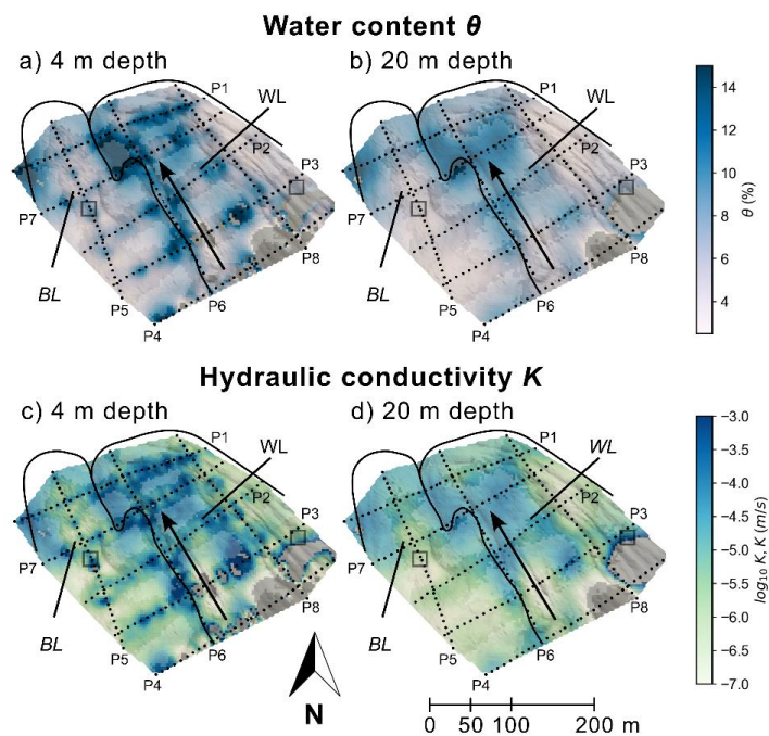
385 Figure 4: Water content (a and b) and hydraulic conductivity (c and d) visualized as slices parallel to the surface in two different depths. The edges of the black lobe (BL) and white lobe (WL) are indicated by black lines. Low sensitivity areas are displayed transparently, and the positions of electrodes are presented by black dots. Additionally, the direction of topography is indicated by a black arrow and the positions of tracer experiments by gray squares.
