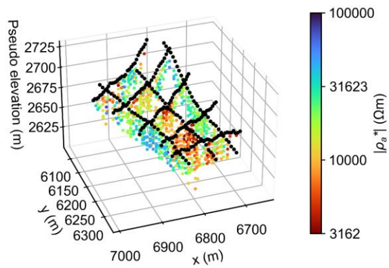
695 Figure A1: 3D visualization of the data along P1-P8 after the filtering procedure. The data are presented in terms of the apparent resistivity ( |\rho_a^*| ). Electrode positions are visualized as black dots.
