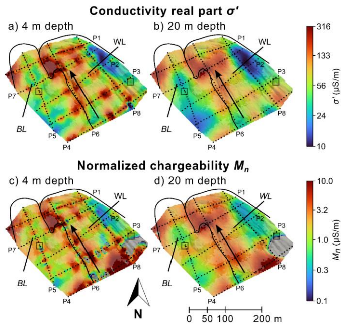
715 Figure C1: Conductivity real part (a and b) and normalized chargeability (c and d) visualized as slices parallel to the surface in two different depths. The edges of the black lobe (BL) and white lobe (WL) are indicated by black lines. Low sensitivity areas are displayed transparently, and the positions of electrodes are presented by black dots. Additionally, the direction of topography is indicated by a black arrow and the positions of tracer experiments by gray squares. The normalized chargeability refers to the difference between the bulk electrical conductivity at high 720 and low frequency (2.5 and 0.5 Hz in our study, respectively), as presented in Equation 8.
