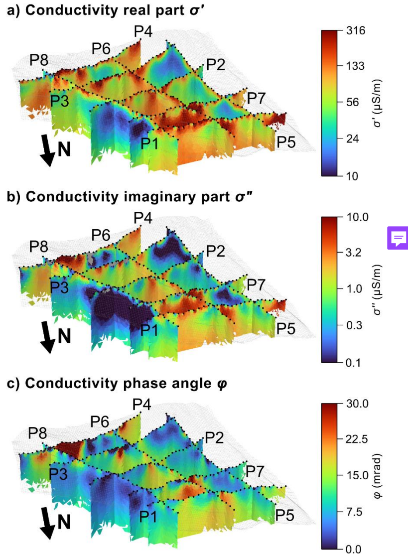
365 Figure 3: Slices of the 3D inverse model along the profiles at 0.5 Hz in terms of a) real part, b) imaginary part and c) phase angle of the complex conductivity. The north direction is given by a black arrow. The positions of electrodes are indicated by black dots.
