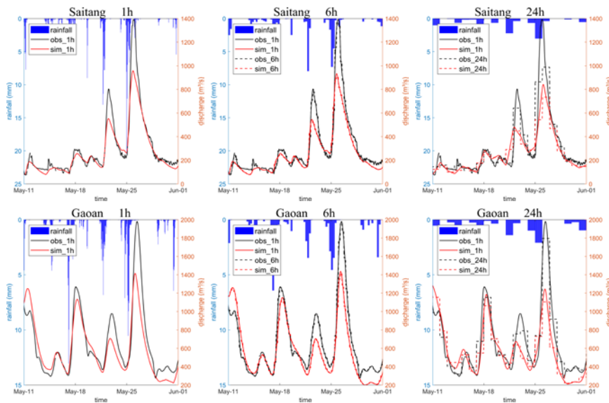
Figure 12. Hourly time series of rainfall, simulated flow, and observed flow for the representative flood events under 1h, 6h and 24h resolutions. The blue bars indicate the resampled hourly average precipitation for the catchment (used by the model during simulation). The red solid line indicates the hourly simulated flow output from the model. The red dashed line represents the simulated flow aggregated to other time resolutions (6h or 12h). The black solid line shows the actual hourly observed flow, and the black dashed line represents the observed flow aggregated to other time resolutions.
