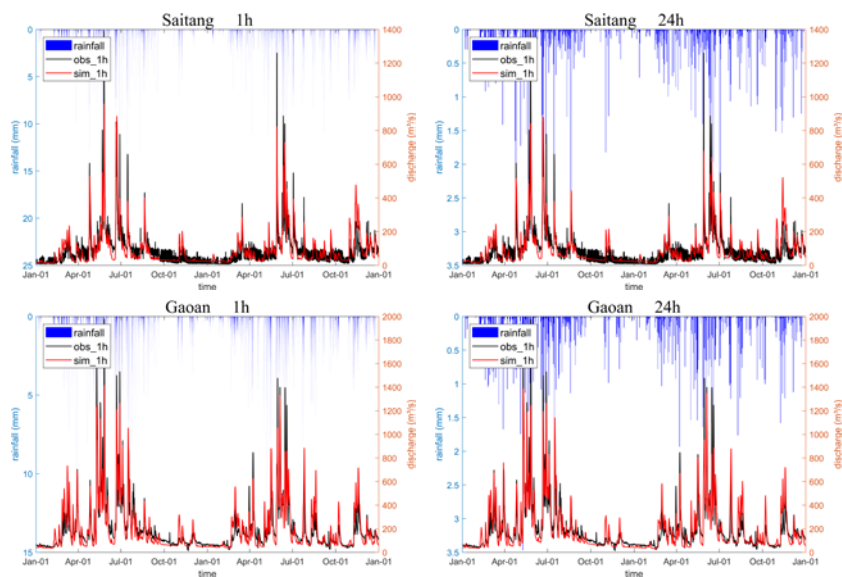
Figure 11. Hourly time series of rainfall, simulated flow, and observed flow for the representative catchments under 1-hour and 24-hour resolution data for the entire study period (2014-2015). Note that when the original data resolution is 24 hours, the rainfall is averaged and resampled to an hourly resolution.
