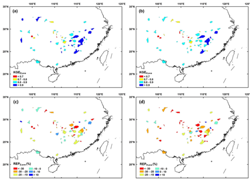
Figure 5: Spatial pattern of KGE and REP
