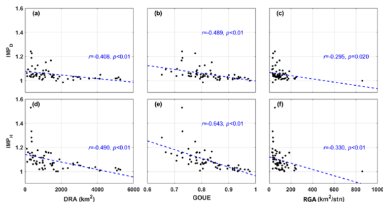
Figure 10: Scatter diagram of IMP and impact factors (DRA, GOUE, RGA)
