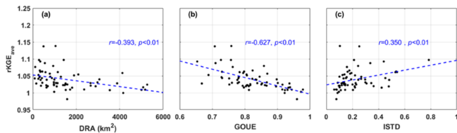
Figure 9: Scatter diagram of rKGE and DRA, GOUE, ISTD
