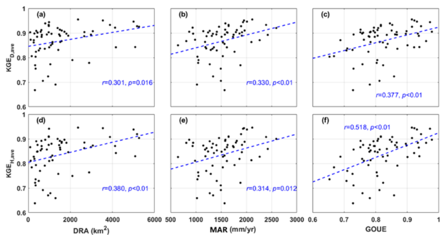
Figure 7: Scatter diagram of KGE and impact factors (DRA, MAR, GOUE)
