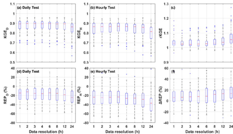
Figure 4: Box plot of KGE, REP, rKGE and \Delta REP based on experiments across 63 catchments
