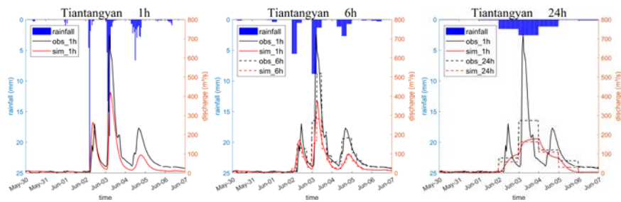
Figure 11. Hourly time series of rainfall, simulated flow, and observed flow for the representative catchments under 1-hour and 24-hour resolution data for the entire study period (2014-2015). Note that when the original data resolution is 24 hours, the rainfall is averaged and resampled to an hourly resolution.
