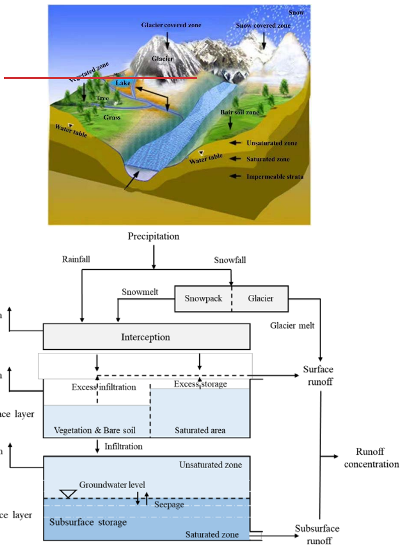
Figure 2. Structural diagram of runoff generation processes in Diagram of the THREW mModel
