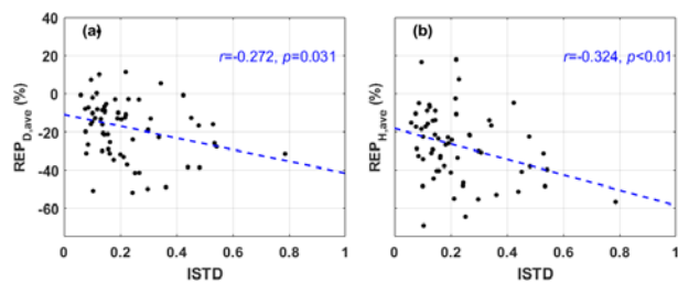
Figure 8: Scatter diagram of REP and ISTD
