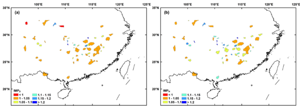
Figure 6: Spatial pattern of the benefit from higher resolution data. (a) IMP in daily test; (b) IMP in hourly test
