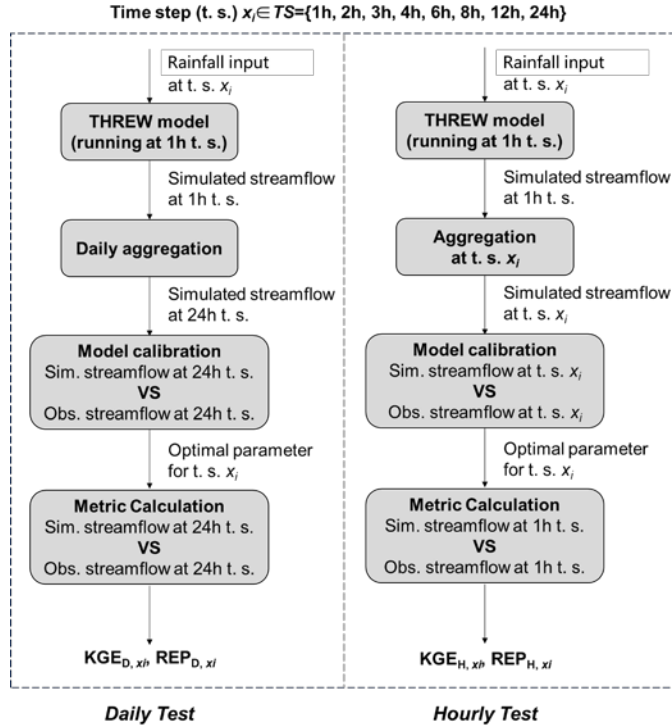
Figure 3: Flowchart of the experimental tests
