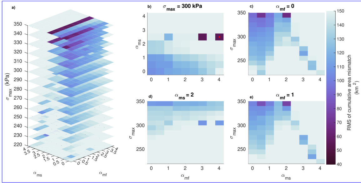
Figure 2. Parameter combination sweep of relevant melt values. Darker colors indicate a smaller RMS error of cumulative area mismatch between modeled and observational records of SK’s calving front position. Panel a displays the RMS of cumulative area mismatch for specified maximum stress levels. Panels b-d show respective RMS slices for \sigma_{\max} = 300\text{kPa} , \alpha_{mf} = 0 , \alpha_{ms} = 2 , and \alpha_{mf} = 1 . The red diamond in panel b indicates where our best-fit parameter combination lies in parameter space.
