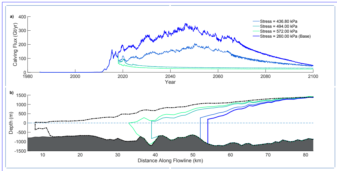
Figure 4. Top Panel (a): Calving fluxes of 2100-1985-2100 run ensemble members from 1985 to 2100 with the onset of stress amplification at 2018. Bottom Panel (b): Along flowline profiles of ensemble members at year 2030. The initial 2018 profile is denoted with a thick black dashed outline and sea level is denoted with a blue dashed line.
