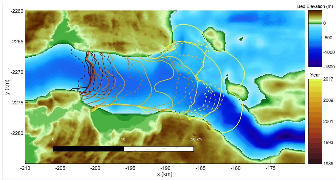
Figure 1. Observed and simulated calving fronts from our highest scoring simulation at SK from 1985-2018. The solid lines denote outputs from our best fitting ensemble member and the dashed lines indicate the observed positions of SK's calving front with the color corresponding to the year of observation.
