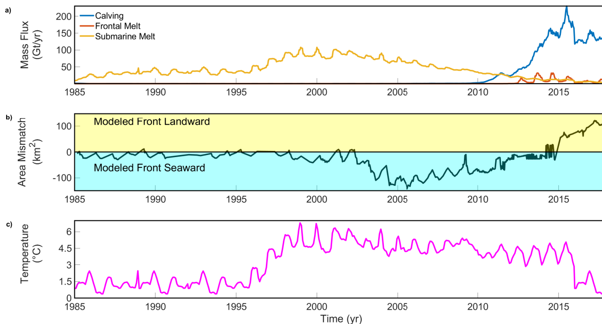
Figure 3. Best fitting model flux contribution and performance. ( Top-Panel, a) Mass flux contribution of relevant ablation mechanisms to the evolution of SK's calving front. ( Middle-Panel, b) Difference between modeled and observed calving front areas Observed area change time series vs modelled area time series . ( Bottom-Panel, c) Estimated Disko Bay fjord temperatures sourced from ECCO2 ( Menemenlis et al., 2008 ).
