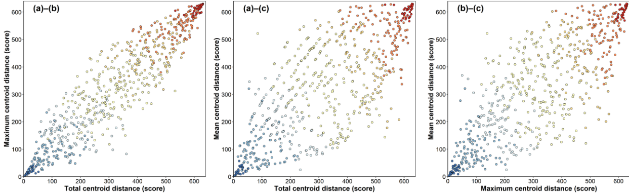
Figure 4: Relationships between three basic dynamic characteristics of global land drought events (a – total centroid distance, b – maximum centroid distance, c – mean centroid distance) according to (A) SoilClim and (B) mHM models divided into seven drought categories for 1980–2022.
