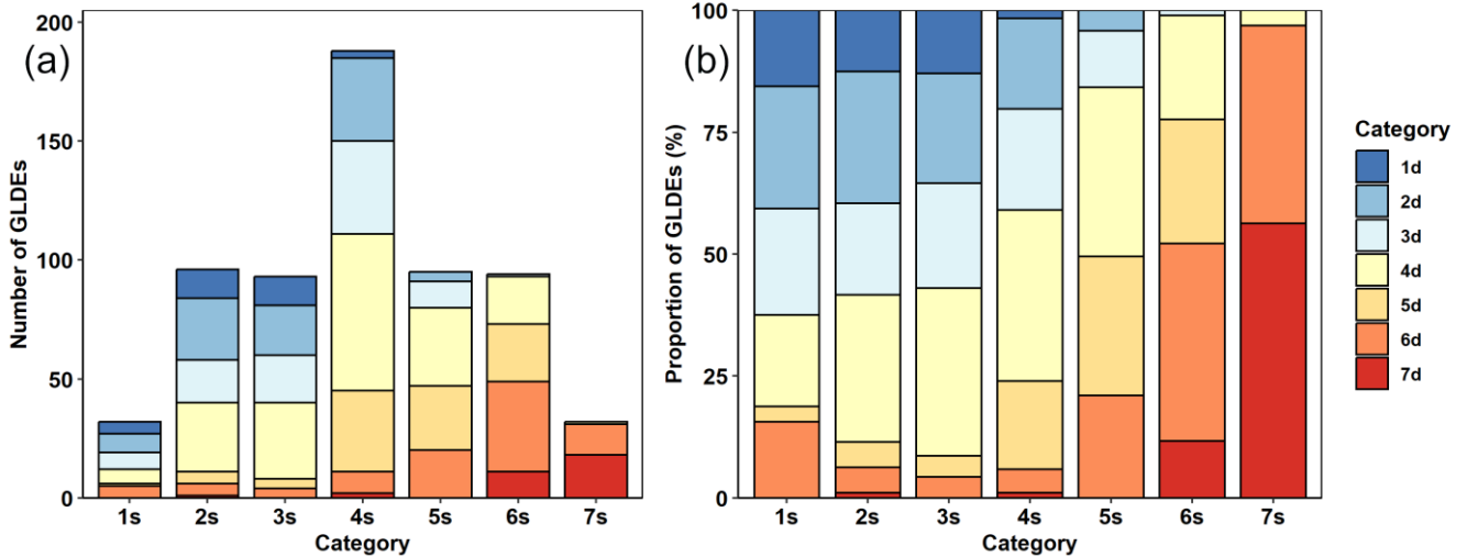
Figure 7. Comparison of global land drought events (GLDEs) from severity and dynamic classifications from 1980–2022 according to (A) the SoilClim and (B) mHM models: (a) total numbers of dynamic categories in severity categories; (b) relative proportions of dynamic categories in severity categories.
