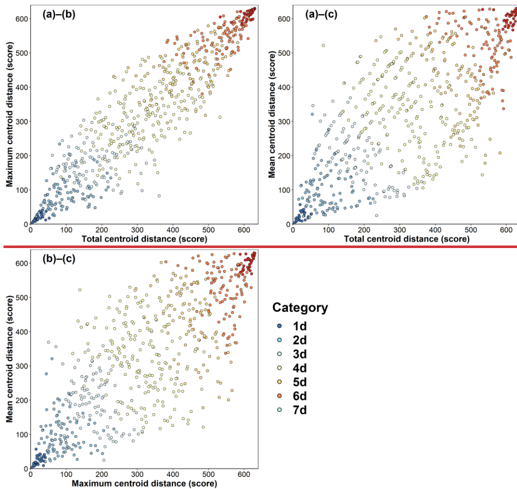
Figure 11: Relationships between the three basic dynamic characteristics of global land drought events (a—total centroid distance, b—maximum centroid distance, c—mean centroid distance) according to the mHM divided into seven drought categories for 1980–2022.
