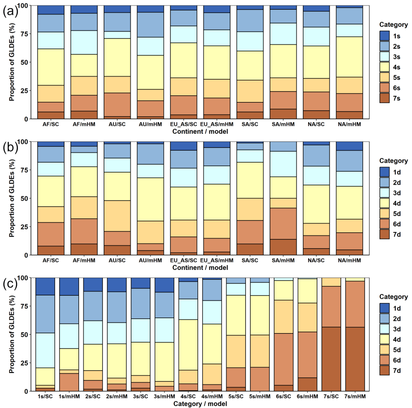
Figure 815: Comparison of the relative proportions of global land drought events (GLDEs) based on SoilClim (SC) and mHM: (a) continental proportions of the seven drought categories 1s–7s according to severity classification; (b) continental proportions of seven drought categories 1d–7d according to dynamic classification; and (c) proportions of dynamic categories 1d–7d in severity categories 1s–7s. Continents: AF – Africa, AU – Australia, EU_AS – Eurasia, SA – South America, NA – North America.
