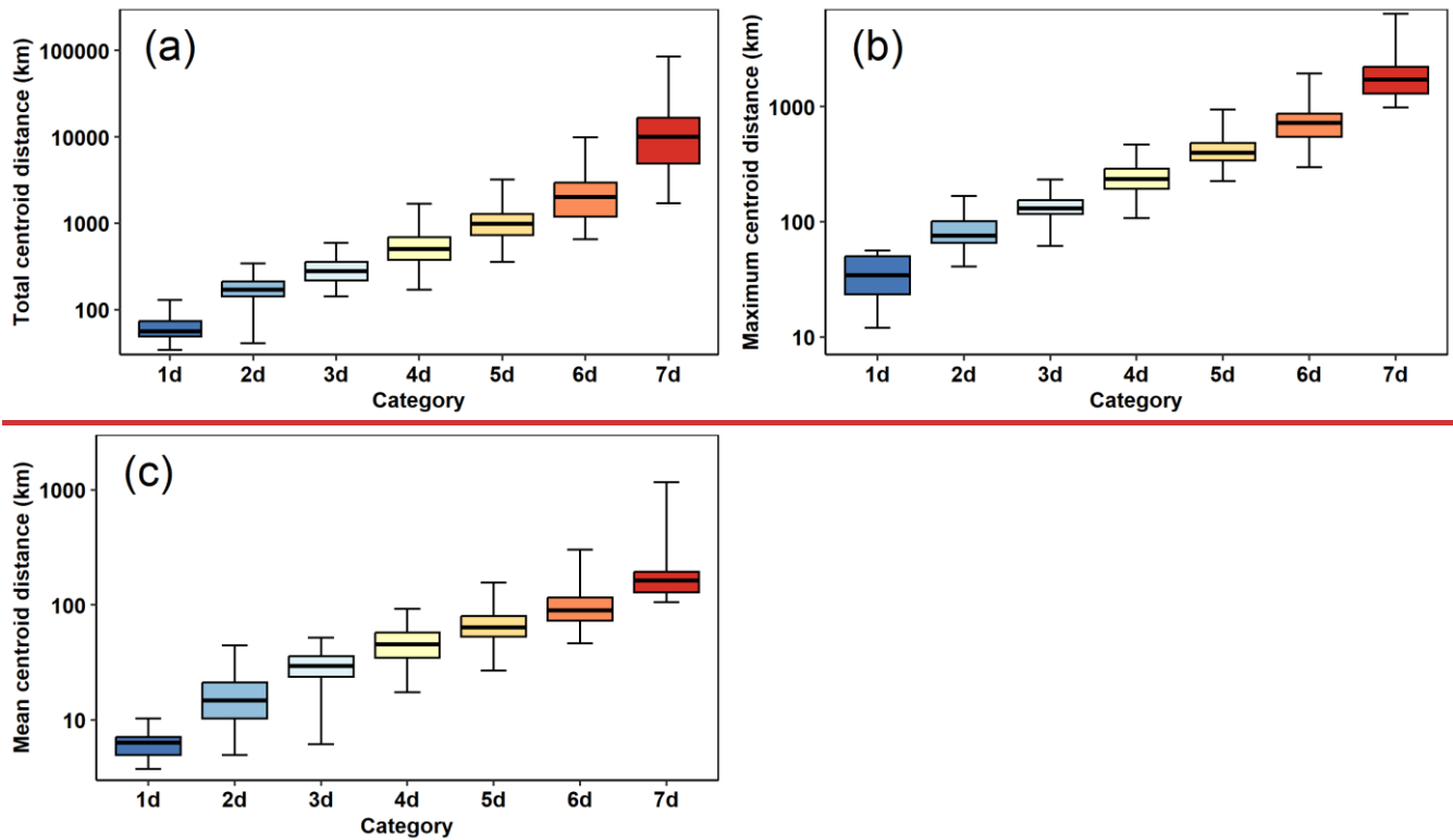
Figure 12: Box plots of the three basic dynamic characteristics of global land drought events (a—total centroid distance, b—maximum centroid distance, c—mean centroid distance) according to the mHM divided into seven drought categories for 1980–2022.
