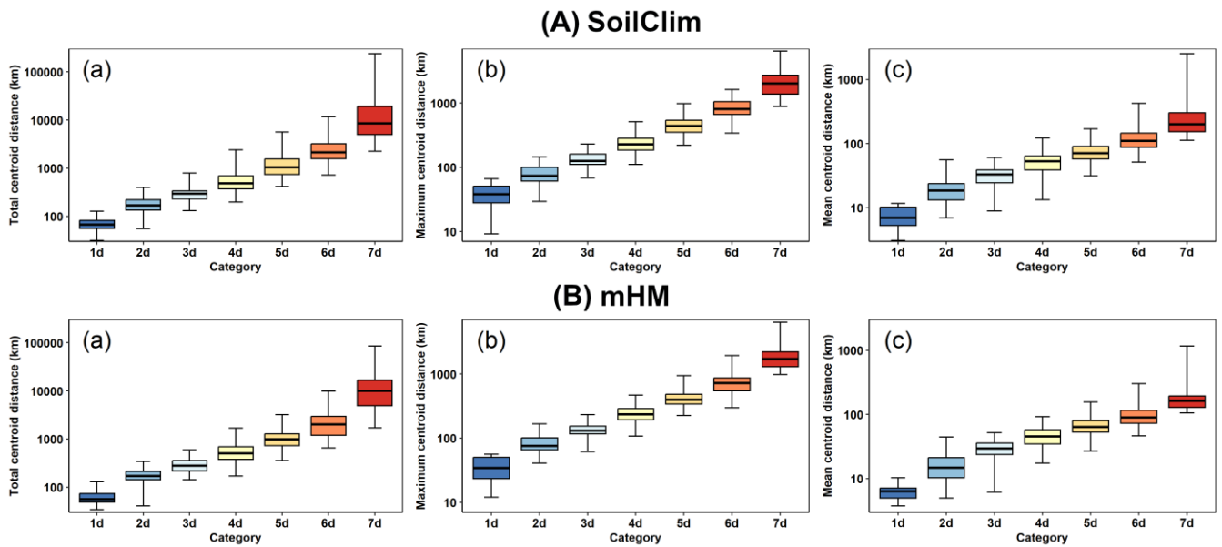
Figure 5: Box plots of the three basic dynamic characteristics of global land drought events (a – total centroid distance, b – maximum centroid distance, c – mean centroid distance) according to (A) the SoilClim and (B) mHM models divided into seven drought categories for 1980–2022.
