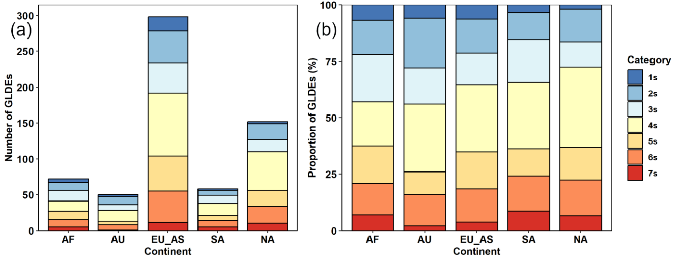
Figure 3: Continental distribution of seven drought categories from the severity classification of global land drought events (GLDEs) according to the (A) SoilClim and (B) mHM models for 1980–2022: (a) total numbers of GLDEs; (b) relative proportions of seven categories of GLDEs for a given continent. Continents: AF – Africa, AU – Australia, EU_AS – Eurasia, SA – South America, NA – North America.
