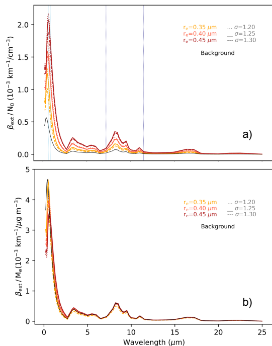
230 Figure 4: Extinction coefficient spectra \beta_{\text{ext}} at fixed number concentration N_0 (a) and effective mass M_e (b), for background (black curve) and Hunga-perturbed aerosol layers (from yellow, red and dark red dotted, dashed and solid curves – see corresponding values of the r_e and \sigma assumption in the figures captions). Light and dark blue vertical dotted lines in panel a indicate the two wavelength bands ( UV/Vis and MIR, respectively ) used to average the extinction to calculate the UV/Vis-to-MIR AE of Fig. 7.
