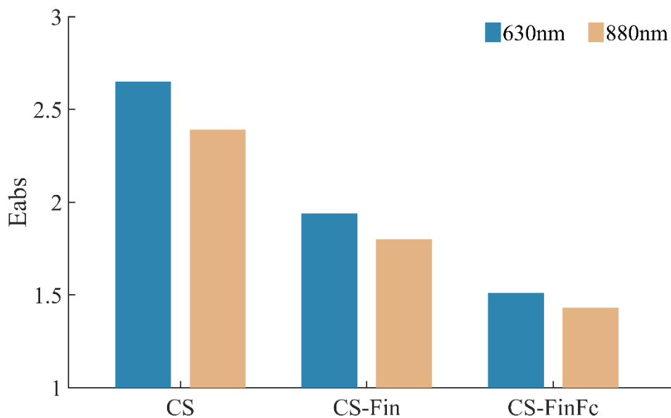
Figure 11. The radiation absorption enhancement of at 630 nm and 880 nm under different mixing state assumptions in Beijing.
