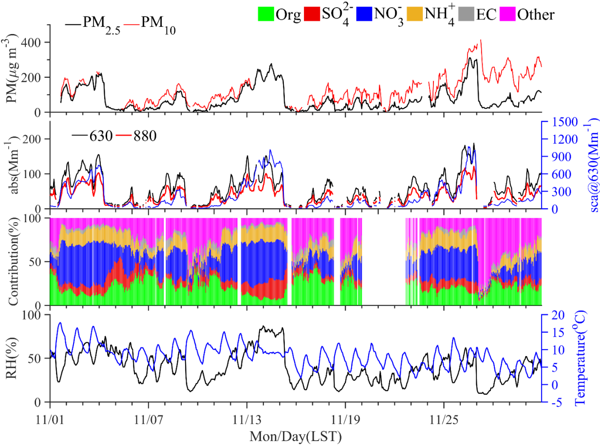
260 Figure 4. Evolution of observed PM_{2.5} , components, aerosol extinction coefficient, and meteorology parameters in November 2018 at Beijing
