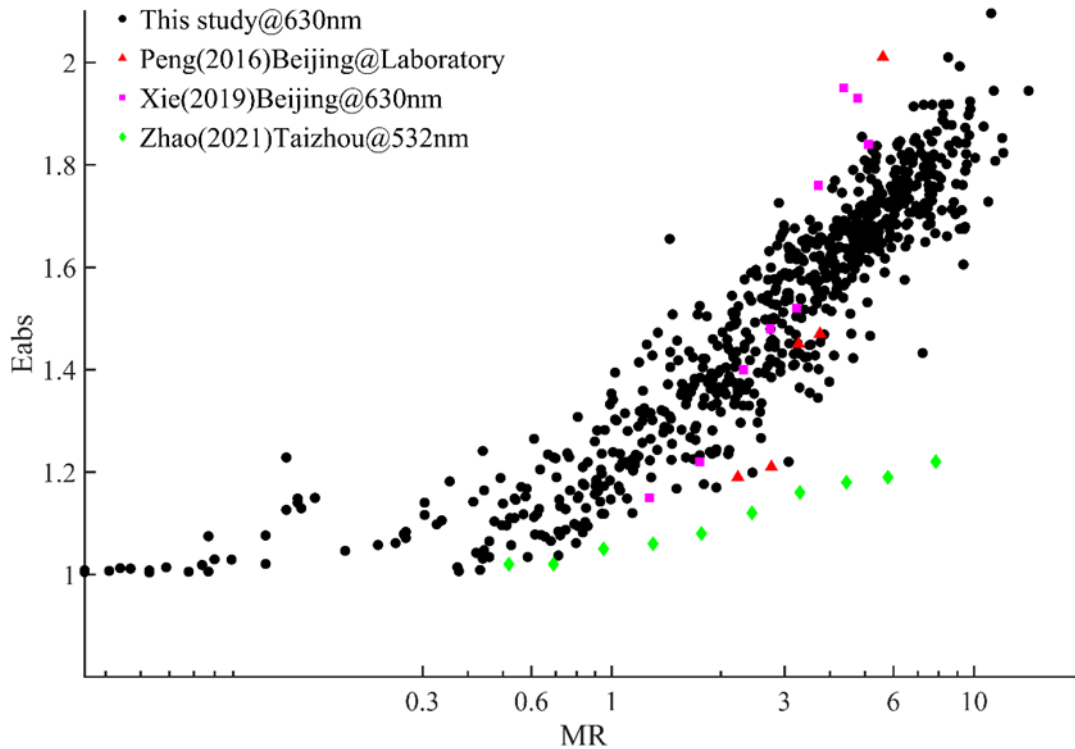
375 Figure 8. The absorption enhancement in the CS-APM case under different mass ratios (MR) of coating materials and BC core
