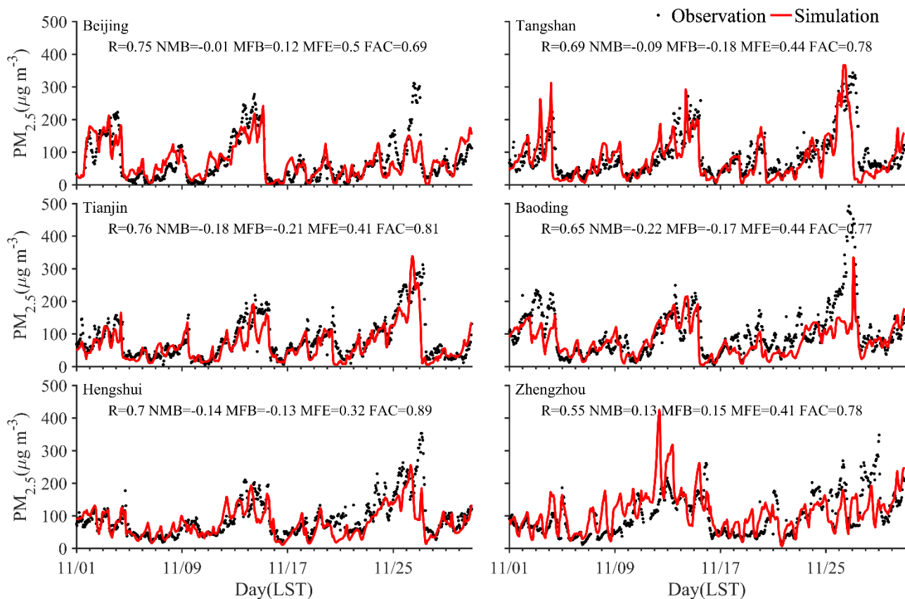
Figure 2. Model evaluation of PM 2.5 at eight-six sites in the Beijing-Tianjin-Hebei region in November 2018.
