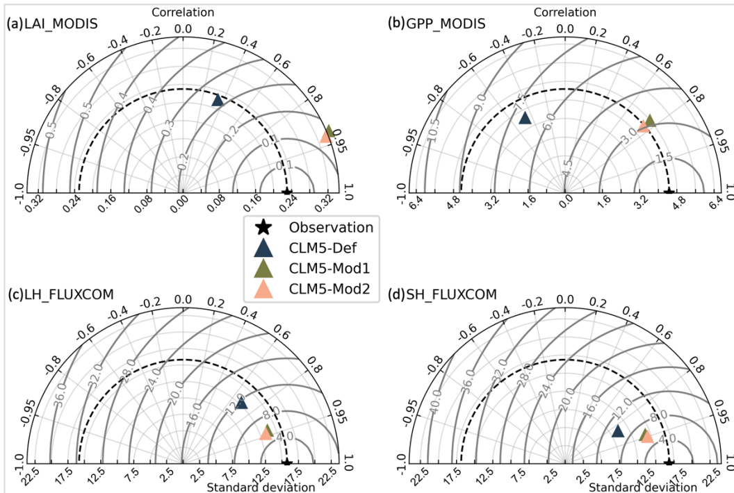
585 Figure 10: Comparing CLM5 simulated (a) LAI, (b) GPP, (c) LH, and (d) SH against observations. The data used here is the monthly mean from 2000 to 2014.
