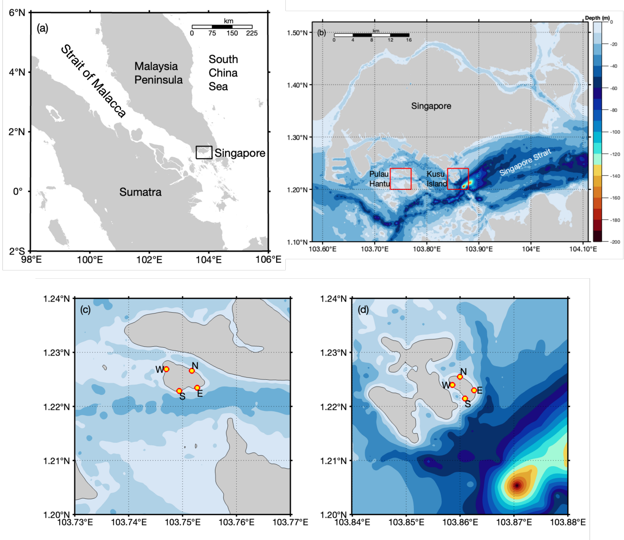
Figure 1. (a) A map of the Southeast Asia region with Singapore indicated by the black rectangle. (b) A zoomed-in map of Singapore with the location of our study areas, Pulau Hantu and Kusu Island, in the southern coast of Singapore (indicated by the red rectangles). The background colour represents the bathymetry. (c) A zoomed-in map of Pulau Hantu with the four
