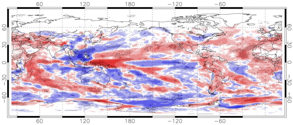
SW TOA flux [ \text{W m}^{-2} ] SHIP20-SHIP100 2020-2049 jja (0.20)
