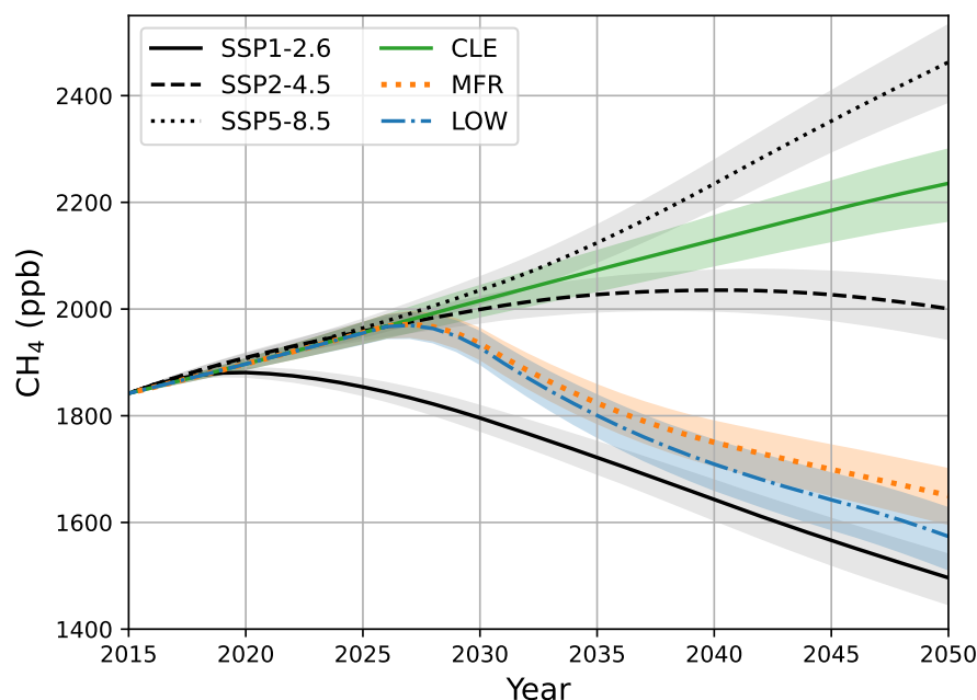
Figure 1. Projected background \text{CH}_4 concentrations up to 2050 for the CLE, MFR, and LOW scenarios described in the text. Projections for the SSP5-8.5, SSP2-4.5, and SSP1-2.6 scenarios are included for reference. The shaded area represents the 600-ensemble 5-95% range.
