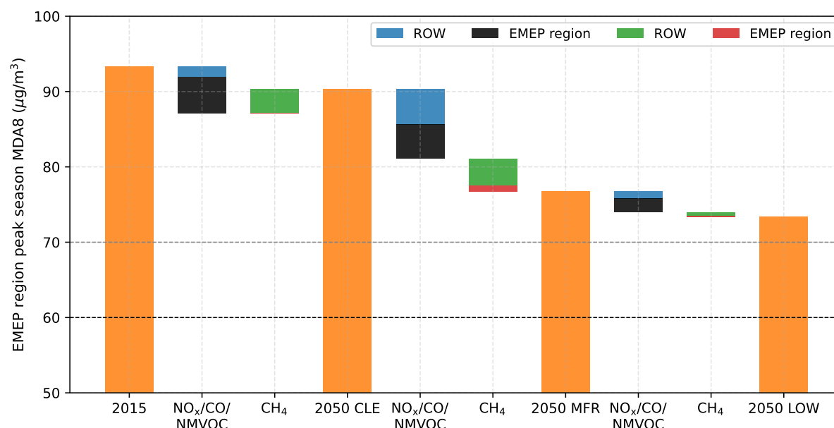
Figure 3. Cascade plot of the population weighted EMEP region average peak season MDA8 scenario changes arising from NO x , CO, and NMVOC emission changes within the EMEP (black) and ROW (blue) regions, and from background CH 4 changes arising from EMEP (red) and ROW (green) region emission changes. The black and grey dashed horizontal line denote guideline and interim WHO target values, respectively. Note that the y-axis starts at 50 μg m -3 .
