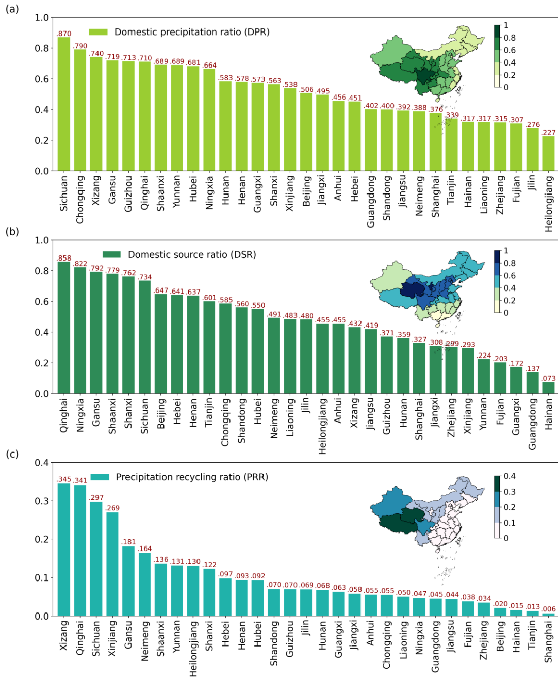
Figure A3. Domestic precipitation ratio (a), domestic source ratio (b) and precipitation recycling ratio (c) in each province.
