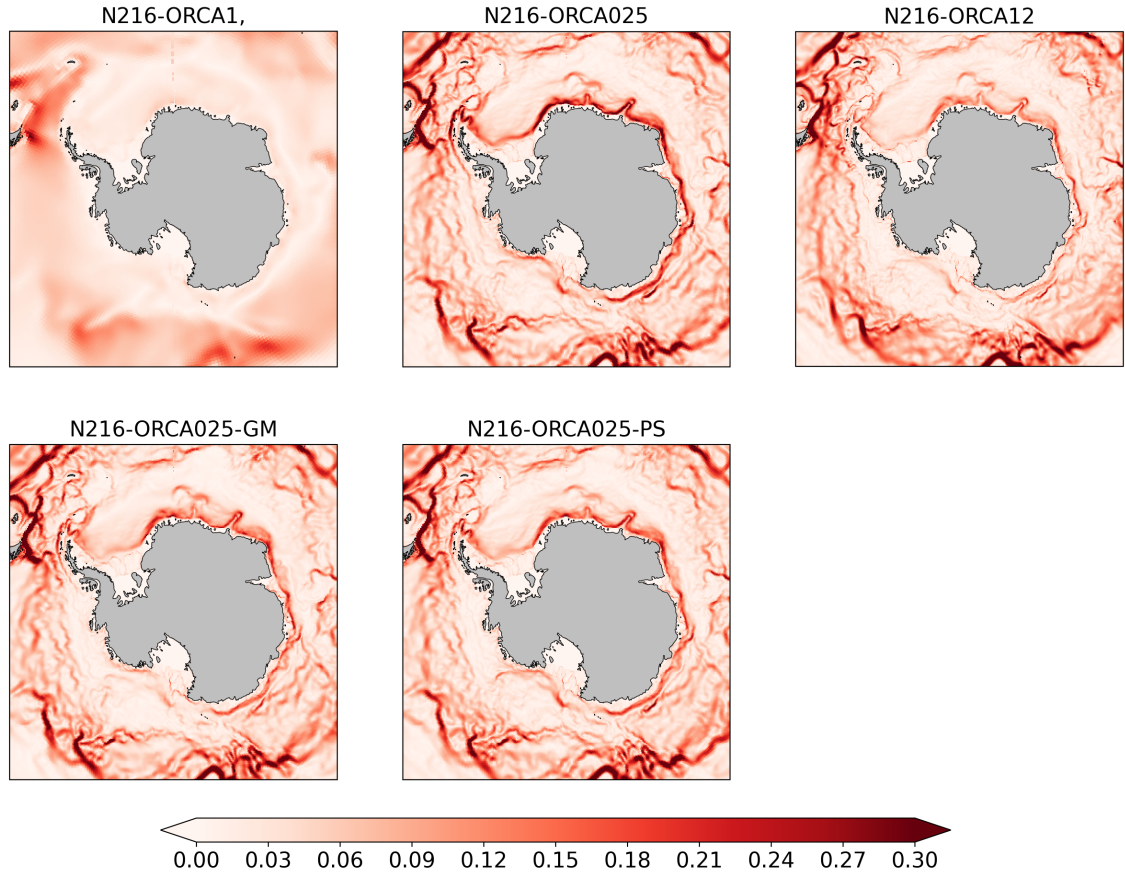
Figure 2. Depth-mean current speeds (m/s) over the top 500m, time mean for the third decade of the spin up. The experiment labels are defined in Table 2. The eddy models show a strong westward flowing slope current, which in the eddy-permitting model is fully circumpolar, including flow at the southern boundary of the Drake Passage and in the Bellingshausen and Amundsen Seas. Note in the region of the gyres the flow along the slope is a combination of the recirculating flow in the gyres and the throughflow.
