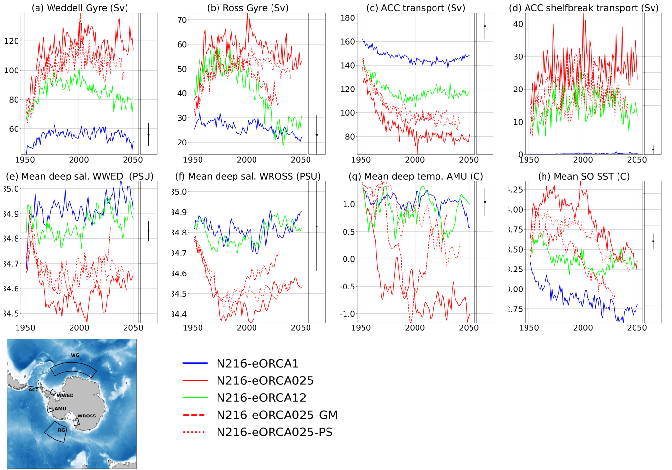
Figure 7. Timeseries of Southern Ocean metrics for the first 150 100 years of the HiResMIP HighResMIP integrations. Experiment labels are defined in Table 2. The plotted quantities are annual means apart from the WWED metric where summertime (DJF) means are used to better match the available observations (see Appendix A). Observational estimates and uncertainties are plotted as the black dots and lines to the right of the timeseries plots. From top left: a) The transport of the Weddell gyre plus ASC as indicated by the maximum streamfunction in the WG box, compared to the estimate of Klatt et al. (2005); b) The transport of the Ross gyre plus ASC as indicated by the maximum streamfunction in the RG box, compared to the estimate of Dotto et al. (2018); c) The net eastward transport in the Drake Passage compared to the estimate of Donohue et al. (2016); d) The total westward transport in the Drake Passage south of 62S compared to the estimate of Meijers et al. (2016) e) The salinity below 400m spatially averaged over the WWED box in the western Weddell Sea; e f ) The salinity below 400m averaged over the WROSS box in the western Ross Sea; f g ) The temperature below 400m averaged over the AMU box in the Amundsen Sea; The deep temperatures and salinities are compared against time and spatial means of profiles from the EN4.2.2.g10 dataset (Good et al., 2013) as described in Appendix A ; g h ) The SST averaged between 45S and 70S compared to the 1950-1954 climatology of the EN4.1.1.g10 analysis (Good et al., 2013) averaged over the same region.
