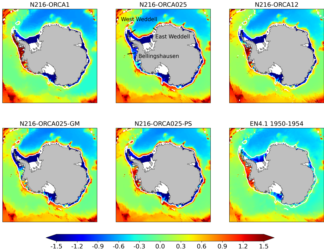
Figure 5. Bottom potential temperature ( ^{\circ}\text{C} ), time mean for the third decade of the spin up. The experiment labels are defined in Table 4. The 1000m depth contour is shown in white. Bottom temperatures from a 1950-1954 climatology of the EN4.1 reanalysis (Good et al., 2013) are shown in the bottom right figure. The top middle figure shows the approximate locations of the sections described in Thompson et al. (2018) and plotted in Figure 8.
