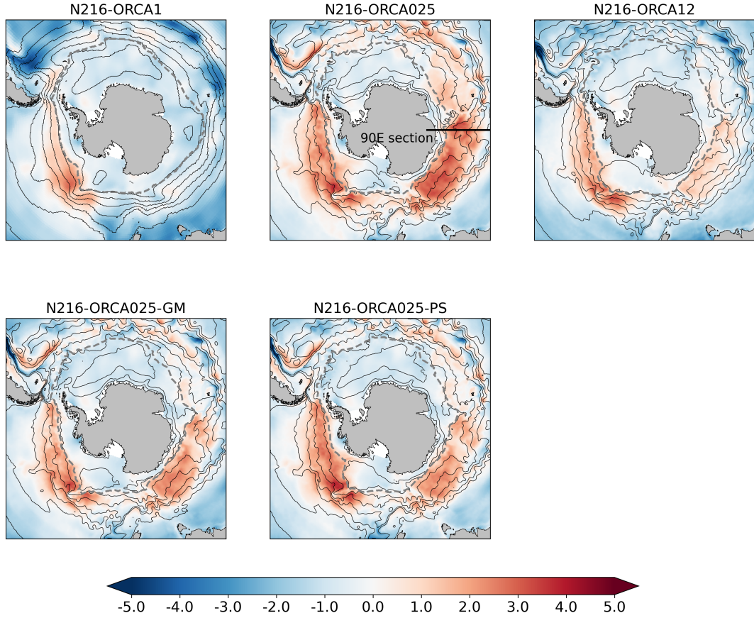
Figure 6. SST anomalies against ESA-CCI-SST (colours) and mean SSH (thin black lines) to show the positions of the gyres and the ACC; and the mean September ice extent indicated by the contour of 15% ice concentration (thick dashed grey line). The experiment labels are defined in Table 1-2. Time mean means for the third decade of the spin up. The line in the top middle plot shows the location of the 90E section displayed in Figure ??9.
