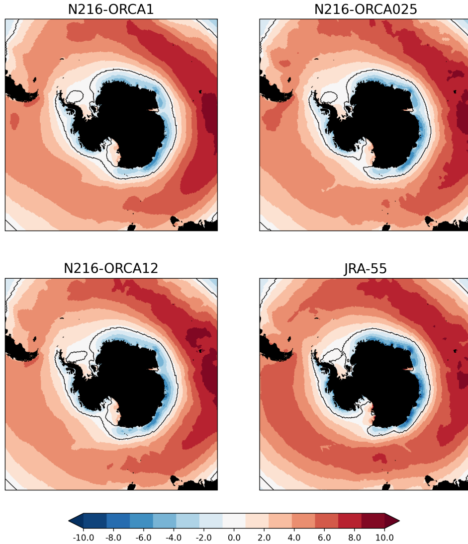
Figure 10. Zonal winds (m/s) at 10m for the JRA-55 reanalysis and the three control integrations and the JRA-55 reanalysis (Kobayashi et al., 2015). The black lines show the contour of zero zonal wind component. The fields are 10-year means for the third decade for the model integrations and means over an equivalent period (1970-1979) for JRA-55.
