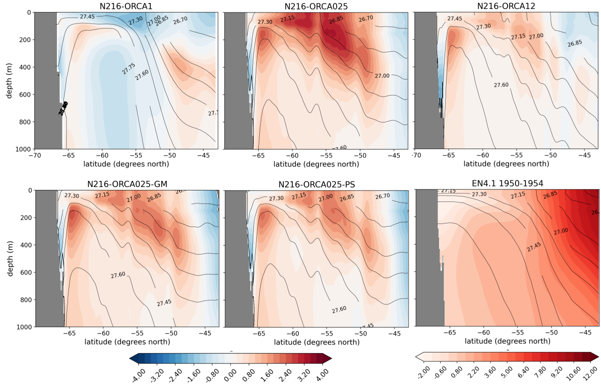
Figure 9. Section at 90E-90°E (marked in Figure ??6) showing temperature anomalies against EN4.1 (colours) and potential density ( \sigma_0 - lines) for the various integrations, and potential temperature and potential density for the EN4.1 climatology. Model fields are time means for the third decade of the integration.
