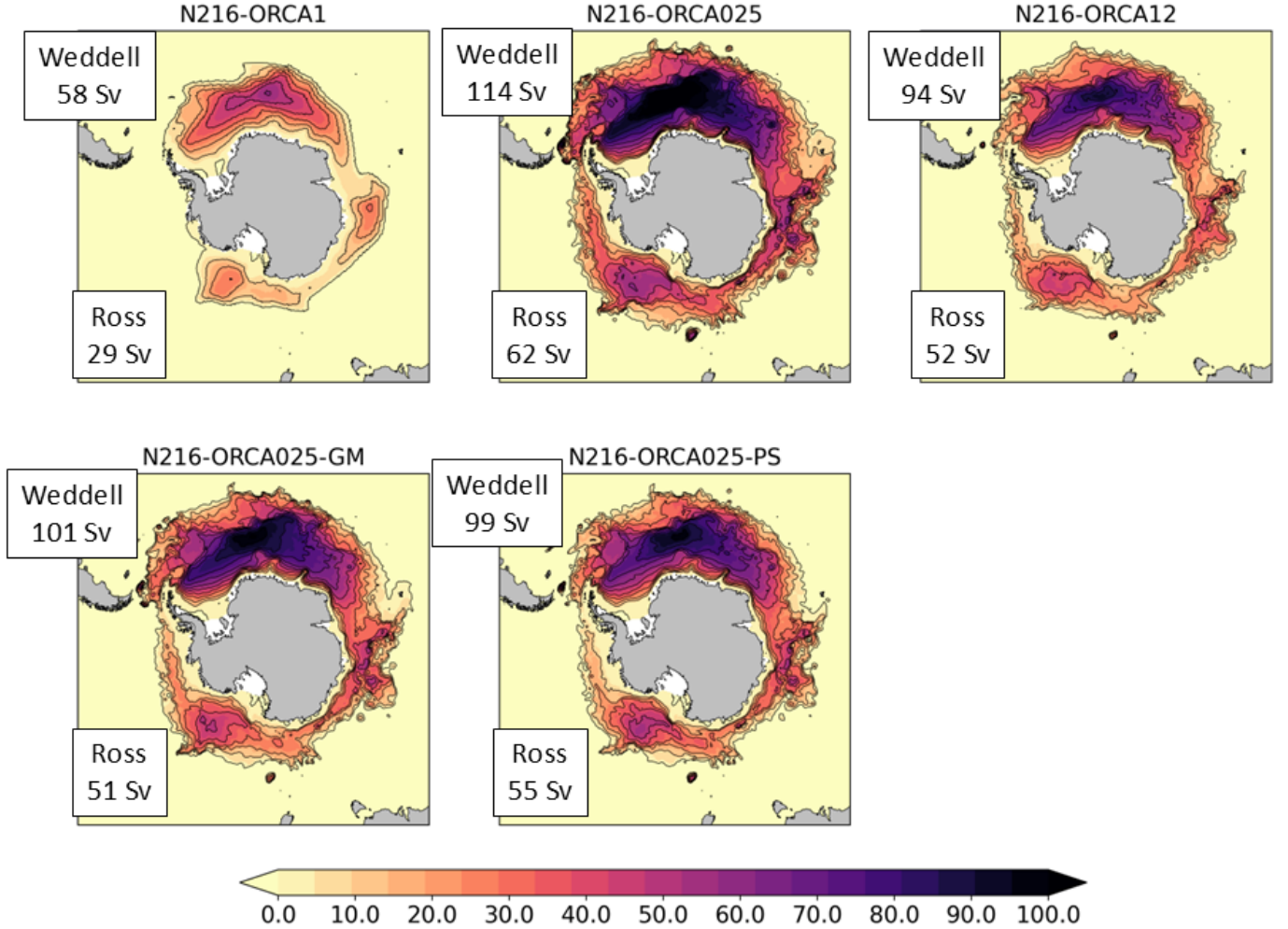
Figure 1. The barotropic streamfunction (Sv), time mean for the third decade of the spin up. The experiment labels are defined in Table 4-2. The integration of the velocity field is done from the south northwards and only positive streamfunction values are plotted, highlighting the subpolar gyres south of the main ACC fronts. The spatial peak of the time-mean streamfunction values for the gyres in the Weddell Sea and Ross Sea are marked. By construction this includes the transport of the southern limb of the recirculating gyre plus the transport of the ASC. These numbers can be compared to the observational estimates of 56 \pm 8 Sv (Klatt et al., 2005) for the Weddell gyre, and 29 \pm 8 Sv (Dotto et al., 2018) for the Ross gyre.
