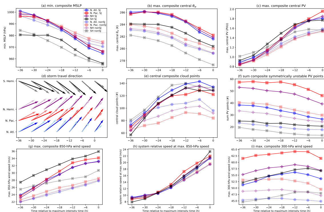
Figure 12. Time series of composite field statistics: (a) minimum MSLP, (b) maximum \theta_w within 300 km of the composite MSLP centre, (c) maximum 700-hPa PV within 300 km of the composite MSLP centre (minimum value for Southern Hemisphere), (d) storm travel direction, (e) number of cloudy points (700-hPa relative humidity with respect to ice >80\% ) within 600 km of the composite MSLP centre, (f) total number of composite mean points with symmetrically unstable 700-hPa PV (negative and positive PV for Northern and Southern Hemisphere, respectively), (g) maximum 850-hPa wind speed, (h) 850-hPa system-relative wind speed at the location of the maximum 850-hPa (Earth-relative) wind speed, and maximum 300-hPa wind speed. In (d) the dark and pale arrows are for the sting-jet and non-sting-jet cyclones, respectively; in all other panels the solid and dotted lines are for the sting-jet and non-sting-jet cyclones, respectively.
