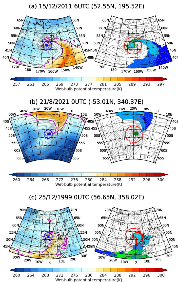
Figure 1. Examples of maps used for evaluation of the warm-seclusion identification algorithm. Left-hand-side maps include MSLP (grey contours, hPa), 850-hPa \theta_w (shading, every 1 K) with warm-sector areas (see definition in the text) highlighted by thick magenta contour. The blue circle (cyclone pressure core) has a radius of 300 km and is centred over the cyclone centre. The blue-shaded region covers the cyclone pressure core. Right-hand-side maps include MSLP (grey contours, hPa) and all warm-sector watersheds identified by the algorithm (discrete colours). The thick green or red contour highlights the watershed that overlaps the pressure core with the most points and its colour depends on whether the cyclone is identified as having a warm seclusion (green) or not (red). The red circle for warm-seclusion identification has a radius of 600 km and is centred over cyclone centre.
