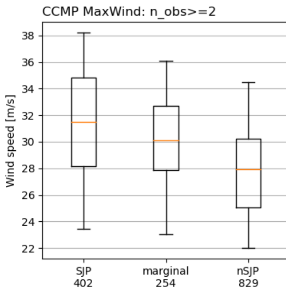
Figure 13. Maximum CCMP3.0 wind speeds within a 10^\circ box of each cyclone centre at the time of maximum intensity. All cyclones from the CCMP3.0 period (1993–2019) that have at least two independent scatterometer observations contributing to the blended wind speed product at the grid point of the maximum are included.
