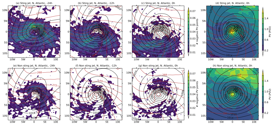
Figure 11. Maps of the composite 700-hPa PV structure of the SJP (top row) and nSJP (bottom row) cyclones for the North Atlantic. In (a–c,e–g) shading is the composite number of negative (symmetrically unstable) PV points at (a,e) 24, (b,f) 12 and (c,g) 0 h prior to the time of maximum intensity; in (d,h) shading is the composite PV at the time of maximum intensity. All other fields as in the top row of Fig. 9.
