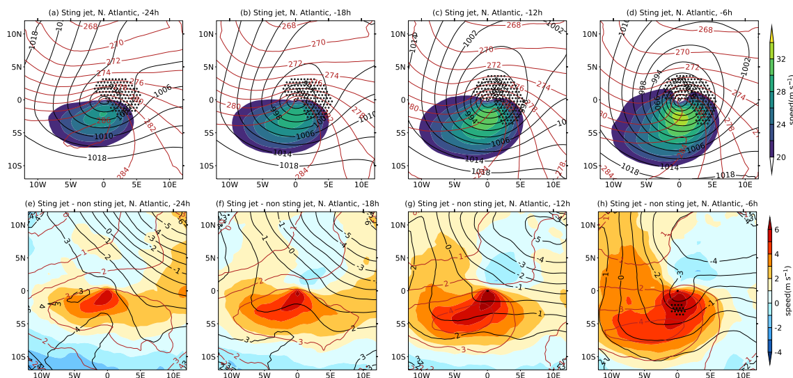
Figure 9. Maps of the low-level composite structure of the SJP cyclones (top row) and their differences to the nSJP cyclones (bottom row) for the North Atlantic at (a,e) 24, (b,f) 18, (c,g) 12, and (d,h) 6 h prior to the time of maximum intensity. Fields shown as in Fig. 8.
