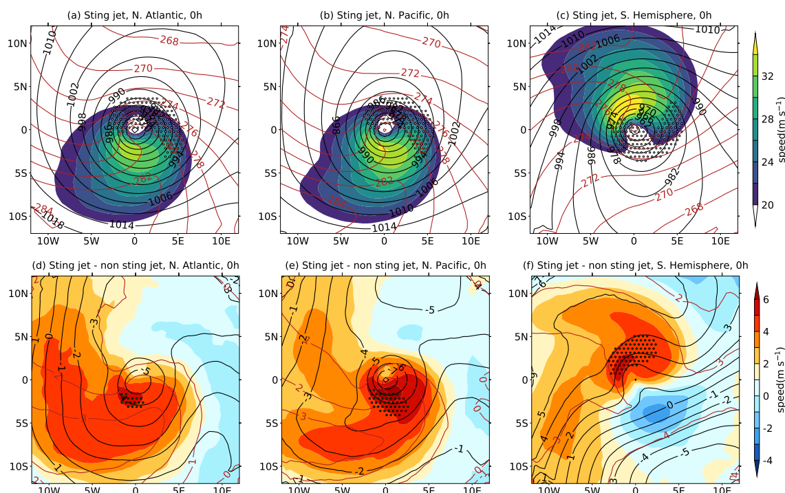
Figure 8. Maps of the low-level composite structure of the SJP cyclones (top row) and their differences to the nSJP cyclones (bottom row) at the time of maximum intensity for the (a,d) North Atlantic, (b,e) North Pacific, and (c,f) Southern Hemisphere: (top row) 850-hPa wind speed (shaded), MSLP (black contours), 850-hPa \theta_w (brown contours) and 700-hPa cloud (stippling indicates relative humidity with respect to ice >80%); (bottom row) difference fields for wind speed (shaded), MSLP (black contours) and 850-hPa \theta_w (brown contours) with green stippling marking the region of winds exceeding 32 m s -1 in the equivalent SJP composites.
