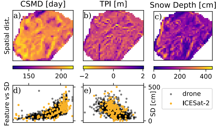
Figure 3. Panels a) and b): spatial distribution of the feature dimensions Climatology of Snow Melt-out Date (CSMD) and Topographical Position index (TPI) in the Izas experimental catchment. Panel c): spatial distribution of snow depth derived from the drone map of the 3 rd of February. Panels d) and e): the dimension's relation with snow depth from the drone map acquired on the 3 rd of February (black) and with ICESat-2 for the observed profiles on the 5 th of February (yellow).
