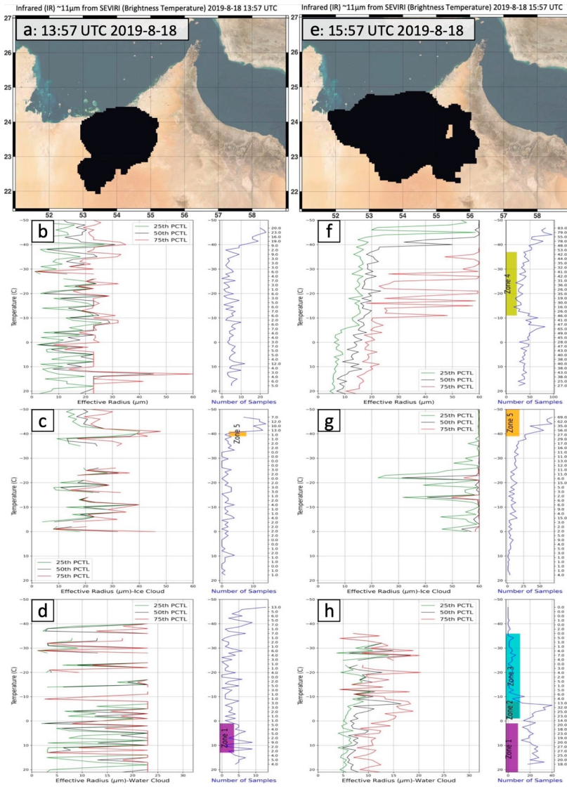
Figure 10. The detected zones in one cloud patch on August 18 th , 2019. (a) The object of a cloud patch at 13:57 UTC. (b)-(d) The effective radius (left) and the number of data samples (right) for the total, ice, and water cloud phases, respectively. (e)-(h) are the same as (a)-(d) but for the same cloud patch at 15:57 UTC.
