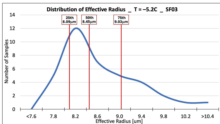
1240 Figure S3: The number of samples distribution of cloud particle effective radius for one cloud penetration at temperature -5.2°C from flight SF03. The three red vertical bars from left to right indicate the 25 th , 50 th , and 75 th percentiles of the effective radius.
