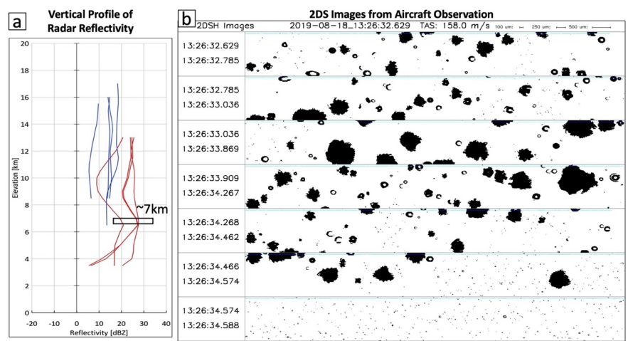
1230 Figure S1. (a) The vertical profiles of radar reflectivity for cloud penetrations in SF03 from the C-band weather radar at Al Ain. (b) The 2-DS image from the aircraft observation at about 7 km elevation.
