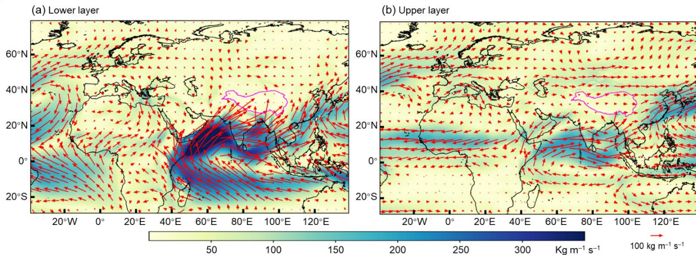
230 Figure 6: Average moisture transport fluxes ( \text{kg m}^{-1} \text{s}^{-1} ) in the (a) lower and (b) upper layers in WAM2layers during the entire simulation period (June–July 2022).
