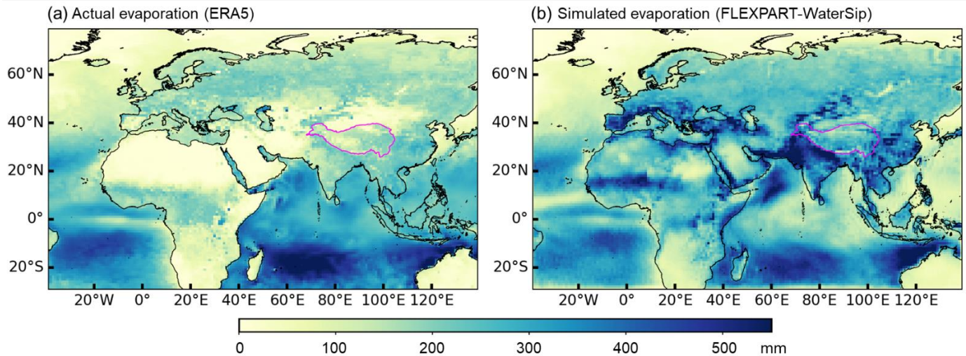
Figure 8: (a) Evaporation from ERA5 and (b) simulated evaporation from FLEXPART-WaterSip during June–July 2022.
