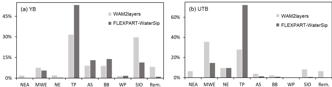
220 Figure 5: Relative moisture contributions (%) to precipitation in July 2022 over the (a) YB and (b) UTB from the eight selected source regions (NEA, MWE, NE, TP, AS, BB, WP, and SIO) and the remaining (Rem.) source regions simulated by WAM2layers and FLEXPART-WaterSip models.
