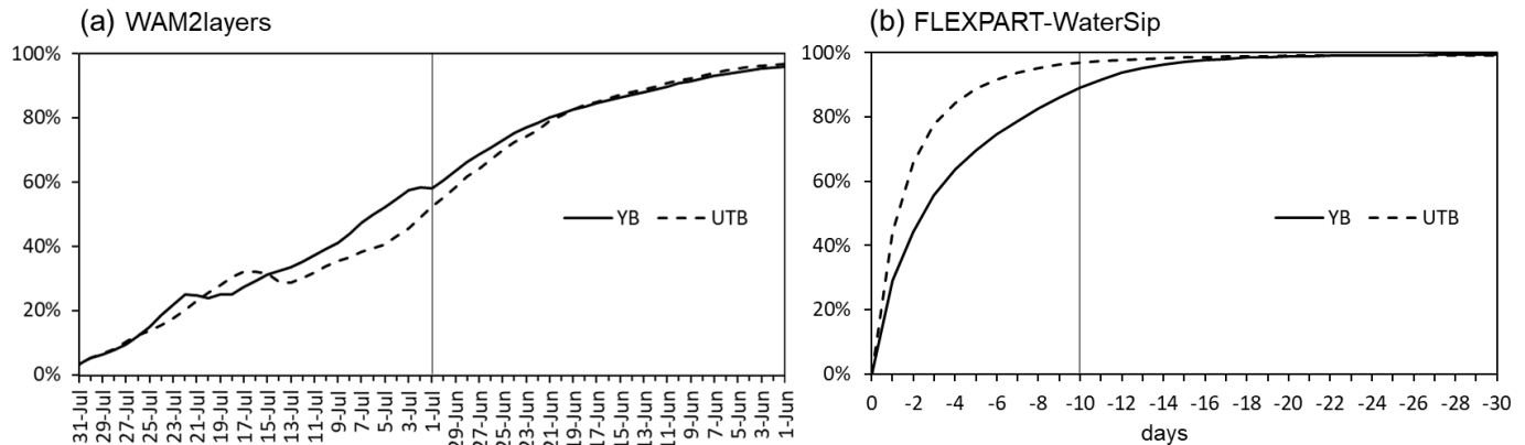
Figure 2. Backward moisture tracking periods and accumulated moisture uptake from all source regions in (a) WAM2layers and (b) FLEXPART-WaterSip models. Solid lines represent the YB, and dotted lines represent the UTB.
