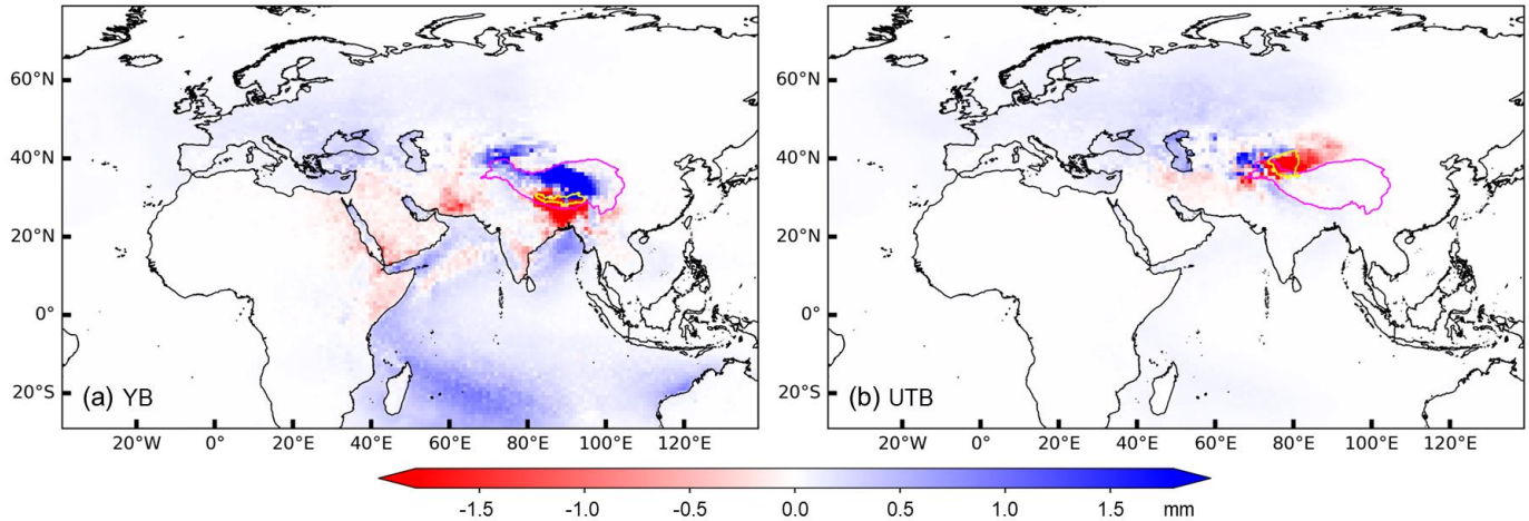
Figure 4: Absolute differences in moisture contributions to precipitation in July 2022 between WAM2layers and FLEXPART-WaterSip (WAM2layers minus FLEXPART-WaterSip) for the (a) YB and (b) UTB simulations.
