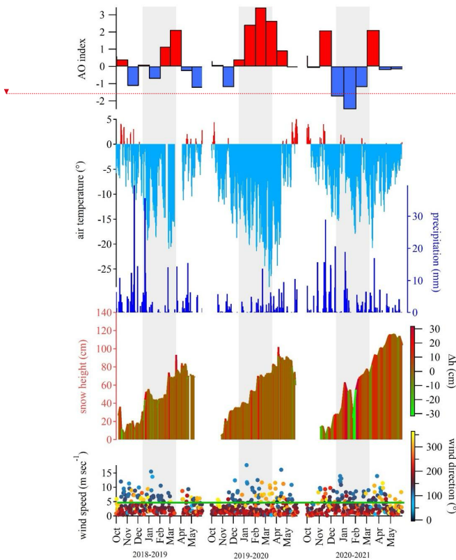
Fig. 2. AO Index, air temperature (°C), precipitation (mm), snow height (cm), \Delta h snow height (cm), wind speed (m sec -1 ), and wind direction (°) from the NCEP/NCAR Reanalysis data. The green horizontal line above the wind speed graph indicates the 5 m sec -1 threshold, above which wind drift may occur on surface snow layers. The colour of the line refers to the \Delta h color scale, which indicates negative values of \Delta h , NOAA Physical Sciences Lab's daily composites tool was used to calculate the near-surface air temperatures across the Northern Hemisphere from October to May. Grey bands indicate the winter periods.
