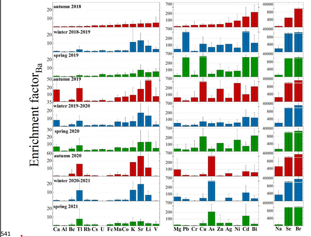
Fig. 4. Enrichment Factors (EFs) calculated on all the presented trace elements for the three sampling campaigns: 2018-19, 2019-20, 2020-21. Calculating EFs for the full dataset offers a more robust assessment of potential sources and enrichment patterns, minimizing the variability inherent in individual seasons and allowing for a clearer distinction between crustal and non-crustal contributions.
