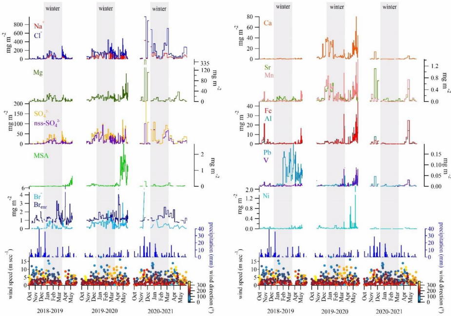
Fig. 3. Wind direction (°), wind speed (m sec -1 ), and ionic loads (mg m -2 ) of Na + , Cl - , Mg, SO 4 2- , nss-SO 4 2- , MSA, Br - , Ca, Sr, Mn, Fe, Al, Pb, V, Ni in the surface snow for the three sampling campaigns: 2018-19, 2019-20, 2020-21. Seasonal trends are here presented for specific elements to provide a detailed view of how concentrations vary across distinct sampling periods.
