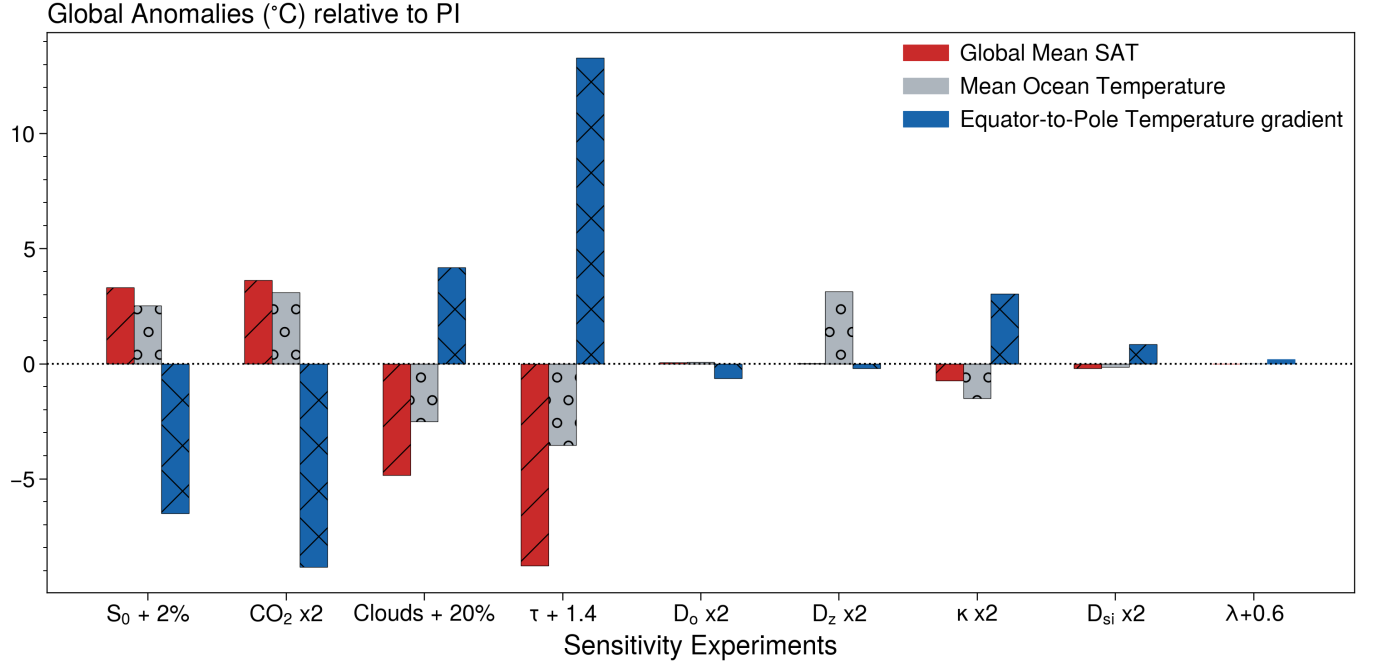
Figure A2. Anomalies in global mean surface air temperature, global mean ocean temperature and the air temperature difference between the equatorial ( 0^\circ - 10^\circ ) and polar regions ( 80^\circ - 90^\circ ) for changes in the solar constant ( S_0 ), atmospheric CO_2 level ( CO_2 ), cloud amount, cloud optical depth ( \tau ), ocean diffusion coefficient for horizontal eddy/gyre heat transport ( D_o ), ocean diffusion coefficient for vertical heat transport ( D_z ), coefficient for turbulent heat fluxes ( \kappa ), sea ice thickness ( d_{si} ) and a Hadley cell parameter ( \lambda ).
