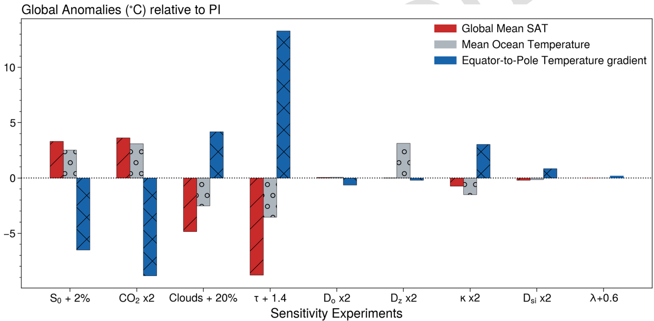
Figure A2. Anomalies in global mean surface air temperature, global mean ocean temperature, and the air temperature difference between the equatorial ( 0-10^\circ ) and polar regions ( 80-90^\circ ) for changes in the solar constant ( S_0 ), atmospheric CO_2 level ( CO_2 ), cloud amount, cloud optical depth ( \tau ), ocean diffusion coefficient for horizontal eddy and gyre heat transport ( D_o ), ocean diffusion coefficient for vertical heat transport ( D_z ), coefficient for turbulent heat fluxes ( \kappa ), sea ice thickness ( d_{si} ) and a Hadley cell parameter ( \lambda ).
