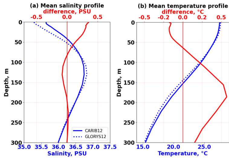
Figure 9. Time mean salinity (a) and temperature (b) profiles for the area average within the region of interest for this study (green box in Figure 1); CARIB12 (solid blue line) and GLOYS12 (dotted blue line). The difference between the two products is shown in red.
