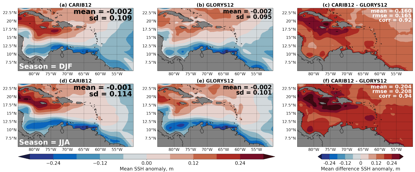
Figure 6. Time mean winter (a-c) and summer (d-f) SSH anomaly (SSHa, m) in the region of interest for this study (green box in Figure 1): (a,d) CARIB12, (b,e) GLORYS12, (c,f) CARIB12 minus GLORYS12 for winter and summer, respectively. The SSHa is the time mean SSH minus the spatial mean. Mean and standard deviation are shown for each product and seasonal mean. The mean bias, root mean squared error (rmse), and spatial correlation (corr) are shown in each comparison panel.
