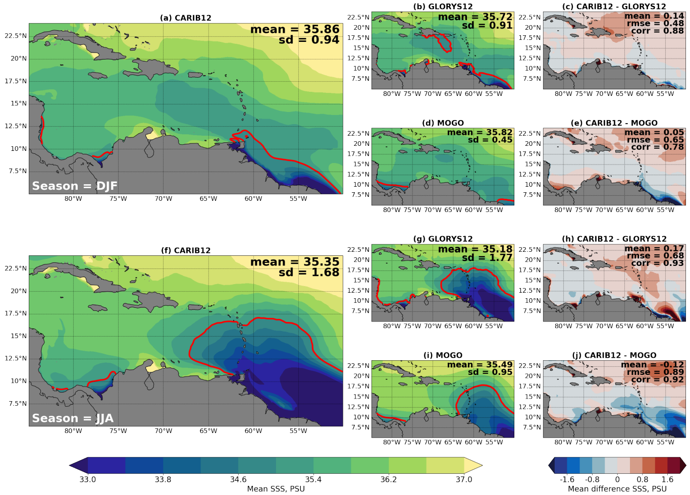
Figure 3. Time mean winter (a-e) and summer (f-j) SSS (PSU) in the region of interest for this study (green box in Figure 1): (a,f) CARIB12, (b,g) GLORYS12, (c,h) CARIB12 minus GLORYS12, (d,i) MOGO, (e,j) CARIB12 minus MOGO for winter and summer, respectively. The red line in panels (a, b, d, f, g, i) shows the 35 PSU isohaline as a proxy for the extent of the freshwater plumes from the Amazon and Orinoco rivers. Mean and standard deviation are shown for each product and seasonal mean. The mean bias, root mean squared error (rmse), and spatial correlation (corr) are shown in each comparison panel.
