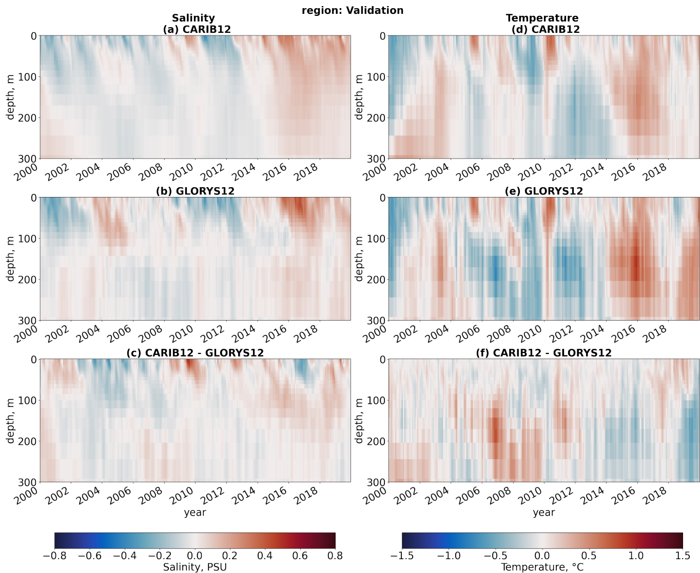
Figure 13. Area weighted mean monthly salinity anomaly within the validation region (green box in Figure 1): (a) CARIB12, (b) GLORYS12, (c) difference between the products. Area weighted mean seasonal temperature anomaly within the validation region: (d) CARIB12, (e) GLORYS12, (f) difference between the products.
