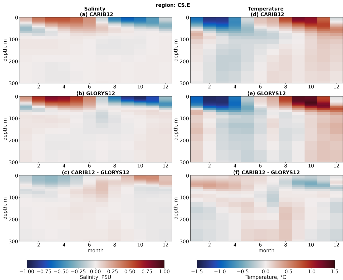
Figure 12. Area weighted mean seasonal salinity anomalies within the eastern CS region (CS.E) in Figure A5: (a) CARIB12, (b) GLORYS12, (c) difference between the products. Area weighted mean seasonal temperature anomaly within the validation region: (d) CARIB12, (e) GLORYS12, (f) difference between the products.
