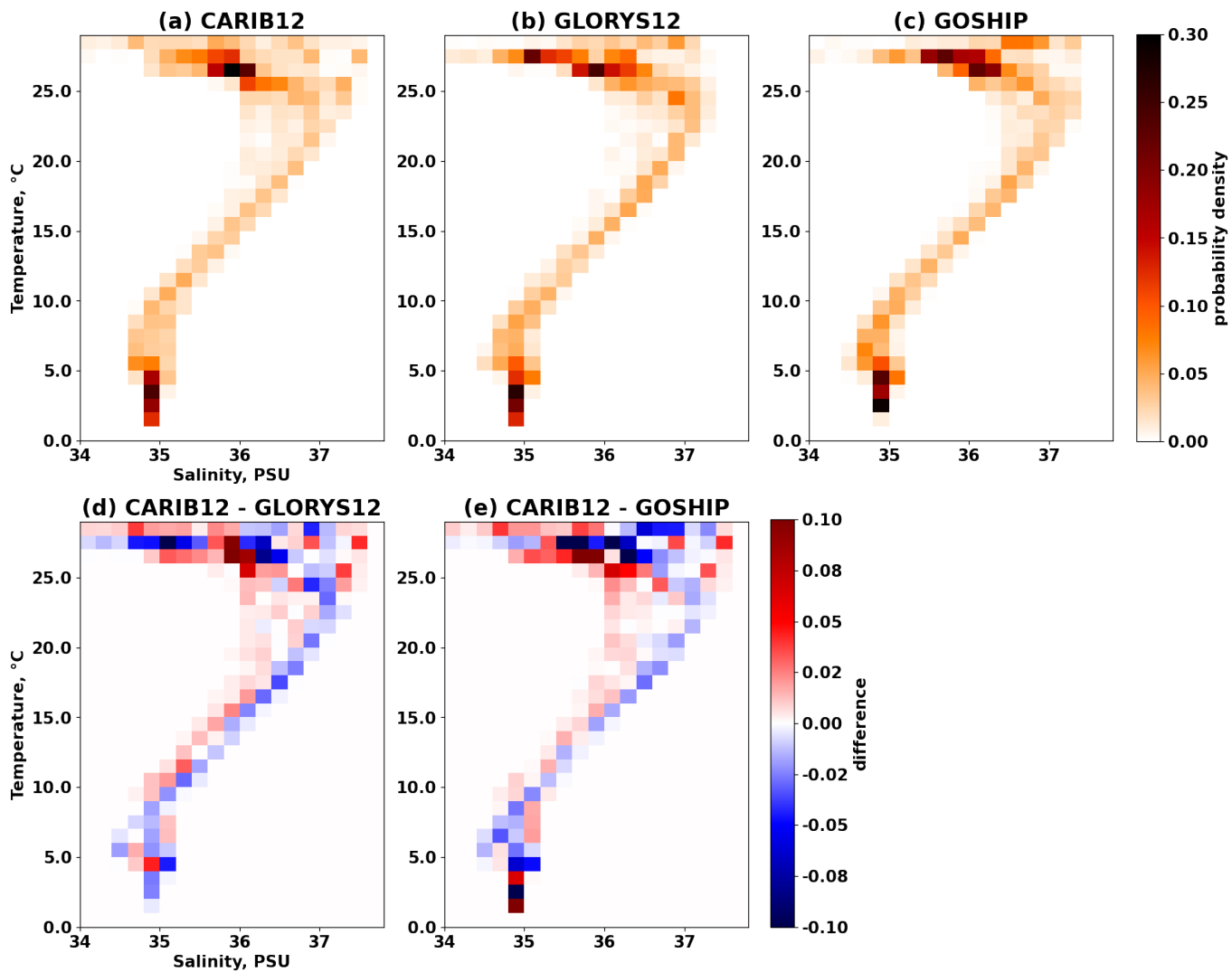
Figure 8. Temperature-Salinity joint probability density function for (a) CARIB12, (b) GLORYS12 and, (c) GO-SHIP. Panel (d) shows the difference between panel (a) and (b). Panel (e), the difference between (a) and (c).
