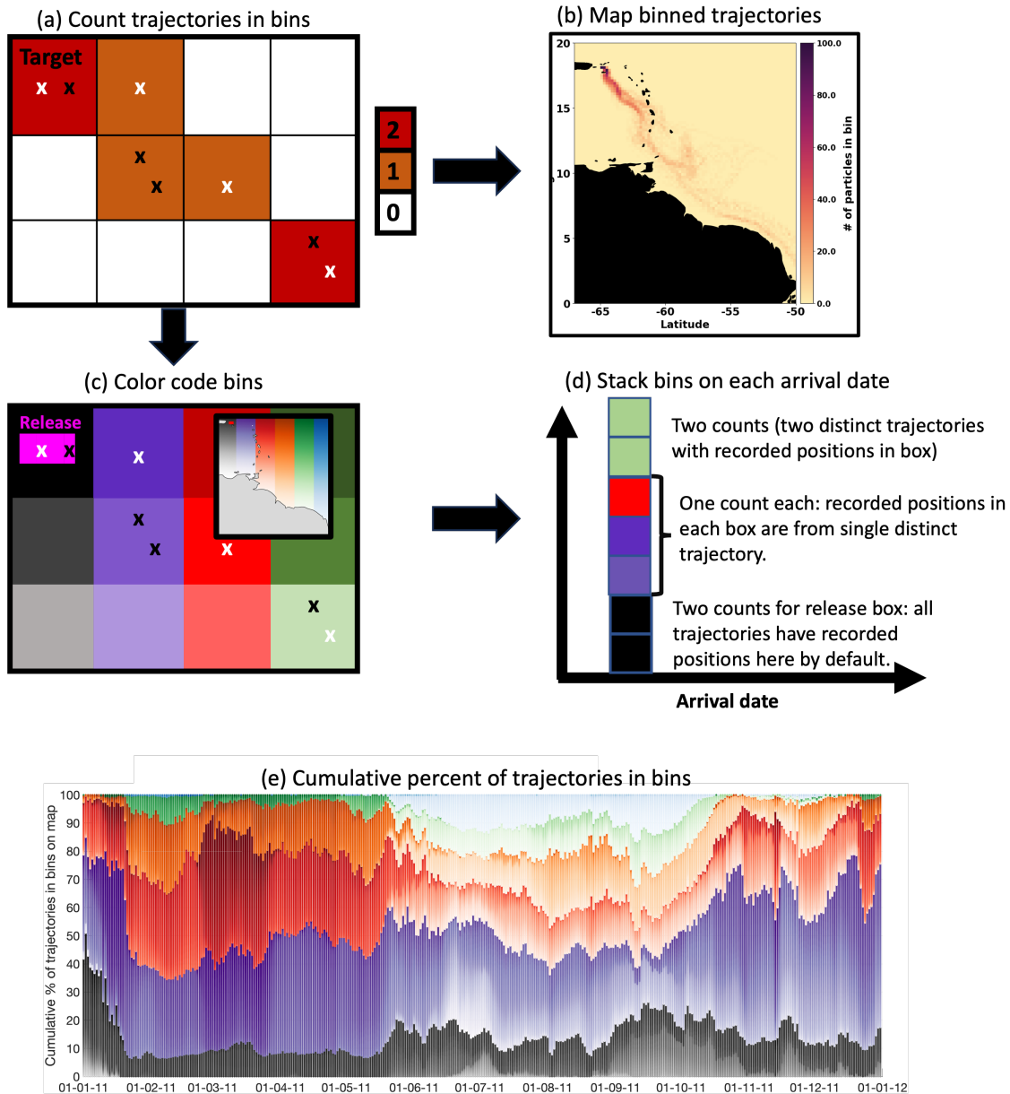
Figure B1. Schematic demonstrating the method used to generate Figures B2. a) Example positions of a trajectory for two particles (one black and one white). The 'Release' bin corresponds to the release site from which particles are backtracked. Positions within 0.2^\circ \times 0.2^\circ bins are counted and mapped as shown in panel (b). (c) Bins are now color-coded by their location (actual example in the inset map). A change in color represents a meridional position change, while a change in shading corresponds to a latitudinal position change. b) Example of position counting in each bin. (d) Example schematic of how the time series is generated. For each arrival date bins are stacked by the number of particles in each bin (scaled by the number of bins with recorded particles). (e) Actual example of the time series. The colored bins stacked on top of each day in the x-axis represent the pathway the waters came from. The inset map in panel (c) shows the color-coded bins to identify pathways. For a detailed description refer to Seijo-Ellis et al. (2023).
