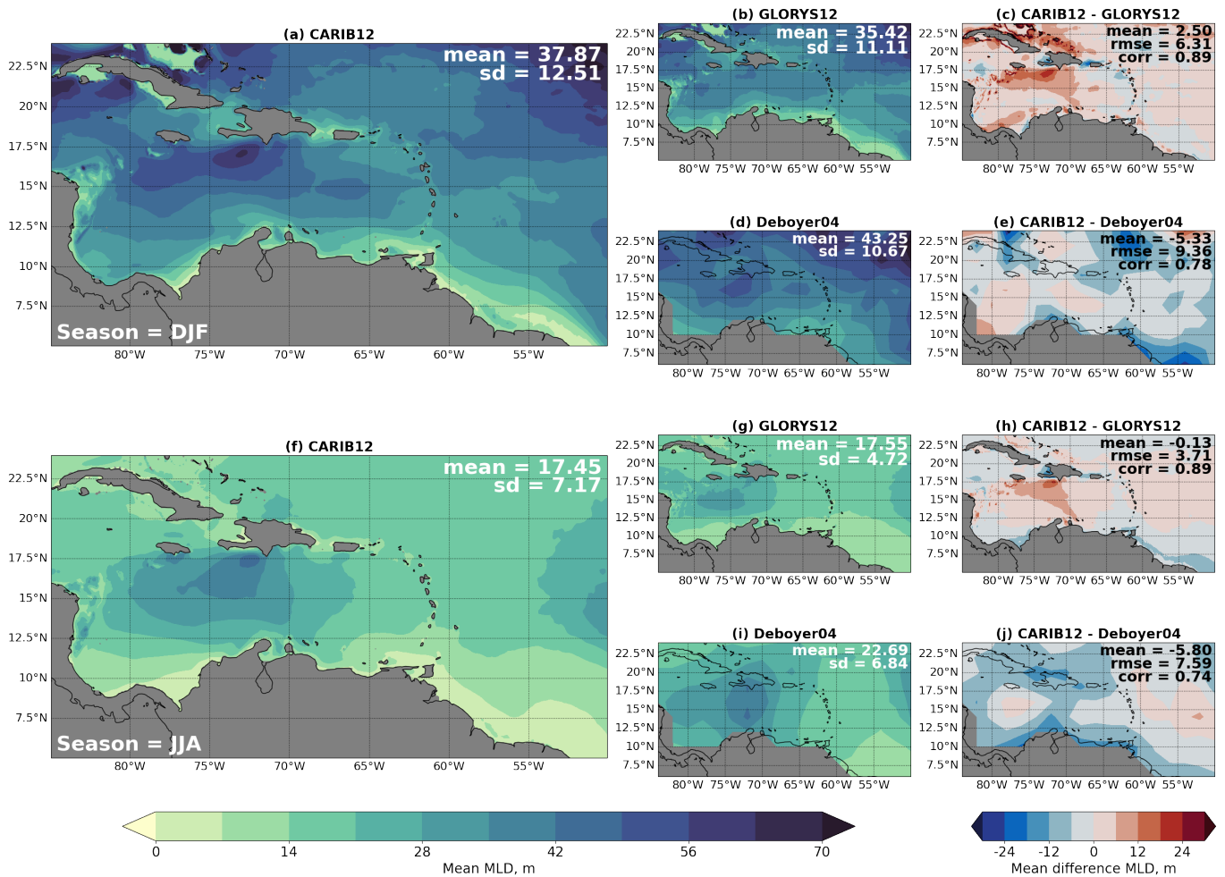
Figure 7. Time mean winter (a-e) and summer (f-j) MLD (m) in the region of interest for this study (green box in Figure 1): (a,f) CARIB12, (b,g) GLORYS12, (c,h) CARIB12 minus GLORYS12, (d,i) Deboyer, (e,j) CARIB12 minus Deboyer for winter and summer, respectively. Mean and standard deviation are shown for each product and seasonal mean. The mean bias, root mean squared error (rmse), and spatial correlation (corr) are shown in each comparison panel.
