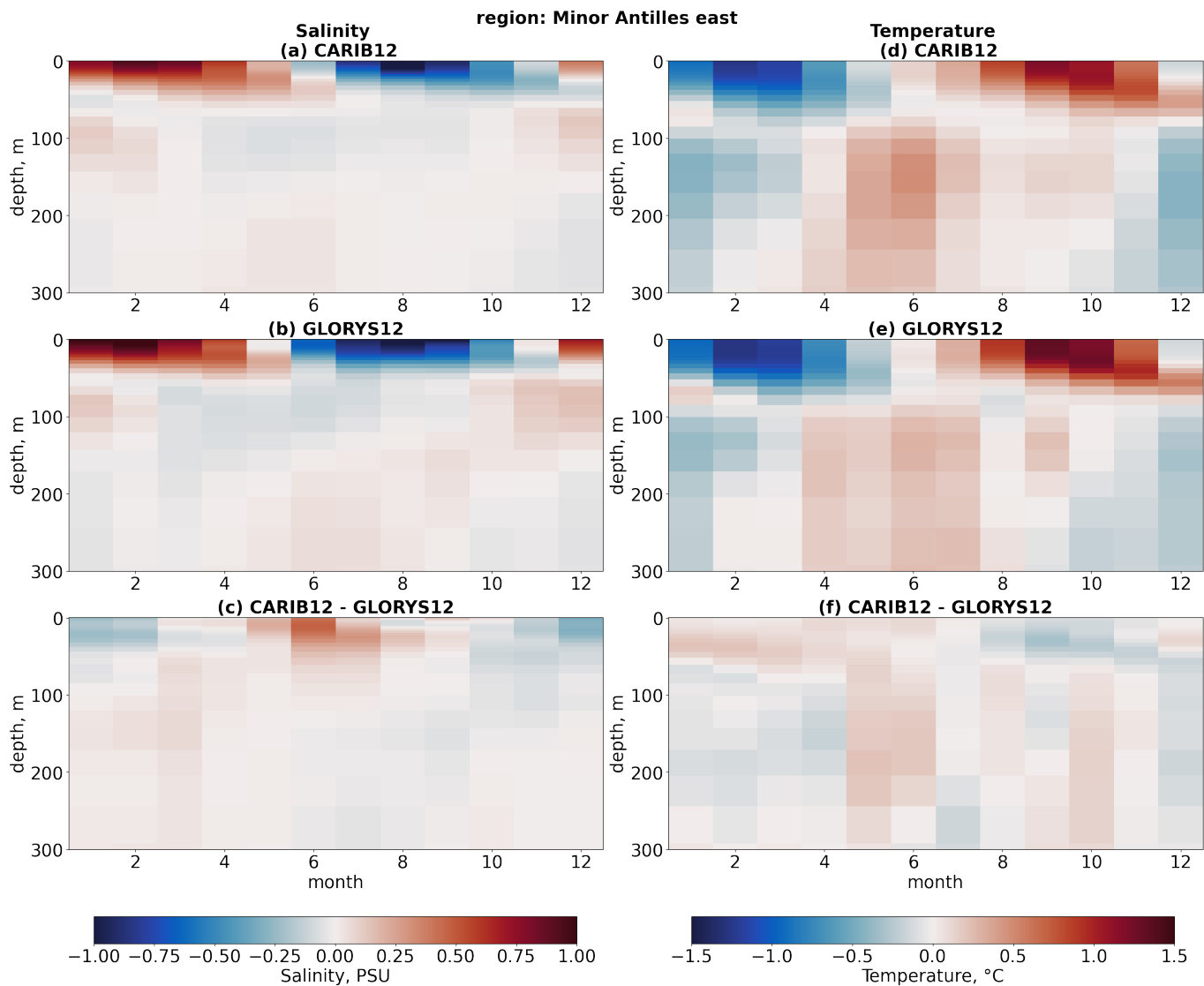
Figure 11. Area weighted mean seasonal salinity anomalies within the Minor Antilles east sub-region shown in Figure A5: (a) CARIB12, (b) GLORYS12, (c) difference between the products. Area weighted mean seasonal temperature anomaly within the validation region: (d) CARIB12, (e) GLORYS12, (f) difference between the products.
