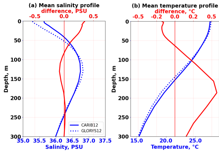
Figure 9. Time mean salinity (a) and temperature (b) profiles for the area average within the region of interest for this study (green box in Figure 1); CARIB12 (solid blue line) and GLOGY12 (dotted blue line). The difference between the two products is shown in red.
