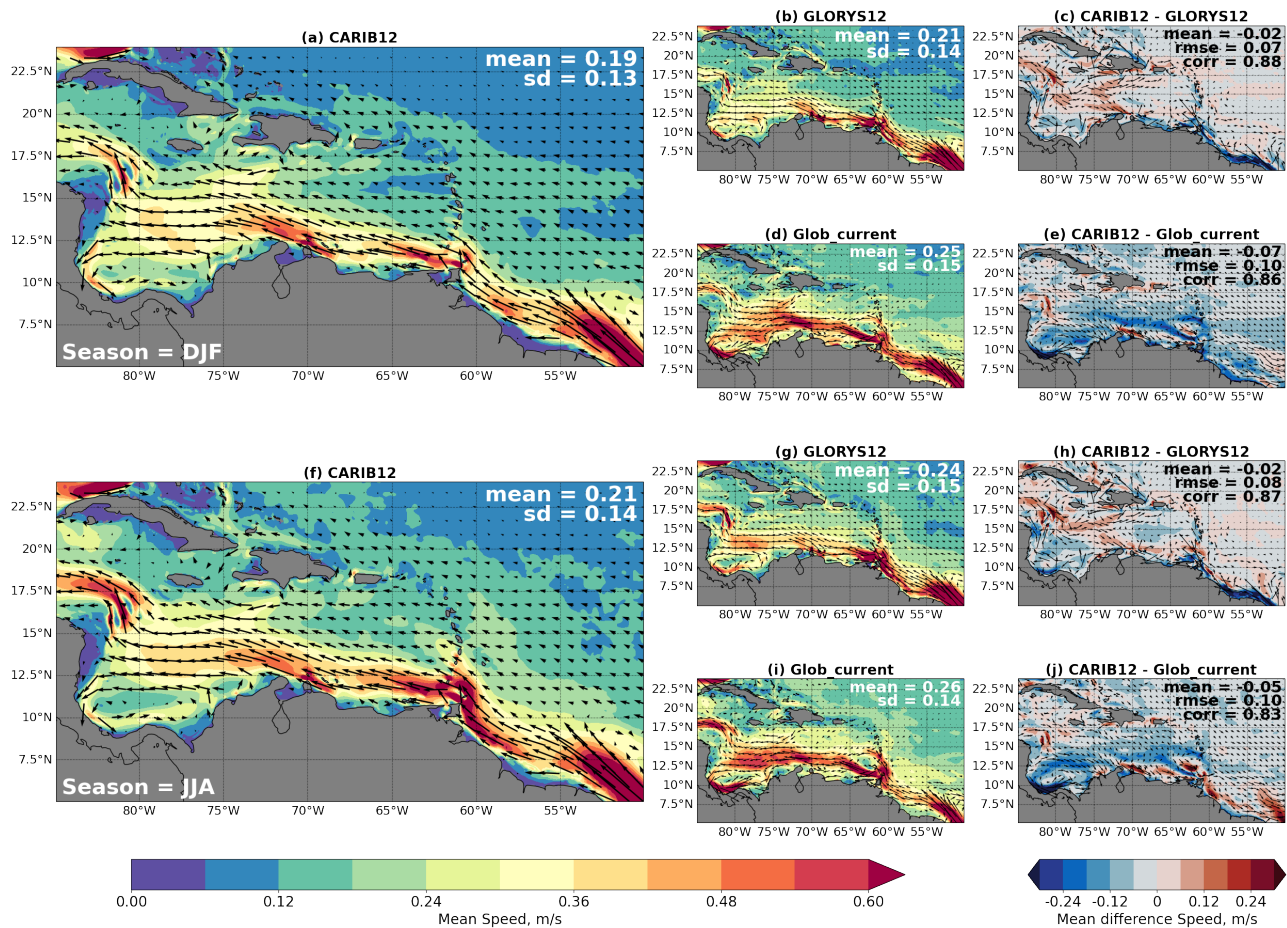
Figure 4. Time mean winter (a-e) and summer (f-j) surface speed (m/s) in the region of interest for this study (green box in Figure 1): (a,f) CARIB12, (b,g) GLORYS12, (c,h) CARIB12 minus GLORYS12, (d,i) GLOBCURRENT, (e,j) CARIB12 minus GLOBCURRENT for winter and summer, respectively. Black arrows show the direction of the surface flow with the size of the arrows scaled by the magnitude of the speed. Mean and standard deviation are shown for each product and seasonal mean. The mean bias, root mean squared error (rmse), and spatial correlation (corr) are shown in each comparison panel.
