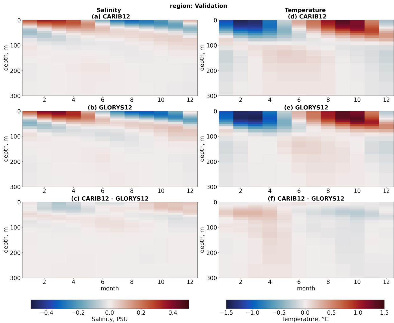
Figure 10. Area weighted mean seasonal salinity anomalies within the validation region (green box in Figure 1): (a) CARIB12, (b) GLORYS12, (c) difference between the products. Area weighted mean seasonal temperature anomaly within the validation region: (d) CARIB12, (e) GLORYS12, (f) difference between the products.
