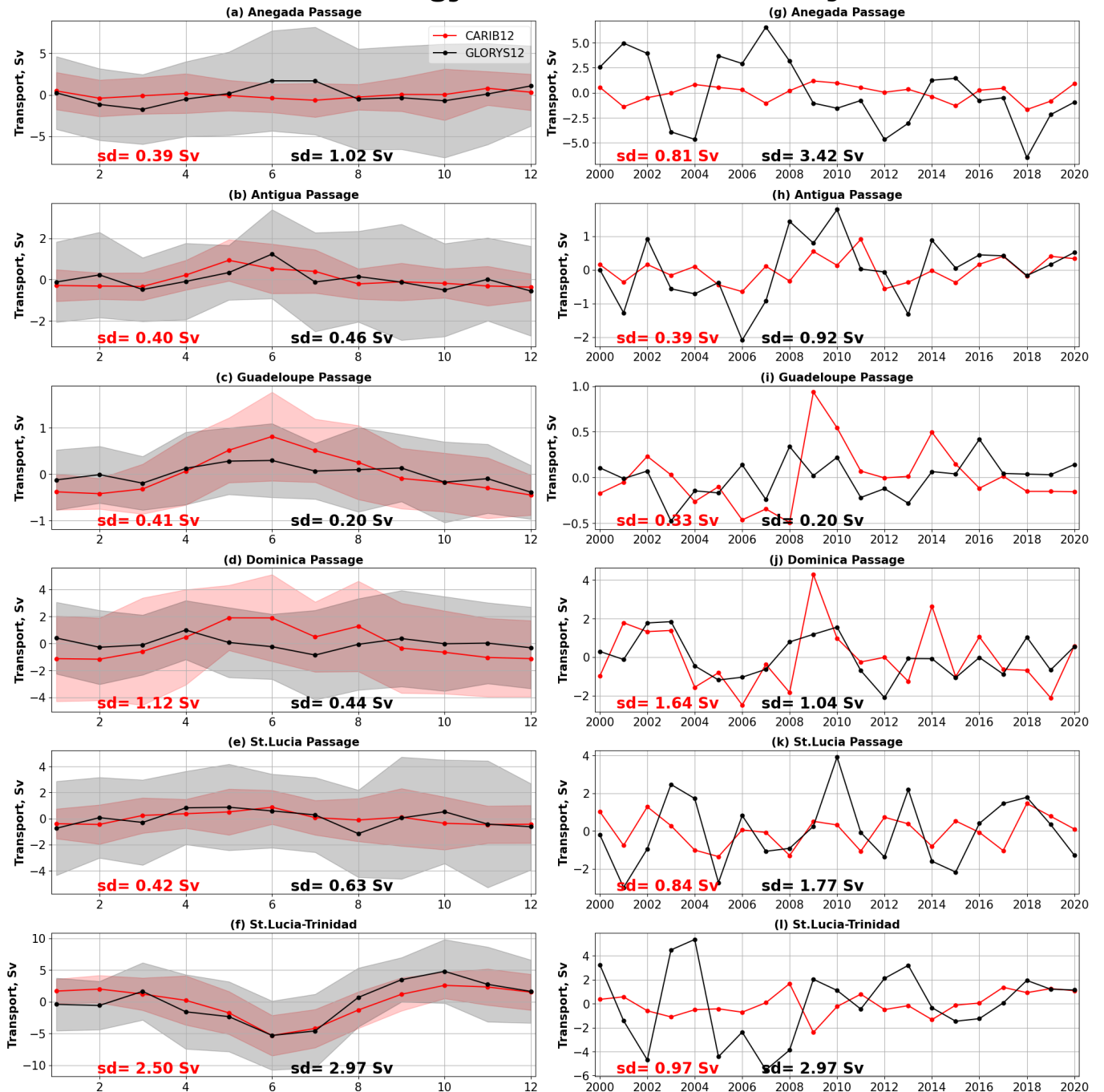
Figure 16. Transport through passages in the Eastern Caribbean Sea from CARIB12 (red) and GLORYS12 (black): (a-f) seasonal anomalies, and (g-l) yearly anomalies. In panels (a-f), the shading shows the standard deviation for each month (i.e. standard deviation of all January means, and so on).
