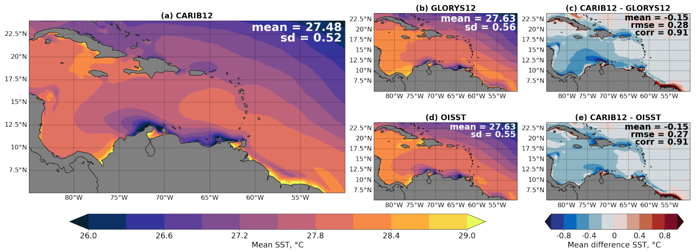
Figure 2. Time mean SST (°C) in the region of interest for this study (green box in Figure 1), during 2000-2020: (a) CARIB12, (b) GLORYS12, (c) CARIB12 minus GLORYS12, (d) OISST, (e) CARIB12 minus OISST. Mean and standard deviation are shown for each product (a, b and d). The mean bias, root mean squared error (rmse), and spatial correlation (corr) are shown in each comparison panel (c and e).
