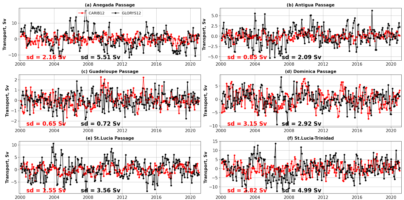
Figure 13. Transport through passages in the Eastern Caribbean Sea: monthly anomalies from CARIB12 (red) and GLORYS12 (black) for (a) Anegada Passage, (b) Antigua Passage, (c) Guadeloupe Passage, (d) Dominica Passage, (e) St. Lucia Passage and, (f) the St. Lucia - Trinidad transect. The standard deviation of the time series is indicated at the bottom of each panel, color coded by product. Time mean transports for each passage can be found in Table 4 for both CARIB12 and GLORYS12, as well as available observations.
