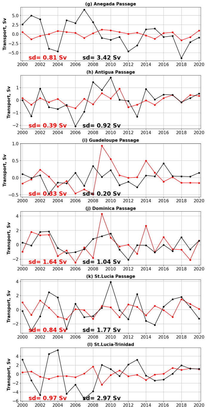
Figure 14. Transport through passages in the Eastern Caribbean Sea from CARIB12 (red) and GLORYS12 (black): (a-f) seasonal anomalies, and (g-l) yearly anomalies. In panels (a-f), the shading shows the standard deviation for each month (i.e. standard deviation of all January means, and so on).
