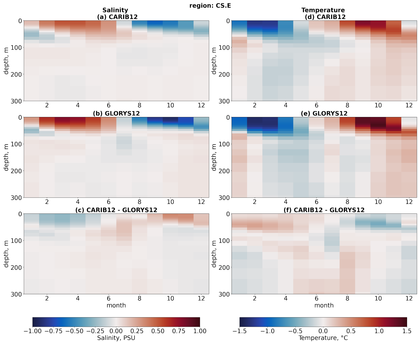
Figure A8. Area weighted mean seasonal salinity anomalies within the eastern CS region (CS.E) in Figure A5: (a) CARIB12, (b) GLORYS12, (c) difference between the products. Area weighted mean seasonal temperature anomaly within the validation region: (d) CARIB12, (e) GLORYS12, (f) difference between the products.
