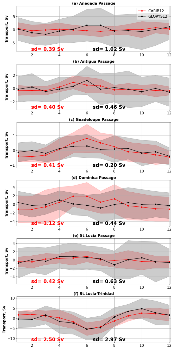
Figure 14. Transport through passages in the Eastern Caribbean Sea from CARIB12 (red) and GLORYS12 (black): (a-f) seasonal anomalies, and (g-l) yearly anomalies. In panels (a-f), the shading shows the standard deviation for each month (i.e. standard deviation of all January means, and so on).
