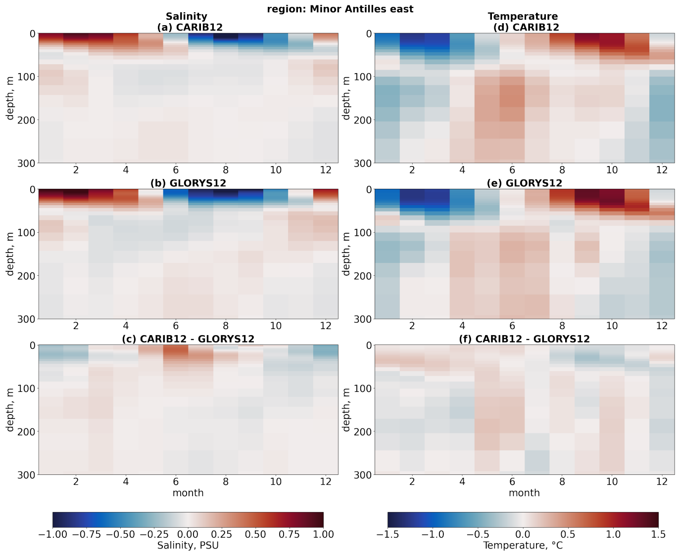
Figure A7. Area weighted mean seasonal salinity anomalies within the Minor Antilles east sub-region shown in Figure A5: (a) CARIB12, (b) GLORYS12, (c) difference between the products. Area weighted mean seasonal temperature anomaly within the validation region: (d) CARIB12, (e) GLORYS12, (f) difference between the products.
