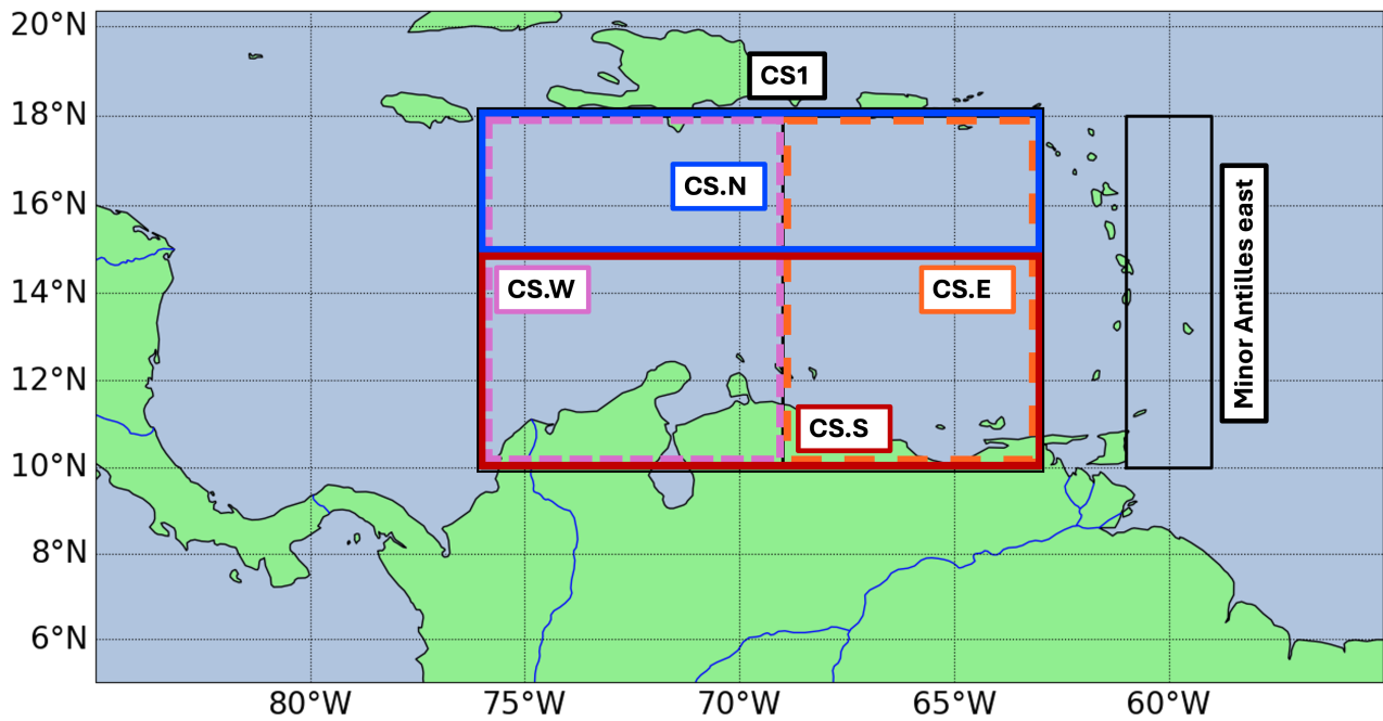
Figure A5. Sub-regions used for additional validation of CARIB12. Region CS1 encompasses all 4 subregions CS.N, CS.S, CS.E and CS.W. Only validations for CS1, CS.E and Minor Antilles east are shown in addition to the the full validation region shown in Figure 1.
