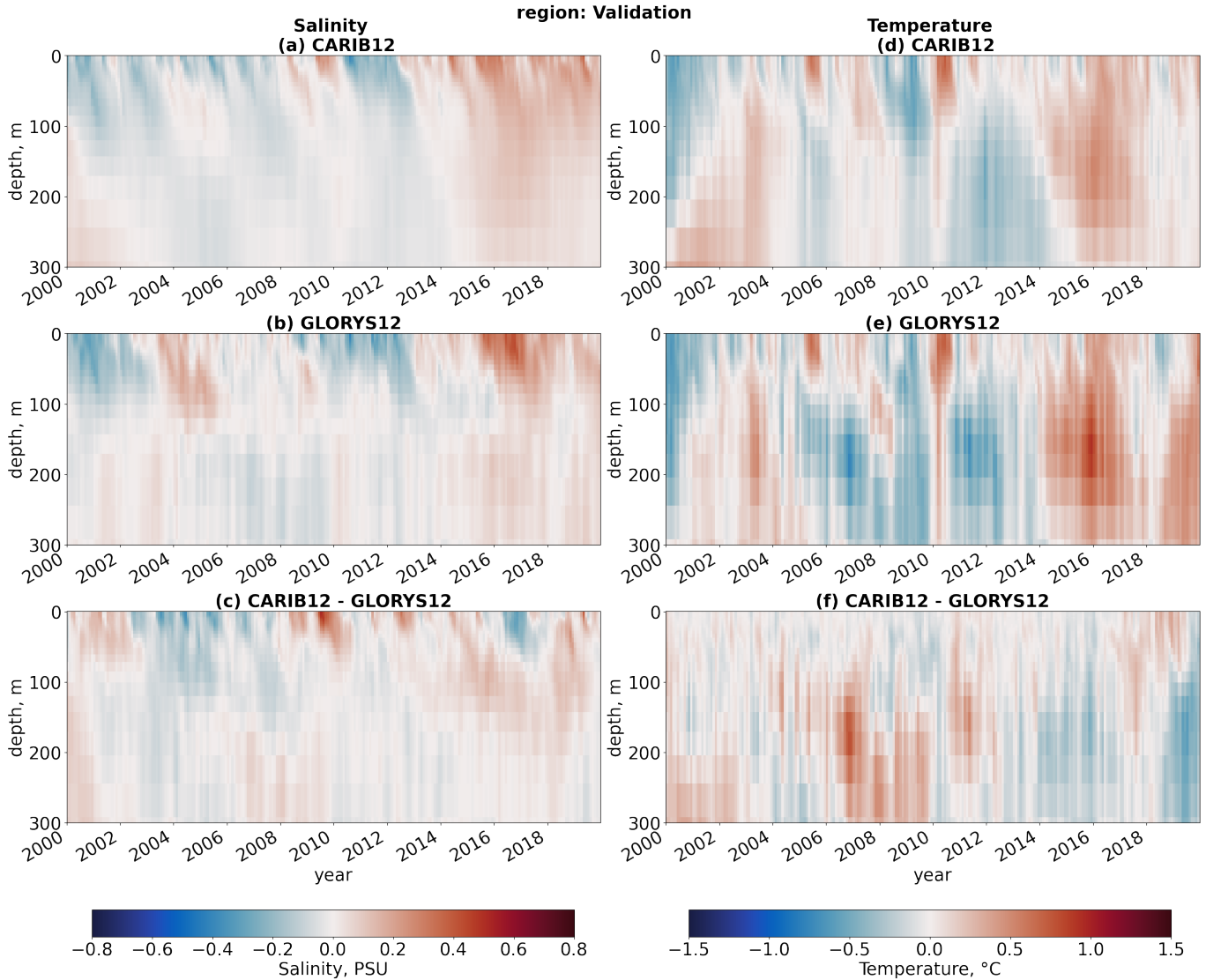
Figure 11. Area weighted mean monthly salinity anomaly within the validation region (green box in Figure 1): (a) CARIB12, (b) GLORYS12, (c) difference between the products. Area weighted mean seasonal temperature anomaly within the validation region: (d) CARIB12, (e) GLORYS12, (f) difference between the products.
