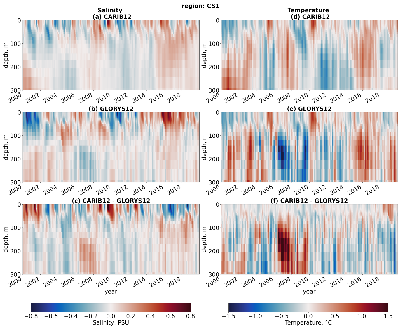
Figure 12. Area weighted mean monthly salinity anomaly within the CS (CS1 in Figure A5): (a) CARIB12, (b) GLORYS12, (c) difference between the products. Area weighted mean seasonal temperature anomaly within the validation region: (d) CARIB12, (e) GLORYS12, (f) difference between the products.
