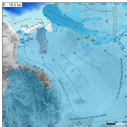
Figure 6: The evolution of ice flow using the 500-year timeslices of NADI-1 (Dalton et al., 2023). In panel A, green numbering indicates pre-LGM flowsets and black numbering indicates unclassified flowsets. Due to the size of the
