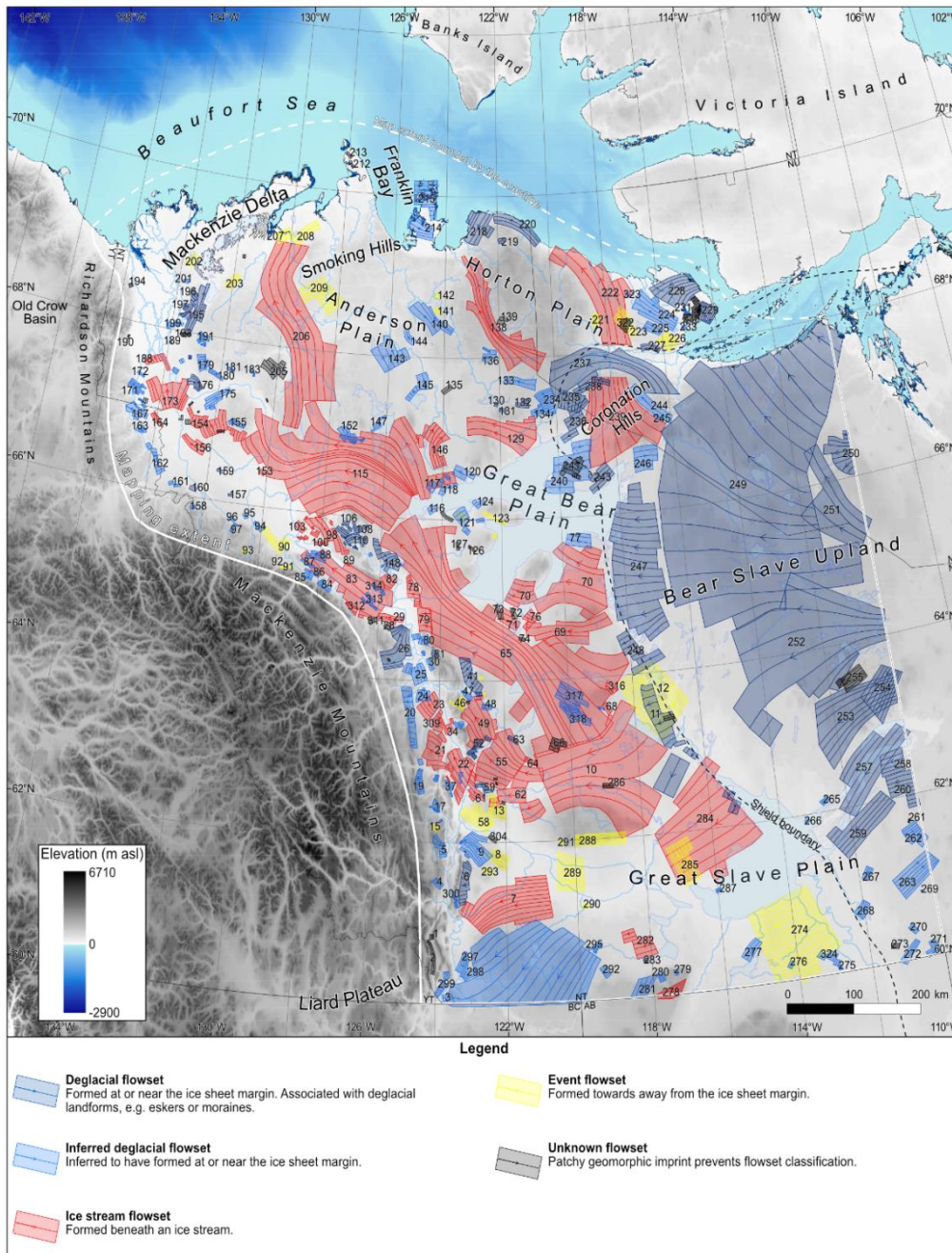
310 Figure 4: Flowset map of the northwest sector of the Laurentide Ice Sheet. Flowsets have been assigned a number with corresponding information available in Supplementary Table 1. Due to the scale of the figure, only the largest flowsets are labelled in this figure. An A0 version of this map is provided in the supplementary materials, which includes labels for each flowset and information on the cross-cutting of different flowsets (Supplementary Figure 1). The flowsets are classified according to the criteria in Table 1.
