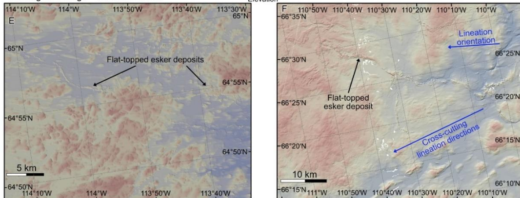
Figure 10: Glacial landforms examples from the former northwestern LIS bed which highlight the contrasting styles of deglaciation across the region. Panel locations are indicated on Figure 1. Note some landforms may only be visible
