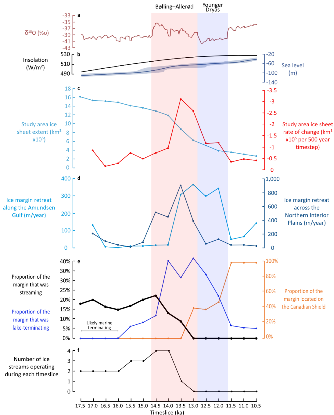
Figure 11: (A) \delta^{18}\text{O} record from the Greenland GRIP ice core displayed in red (Rasmussen et al., 2014; Seierstad et al., 2014), (B) Relative sea level curve is blue is adapted from Carlson and Clark (2012) and based on a compilation of far-field sites and the mean summer insolation at 65^\circ\text{N} is in black (Laskar et al., 2004). (C) The total extent of the LIS (blue line) in our study area (displayed in Figure 1) at each 500-year timestep covered in our reconstruction, based upon the
