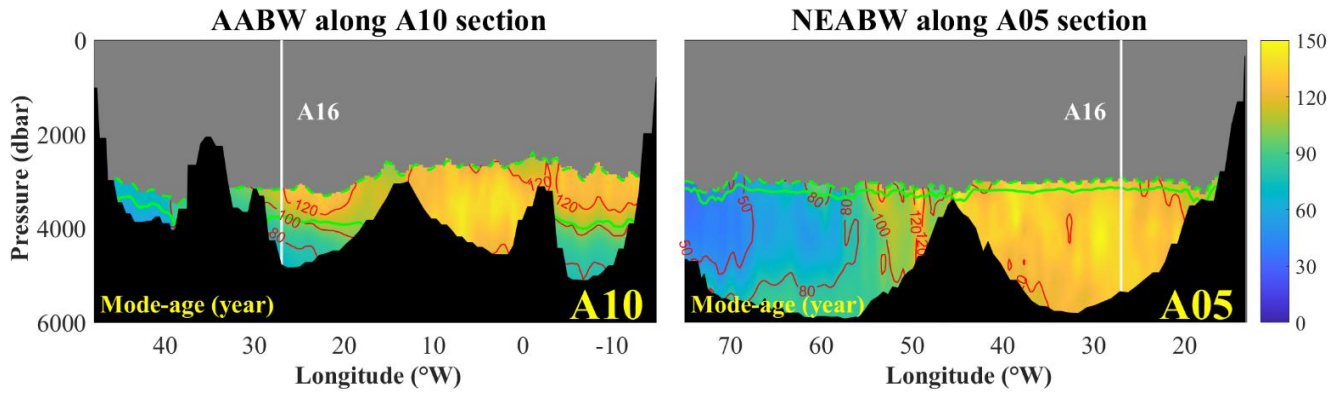
Figure 13. Mode-ages of AABW and NEABW along the A16 (a), A05 and A10 (b) section lines.
