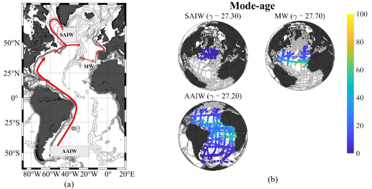
Figure 8. Mode-ages of intermediate water masses in the Atlantic Ocean.
