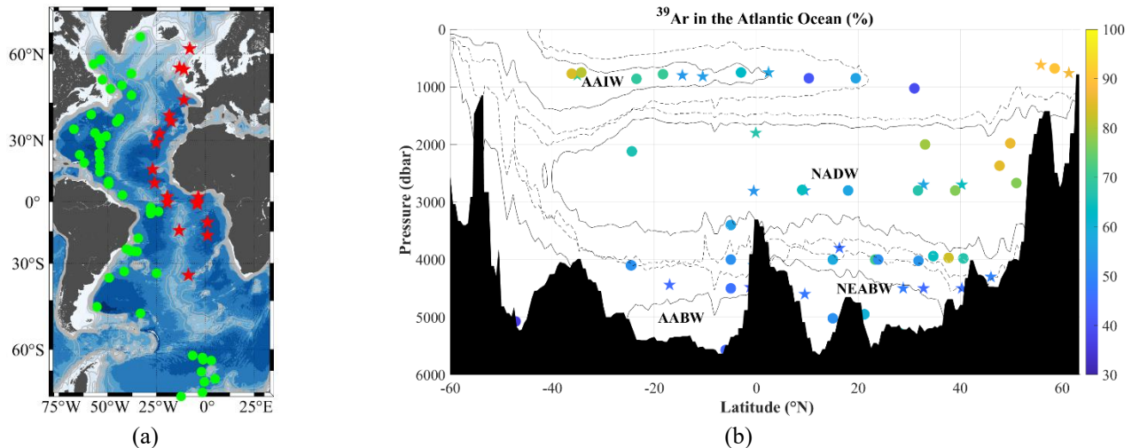
Figure 16. (a) Map of the ^{39}\text{Ar} sampling stations. The green circle dots show the stations in the west Atlantic Ocean (west of the Mid Atlantic Ridge), while the red stars show the stations in the east Atlantic Ocean. (b) Distributions of ^{39}\text{Ar} in the
