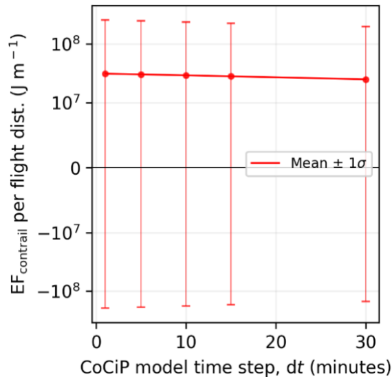
680 Figure A3: Change in the global mean and standard deviation of EF_{\text{contrail}} per flight distance across different CoCiP model time steps ( dt ). Contrails are simulated globally at FL360 (10,973 m) on the 7 th of January 2019 at 03:00:00, with the nominal nvPM aircraft-engine group. The y-axis uses a logarithmic scale for |EF_{\text{contrail}}| > 10^7 J m^{-1} and a linear scale between 10^{-7} and 10^7 J m^{-1} .
