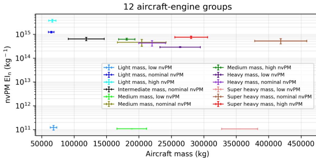
Figure A5: Range of aircraft mass and nvPM El_n for each aircraft-engine group when they are clustered into 12 groups. The error bars for each data point represent one standard deviation of these values, which are provided by the 2019 global aviation emissions inventory based on ADS-B (GAIA) (Teoh et al., 2024b).
