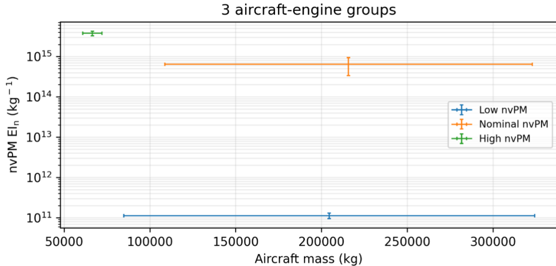
Figure A7: Range of aircraft mass and nvPM EI n for each aircraft-engine group when they are clustered into 3 groups. The error bars for each data point represent one standard deviation of these values, which are provided by the 2019 global aviation emissions inventory based on ADS-B (GAIA) (Teoh et al., 2024b).
