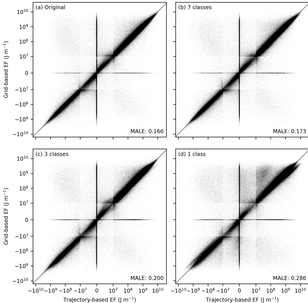
Figure 3: Pointwise errors between \text{EF}_{\text{contrail}}^{\text{traj}} and \text{EF}_{\text{contrail}}^{\text{grid}} when the grid-based CoCiP is configured: (a) using the exact/original aircraft-engine types (i.e., the same as the trajectory-based CoCiP); and with (b) N=7 ; (c) N=3 ; and (d) N=1 aircraft-engine groups respectively. Each panel contains 10,000,000 randomly-sampled flight waypoints. The axes use a logarithmic scale for |\text{EF}_{\text{contrail}}| > 10^7 \text{ J m}^{-1} and a linear scale between 10^{-7} and 10^7 \text{ J m}^{-1} . For both axes, the box-like structures observed around 10^{-7} and 10^7 \text{ J m}^{-1} arise from the transition between the linear and logarithmic scale.
