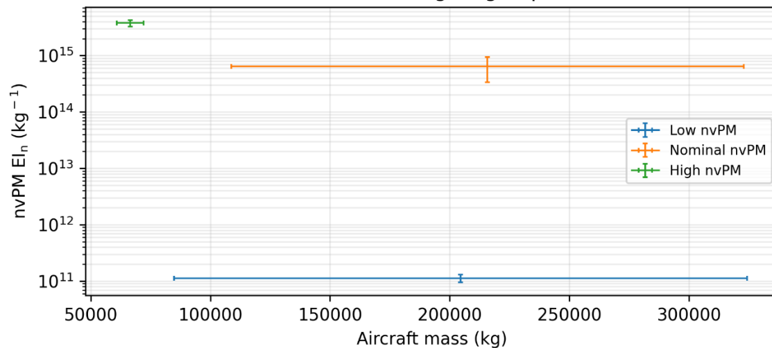
755 Figure A7: Range of aircraft mass and nvPM EI n for each aircraft-engine group when they are clustered into 3 groups. The error bars for each data point represent one standard deviation of these values, which are provided by the 2019 global aviation emissions inventory based on ADS-B (GAIA) (Teoh et al., 2024b).
