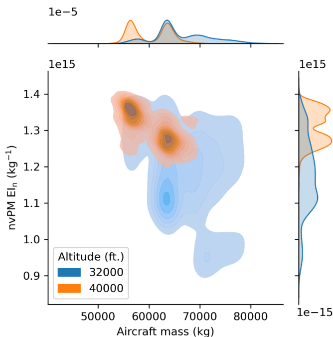
235 Figure 1: Multivariate distribution of aircraft mass and \text{nvPM EI}_n for one aircraft-engine group (light aircraft mass and nominal \text{nvPM EI}_n , see Table 2) at 32,000 feet (in blue) and 40,000 feet (in orange). The underlying data is provided by the 2019 global aviation emissions inventory based on ADS-B (GAIA) (Teoh et al., 2024b). The multi-modal distribution of the aircraft mass and \text{nvPM EI}_n is due to the inclusion of two comparable aircraft engine families (Boeing 737 and Airbus A320 families) in the same group, each exhibiting distinct operating characteristics. The variations in \text{nvPM EI}_n with altitude results from changes in aircraft mass and air density, both of which influence the engine thrust settings and subsequently \text{nvPM} emissions (EASA, 2021).
