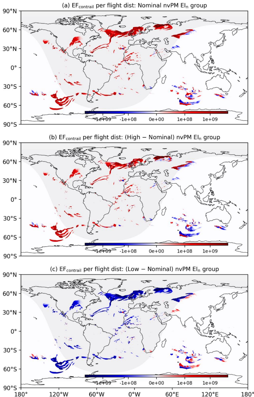
400 Figure 4: The (a) absolute EF_{\text{contrail}} per flight distance for the aircraft-engine group with nominal nvPM; and the absolute difference in EF_{\text{contrail}} per flight distance between the (b) nominal and high nvPM aircraft-engine group; and (c) nominal and low nvPM aircraft-engine group. The global contrail climate forcing shown here are simulated at FL360 (10,973 m) on the 7 th of January 2019 at 03:00:00 UTC. Basemap plotted using Cartopy 0.22.0 and sourced from Natural Earth; licensed under public domain.
