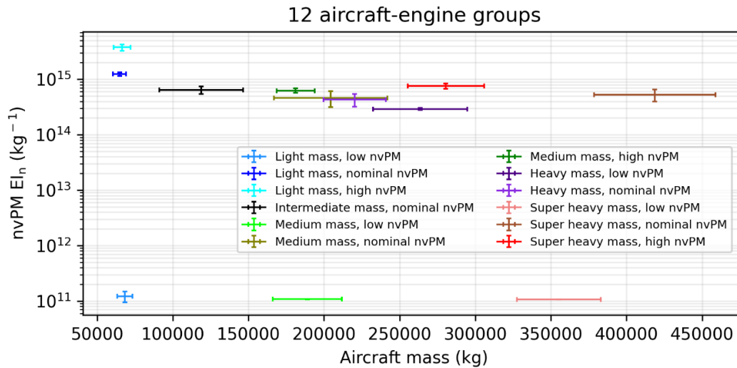
735 Figure A5: Range of aircraft mass and nvPM El_n for each aircraft-engine group when they are clustered into 12 groups. The error bars for each data point represent one standard deviation of these values, which are provided by the 2019 global aviation emissions inventory based on ADS-B (GAIA) (Teoh et al., 2024b).
