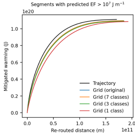
290 Figure 2: Performance curves for the trajectory-based CoCiP (black line) and the grid-based CoCiP when it is configured using the exact/original aircraft-engine types (i.e., the same as the trajectory-based CoCiP; blue line), and with N=7 (orange line), N=3 (green line), and N=1 (red line) aircraft-engine groups respectively. Further methodological information used to construct these performance curves can be found in Appendix A5.
