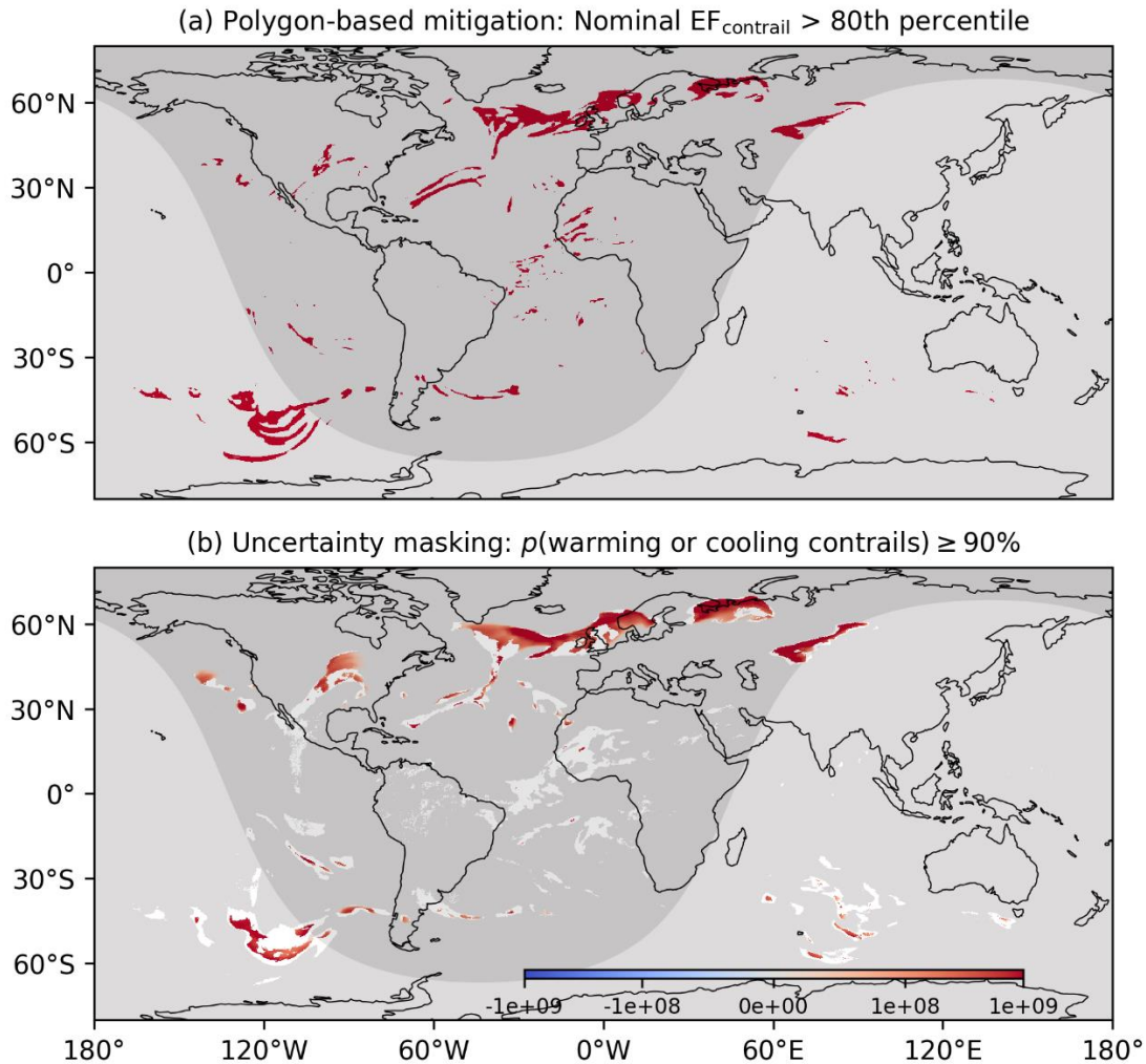
490 Figure 9: Application of the simulated EF_{\text{contrail}} per flight distance for contrail mitigation, where flight planners can: (a) construct polygons and avoid flying in regions forecast with strongly warming contrails (i.e., grid cells where the EF_{\text{contrail}} per flight distance is greater than the 80 th percentile ( 5.0 \times 10^8 \text{ J m}^{-1} ); and/or (b) account for uncertainties in the simulated contrail climate forcing by 495 masking and disregarding grid cells (shown in white) when their probability of forming net warming (or cooling) contrails is less than 90%. The global contrail climate forcing shown here are from the nominal nvPM aircraft-engine group and simulated at FL360 (10,973 m) on the 7 th of January 2019 at 03:00:00. For panel (a), the impact of dt on regions forecast with strongly warming contrails are evaluated in Appendix A2. Basemap plotted using Cartopy 0.22.0 and sourced from Natural Earth; licensed under public domain.
