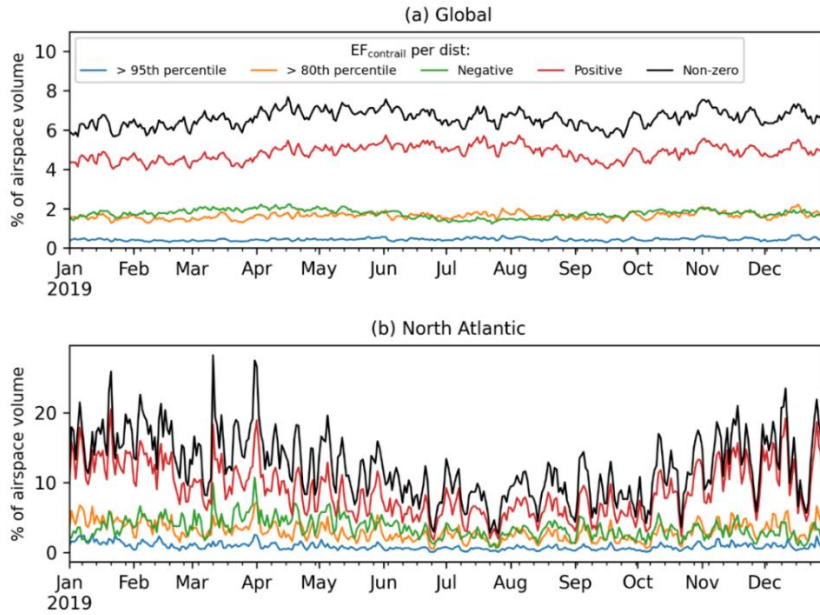
405 Figure 5: Daily means of the percentage of airspace volume: (a) globally; and (b) over the North Atlantic region (between 40–63°N and 70–5°W) in 2019, where the EF_{\text{contrail}} per flight distance is: (i) greater than 1.54 \times 10^9 \text{ J m}^{-1} (95 th percentile, blue lines); (ii) greater than 5.0 \times 10^8 \text{ J m}^{-1} (80 th percentile, orange lines); (iii) negative (i.e., cooling contrails, green lines); (iv) positive (i.e., warming contrails, red lines); and (v) non-zero (i.e., all contrails, black lines).
