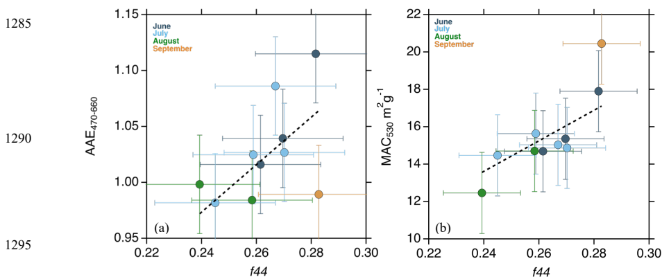
Figure 20. a) AAE_{470-660\text{nm}} versus average f_{44} for the 10 selected plume events. b) Average f_{44} versus MAC_{530} ( \text{m}^2 \text{g}^{-1} ) for the 10 selected plume events. Markers are colored by month and error bars represent the standard deviation of the data set. The black dashed line is the best-fit line calculated by linear regression analysis. The best-fit line is weighted by \mu\text{g m}^{-3} \text{min}^{-1} .
