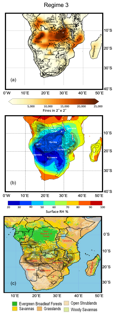
Figure 5. a) Regime 3 fire density maps showing 2°x2° bins of number of fires detected by the NASA SUOMI NPP satellite between August 19, 2017 and September 11, 2017. b) NCEP reanalysis Regime 3 mean surface relative humidity, with contours indicating fire number density. c) MODIS annual (2017) mean land use map with Regime 3 fire number density contours.
