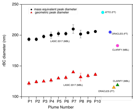
525 Figure 6. Mean rBC_{mpd} (circles) and rBC_{gpd} (triangles) for multiple field campaigns in the SEA. Filled colored circles and triangles represent the observed data from the LASIC MBL (black, red), ORACLES FT (blue, yellow) (Dobracki et al., 2023), CLARIFY MBL (pink, green) (Wu et al., 2020), and ATTO FT (cyan) (Holanda et al., 2022). Error bars are the standard 530 deviation of each plume event.
