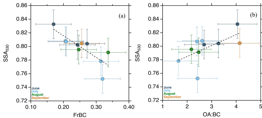
1180 Figure. 17 a) SSA_{530} versus FrBC b) SSA_{530} versus OA:rBC. Markers are colored by month and error bars represent the standard deviation of the data set. The Black dashed line is the best fit line calculated by linear regression analysis. The best-fit line is weighted by \mu\text{g m}^{-3} \text{min}^{-1} .
