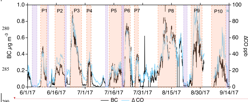
290 Figure 1. Time series of black carbon mass concentration ( \mu\text{g m}^{-3} ) (black) and \Delta CO mixing ratio (ppb) (blue), calculated by removing the bottom 5th percentile of the monthly \Delta CO distribution from the total, from June 1, 2017 through September 15, 2017. Pink boxes indicate selected plume events and purple boxes indicate clean events.
