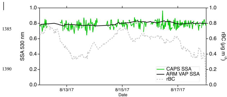
1395 Figure A1. SSA_{530} determined from the PSAP and nephelometer (black) and CAPS-SSA (green). rBC mass concentration (grey dashed line) indicates this comparison was done in the plume.
