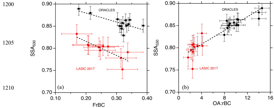
1215 Figure 18. a) SSA_{530} versus FrBC for ORACLES level leg data (black) (Dobracki et al., 2022) and LASIC 2017 major plume event data (red). b) SSA_{530} versus OA:rBC for ORACLES level leg data (black) and LASIC 2017 major plume event data (red). Error bars represent the standard deviation of the data set and the black dashed line is the best-fit line calculated by linear regression analysis.
