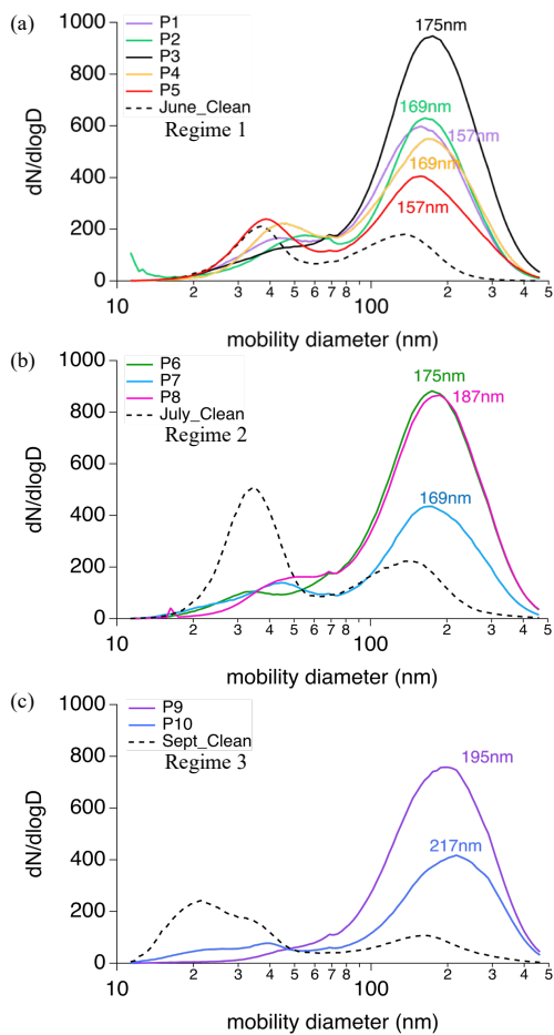
Figure 11. Plume mean SMPS aerosol size distributions ( dN/d\log D cm -3 ) for each selected plume event in a) Regime 1, b) Regime 2, c) Regime 3. Monthly mean distributions from clean periods are denoted as black dashed lines.
