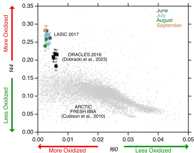
Figure 15. f_{44} versus f_{60} with LASIC plume event data (filled circles), colored by month, ORACLES 2016 level flight average data where OA > 20\mu\text{g}\text{m}^{-3} (black squares) (Dobracki et al., 2023), and fresh BBA from the Arctic (grey dots) (Cubison et al., 2010). Error bars represent the standard deviation of the data set.
