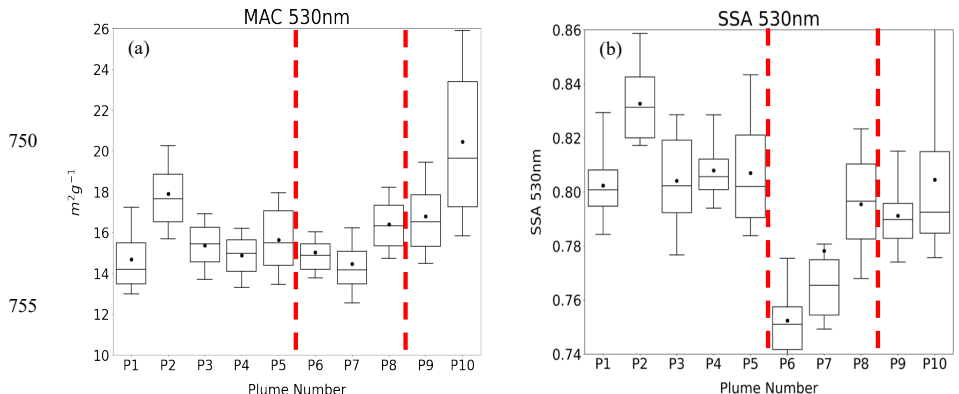
760 Figure 12. Box-whisker distributions of a) MAC_{530} and b) SSA_{530} with lowest whisker at 10 th percentile, lowest bar at 25 th percentile, middle bar at 50 th percentile, upper bar at 75 th percentile, and highest whisker at 90 th percentile. Filled circles represent the mean. Red dashed lines distinguish the three regimes discussed in the text.
