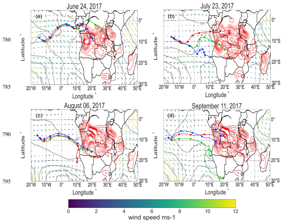
800 Figure 13. HYSPLIT back trajectories at 800 m (red), 1100 m (blue), and 1400 m (green) above sea level for polluted days initiated at 1200 UTC for a) June 24, 2017, b) July 23, 2017, c) August 06, 2017, and d) September 11, 2017. Each filled colored circle represents the trajectory location at 00 UTC after initiation. Grey solid lines represented NCEP reanalysis geopotential height at 850 hPa. Wind direction and magnitude are represented by arrows colored by windspeed (0-25m s -1 ). Fire density is shown in red contours for total fires two weeks prior to the initiation date. 805
