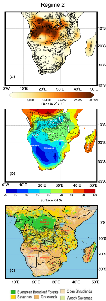
Figure 4. a) Regime 2 fire density maps showing 2^{\circ} \times 2^{\circ} bins of the number of fires detected by the NASA SUOMI NPP satellite between July 14, 2017 and August 17, 2017. b) NCEP reanalysis Regime 2 mean surface relative humidity, with contours indicating fire number density. c) MODIS annual (2017) mean land use map with Regime 2 fire number density contours.
