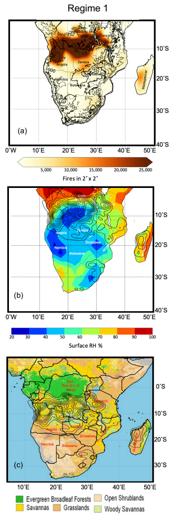
405 Figure 3. a) Regime 1 fire density maps showing 2^{\circ} \times 2^{\circ} bins of the number of fires detected by the NASA SUOMI NPP satellite between May 31 , 2017 and July 20, 2017. b) NCEP reanalysis Regime 1 mean surface relative humidity, with contours indicating fire number density. c) MODIS annual (2017) mean land use map with Regime 1 fire number density contours.
