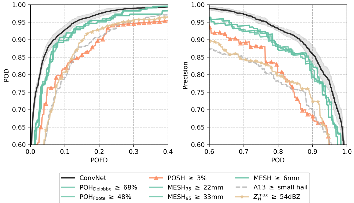
ROC and Precision-Recall curve
