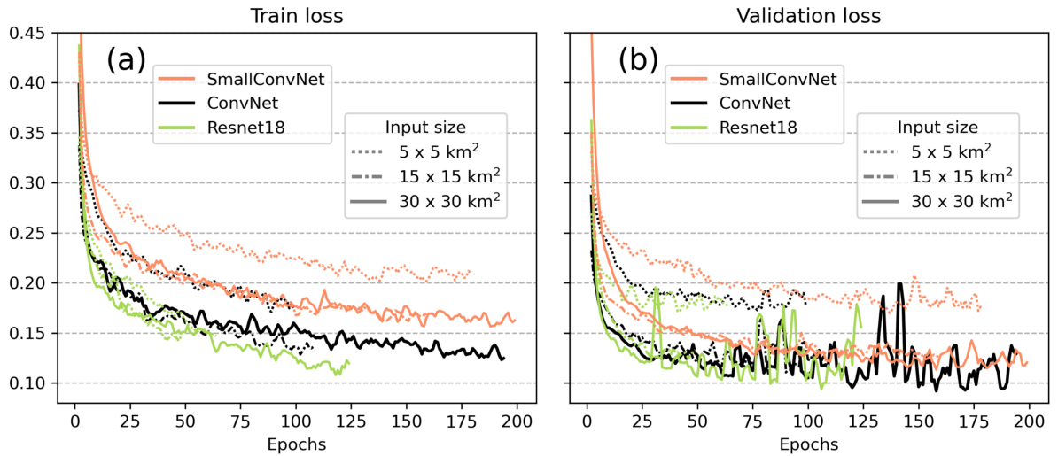
Learning curves for the tuning phase
