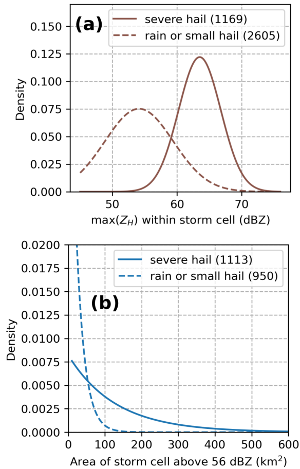
Figure 4. Fitted probability density functions (PDF) for storm cell objects identified above severe hail and rain or small hail reports cases. (a) PDF of the maximum reflectivity ( \max(Z_H) ) within storm cells. (b) PDF of the area for storm cells with the 56 dBZ threshold.
