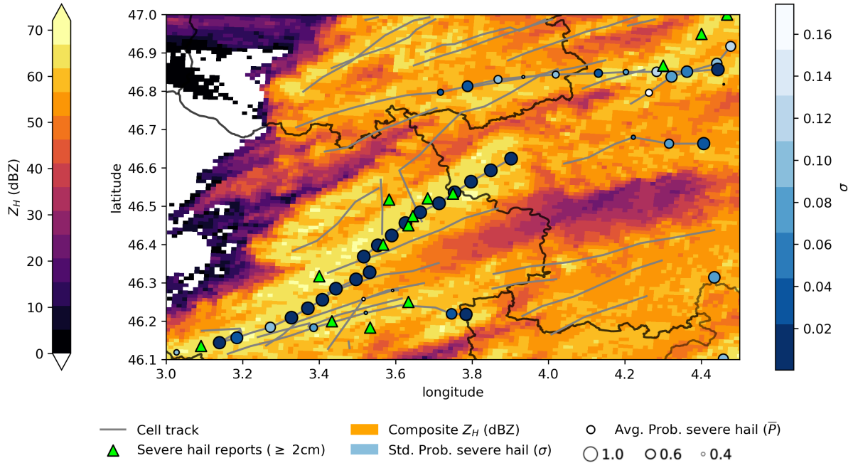
Figure 15. Predictions of ten ConvNet models on the 11th June July 2023 between 17:00 and 19:00 (UTC). The maximum over two hours of the national reflectivity composite is shown in background (orange). Grey lines represent the cell tracks detected with the 'tobac' cell-tracking algorithm (section ??Appendix A). Green triangles represent severe hail reports ( \geq 2 cm) from the ESWD database within the two hours. Circles represent the cell centroids every 5 min. Their average probability of severe hail \bar{P} (circle size) and its affiliated uncertainty \sigma (blue scale) are computed with the predictions of ten ConvNet models applied to 30 \text{ km} \times 30 \text{ km} images around centroids. Cell tracks without circles (pure grey lines) contain cell centroids with \bar{P} < 0.4 .
