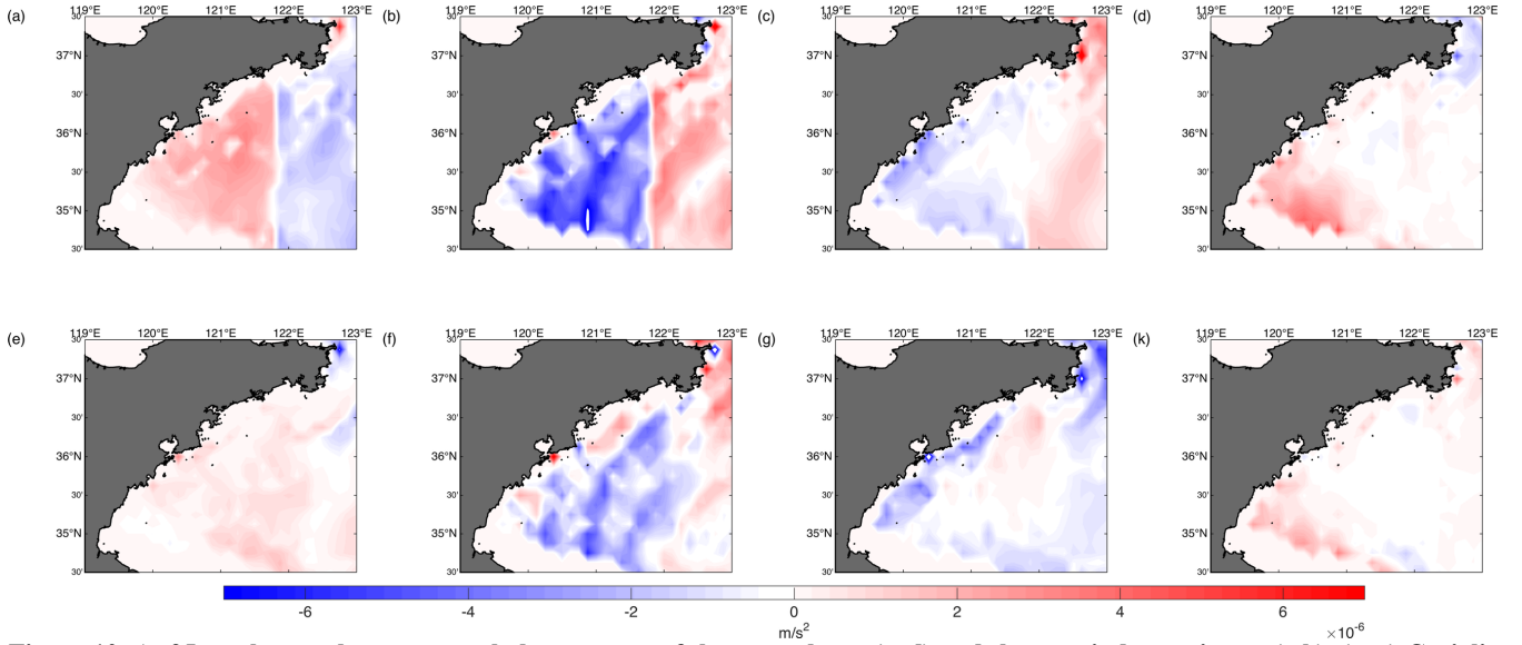
Figure 10. At 25 m, the zonal momentum balance terms of the control run (a–d) and the no-wind experiment (e–h). (a, e) Coriolis 305 force f_v , (b, f) barotropic pressure gradient force -g \frac{\partial \zeta}{\partial x} \vec{l} , (c, g) baroclinic pressure gradient force -\frac{1}{\rho} \frac{\partial}{\partial x} \int_z^\zeta \rho g dz , and (d, h) vertical friction term \frac{\partial}{\partial z} \left( K_m \frac{\partial u}{\partial z} \right) . The results are the monthly means for May. The positive values represent the eastward direction.
