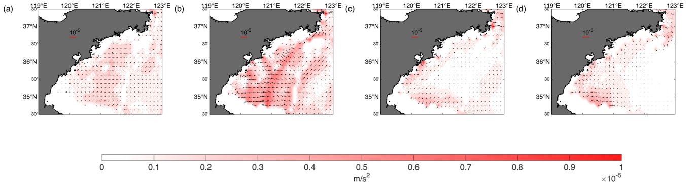
200 Figure 5. Horizontal distributions of momentum terms (monthly mean for May) at depths of (a–d) 25 m: (a) Coriolis force ( f v \vec{i} - f u \vec{j} ), (b) barotropic pressure gradient force ( -g \frac{\partial \zeta}{\partial x} \vec{i} - g \frac{\partial \zeta}{\partial y} \vec{j} ), (c) baroclinic pressure gradient force ( -\frac{1}{\rho} \frac{\partial}{\partial x} \int_z^\zeta \rho g dz \vec{i} - \frac{1}{\rho} \frac{\partial}{\partial y} \int_z^\zeta \rho g dz \vec{j} ), and (d) vertical friction force ( \frac{\partial}{\partial z} \left(K_m \frac{\partial u}{\partial z}\right) \vec{i} + \frac{\partial}{\partial z} \left(K_m \frac{\partial v}{\partial z}\right) \vec{j} ). The color represents the magnitude of the momentum term.
