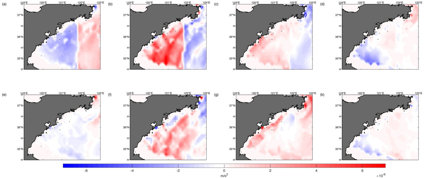
300 Figure 10. At 25 m, the zonal momentum balance terms of the control run (a–d) and the no-wind experiment (e–k). (a, e) Coriolis force f_v , (b, f) barotropic pressure gradient force -g \frac{\partial \zeta}{\partial x} \vec{i} , (c, g) baroclinic pressure gradient force -\frac{1}{\rho} \frac{\partial}{\partial x} \int_z^\zeta \rho g dz , and (d, k) vertical friction term \frac{\partial}{\partial z} \left( K_m \frac{\partial u}{\partial z} \right) . The results are the monthly means for May. The positive values represent the eastward direction.
