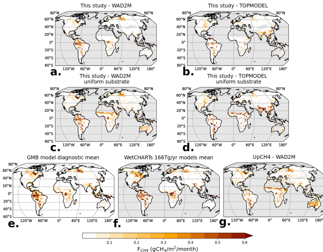
Figure 6. SatWetCH4 modeled mean methane emissions: a. using WAD2M and b. TOPMODEL wetland surfaces; and with a uniform substrate (i.e., C_{substrate} = 1 ) c. using WAD2M and d. using TOPMODEL. Emissions obtained by e. the mean of GMB diagnostic models, f. the mean of WetCHARTs ensemble, and g. UpCH4 upscaling.
