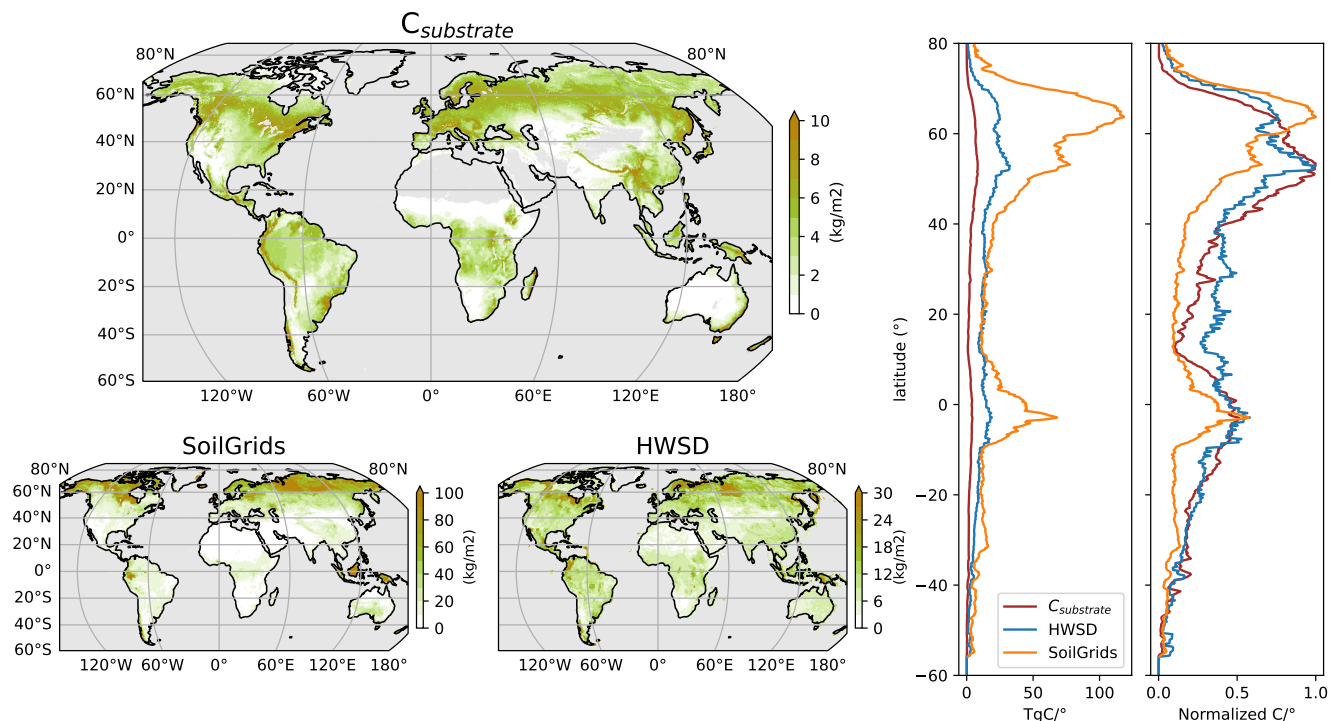
Figure 5. Derived C_{\text{substrate}} product (top left) showing the 2003-2020 mean, alongside two SOC databases (bottom left and middle) for the 0-100 cm layer: HWSD (Wieder, 2014) and SoilGrids (Hengl et al., 2017). The corresponding latitudinal and normalized latitudinal profiles are displayed (right panels). Normalization is achieved by dividing by the latitudinal maximum for each product.
