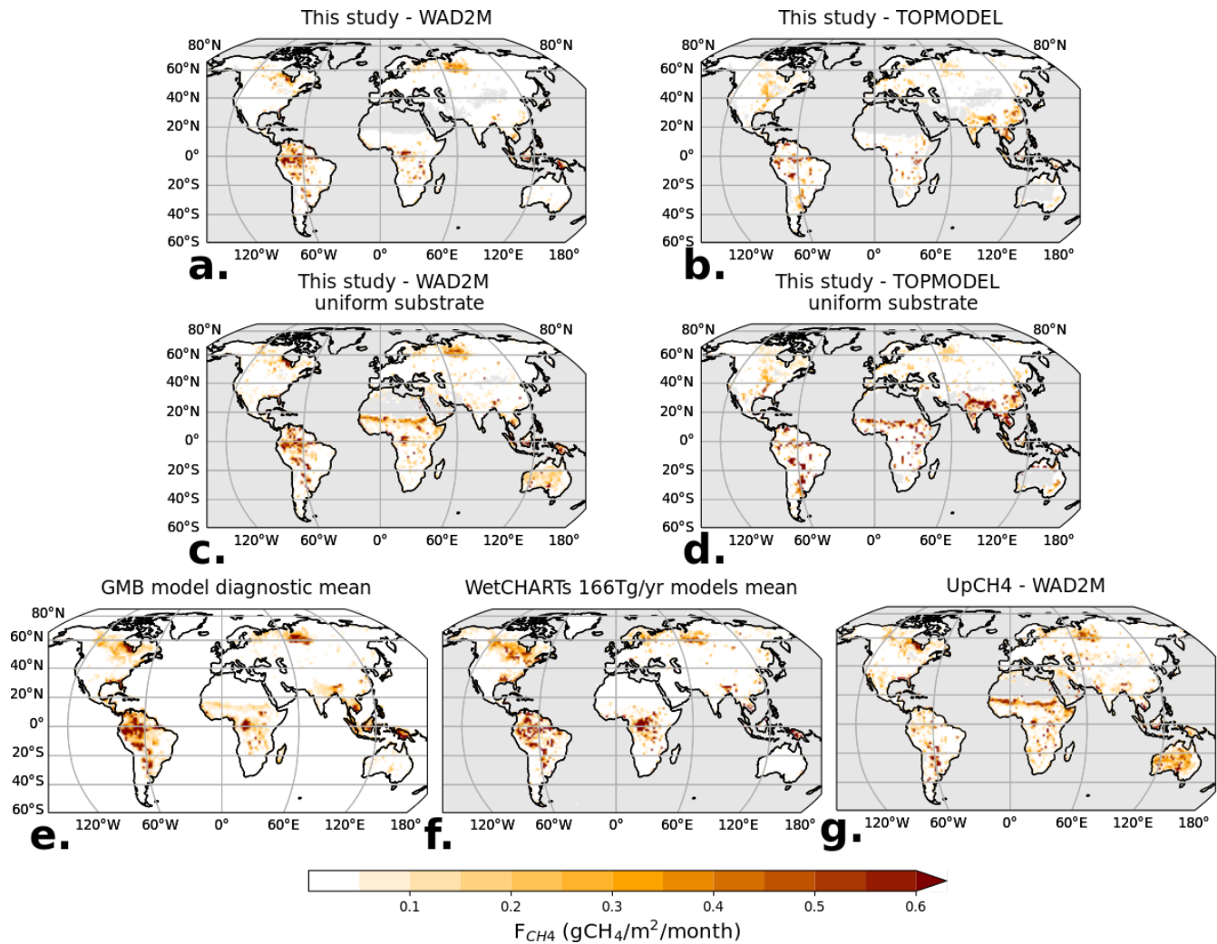
Figure 6. SatWetCH4 modeled mean methane emission using emissions: a. using WAD2M and b. TOPMODEL wetland surfaces: SatWetCH4 emissions obtained using: and with a uniform substrate —(i.e., C_{substrate} = 1 — and ) c. using WAD2M or d. using TOPMODEL . Emissions obtained by e. the mean of GMB diagnostic models , f. the mean of WetCHARTs ensemble , and g. UpCH4 upscaling .
